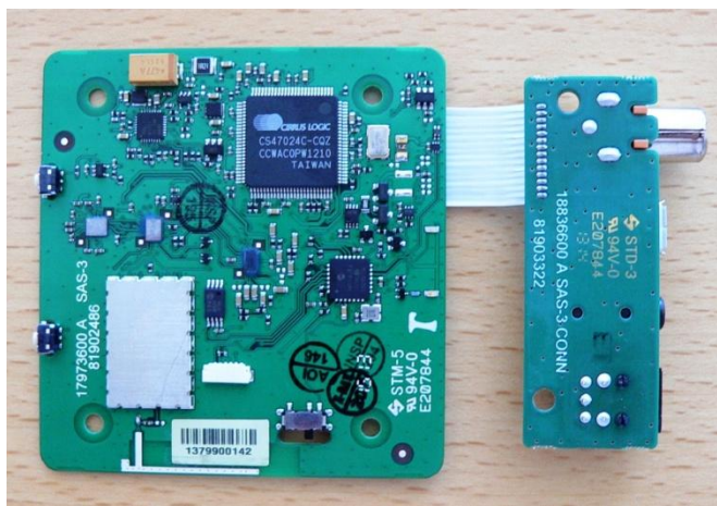
Front side (with shielding cover)
