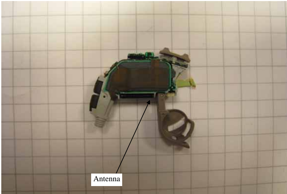
Photo 4.3.1 Test setup regarding Antenna requirement
