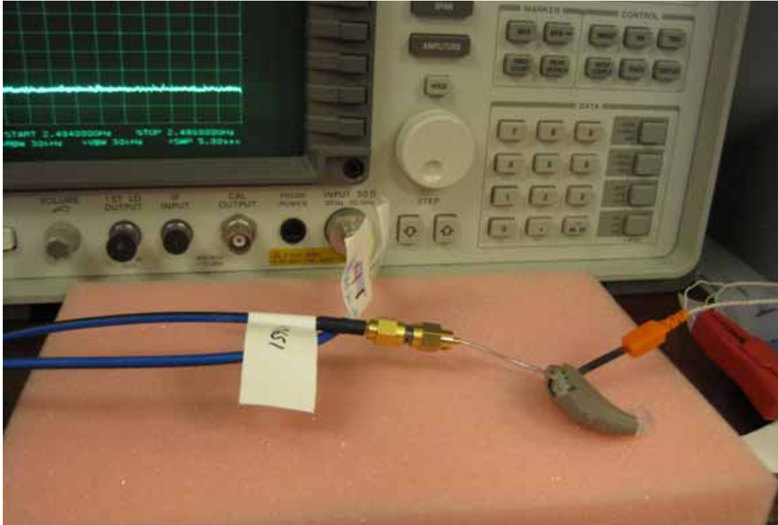
Photo 4.8.1 Test setup regarding measurement of occupied bandwidth, IC.
