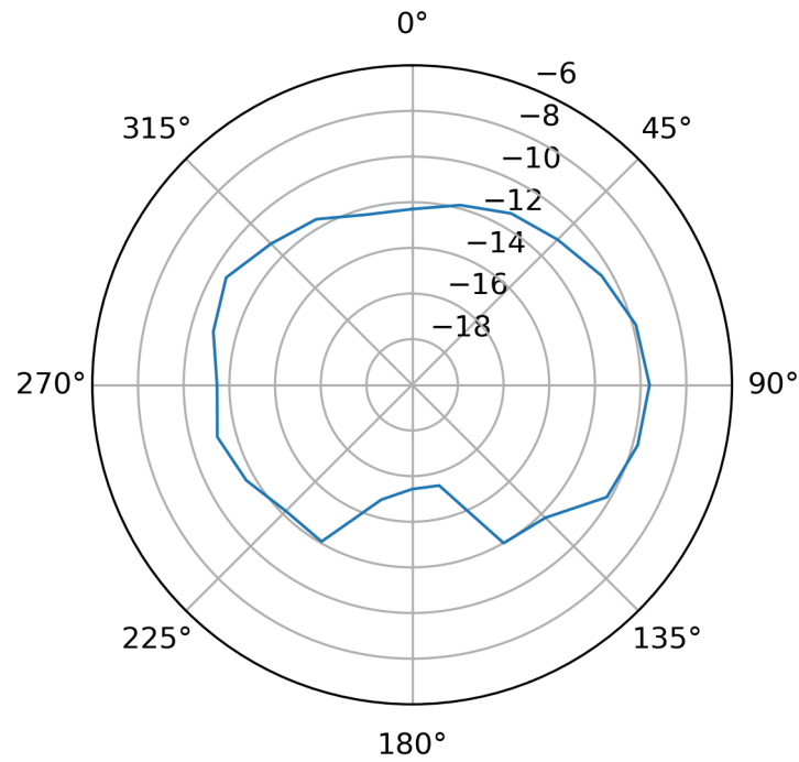
Total EIRP (dBm), Phi=0 (XZ), f=2480
