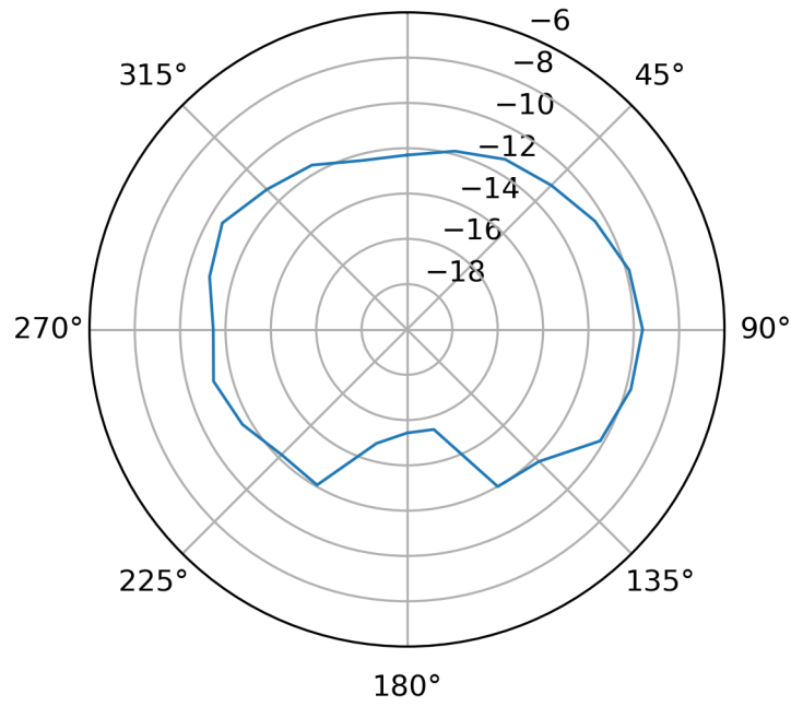
Total EIRP (dBm), Phi=0 (XZ), f=2480 0°
