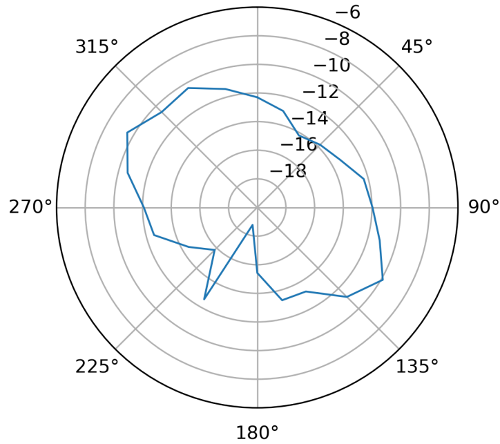
Total EIRP (dBm), Phi=90 (YZ), f=2480 0°
