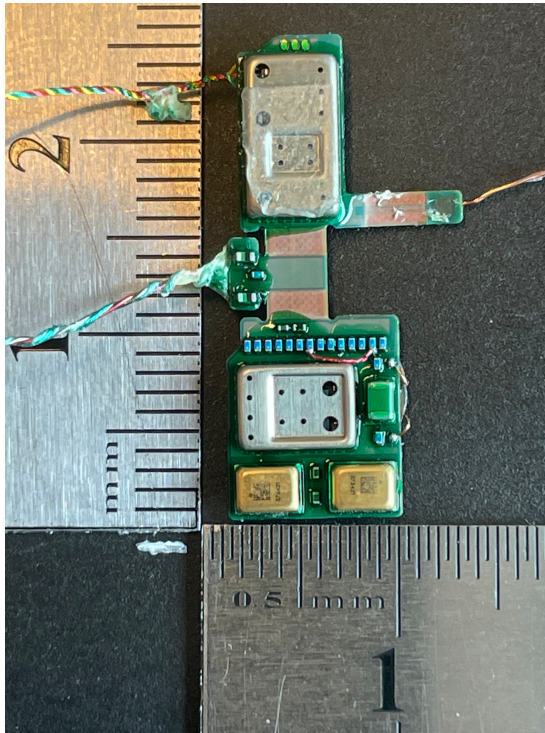
PCBA TOP SIDE VIEW
