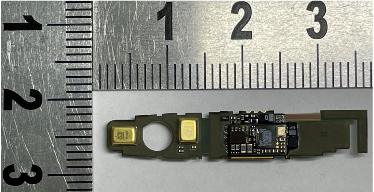
PCB TOP SIDE VIEW
