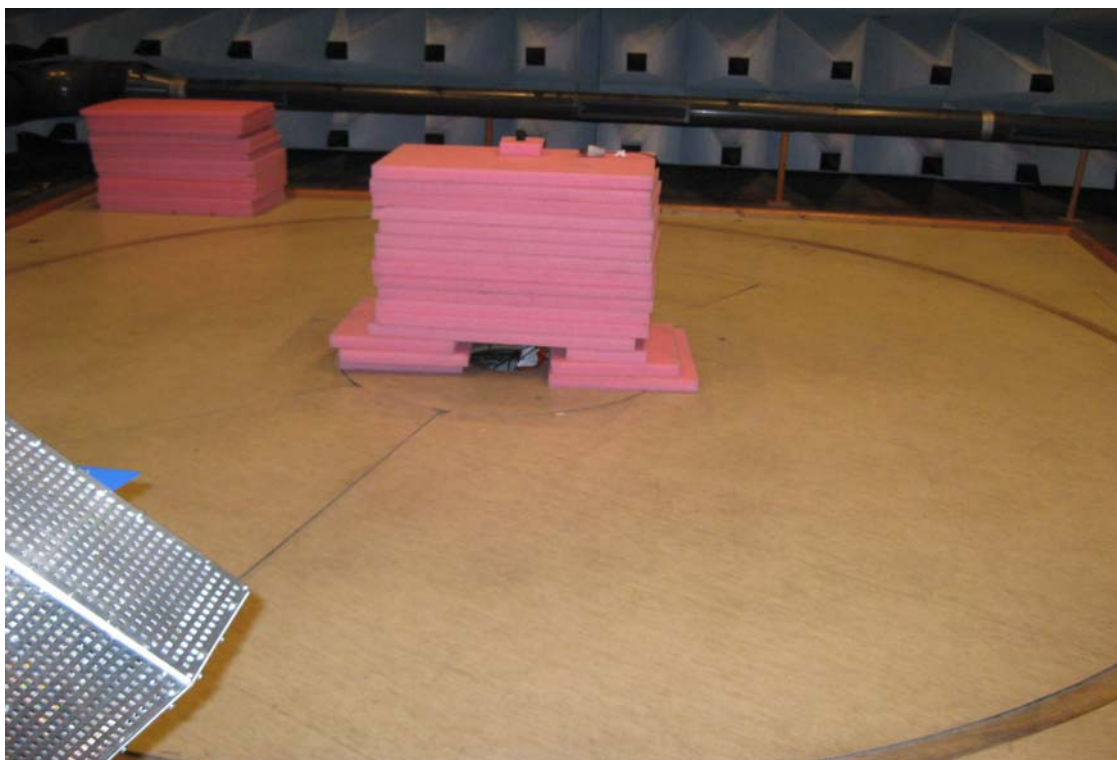
Photo 4.7.1 Test setup regarding measurement of radiated emission, 1 GHz to 25 GHz.
