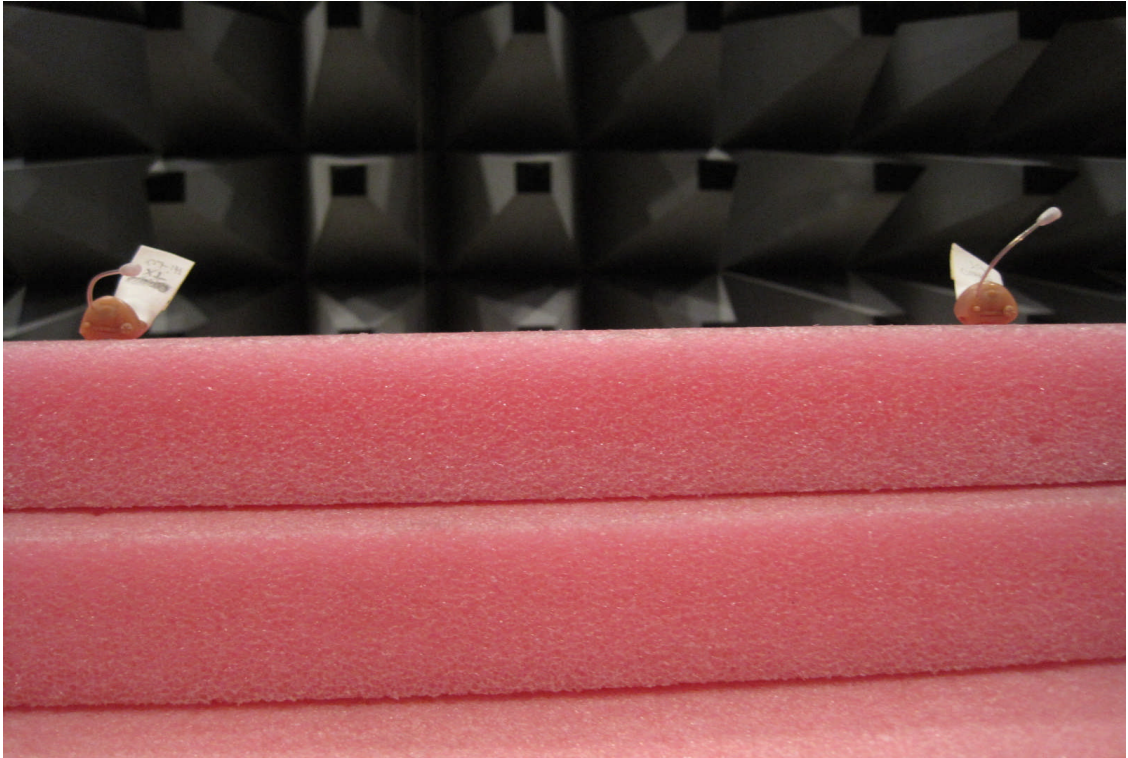
Photo 4.9.3 Test setup regarding measurement of radiated emission, Rx, IC, 1 GHz to 25 GHz.
