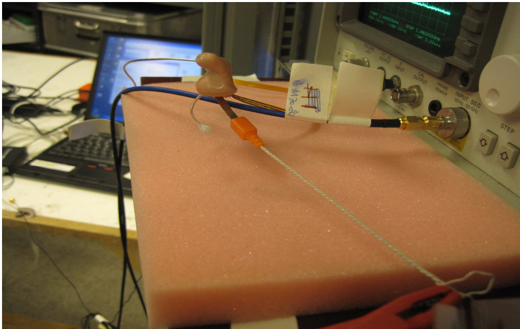
Photo 4.8.1 Test setup regarding measurement of occupied bandwidth, IC.
