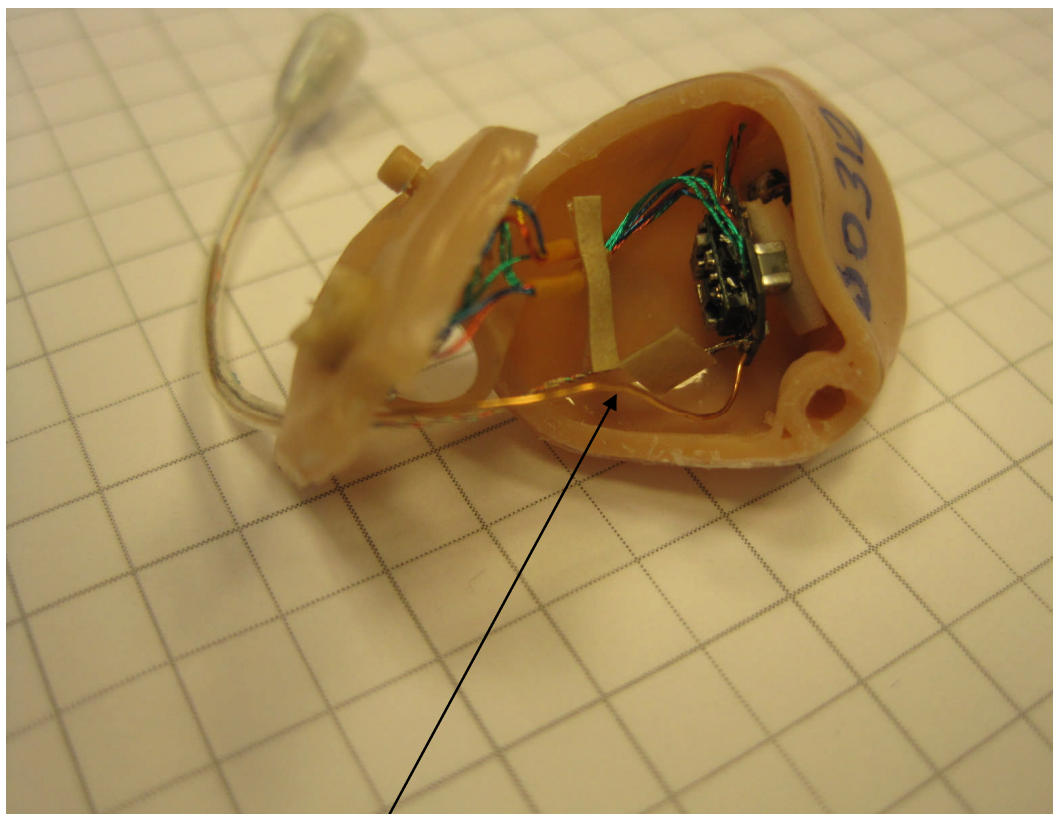
Photo 4.3.1 Test setup regarding Antenna requirement.
