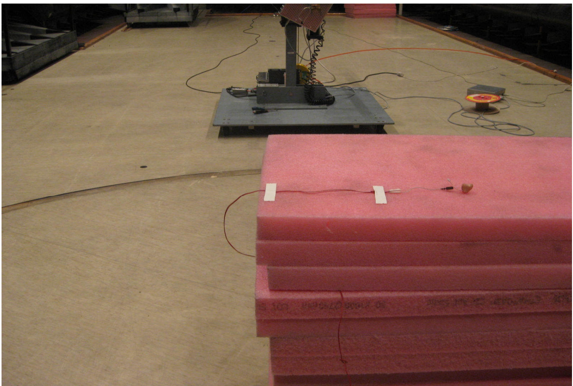
Photo 1.1.7 Test setup regarding measurement of radiated emission, 1 GHz to 25 GHz.
