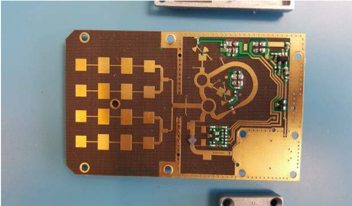
Circuit board 1.1.4
