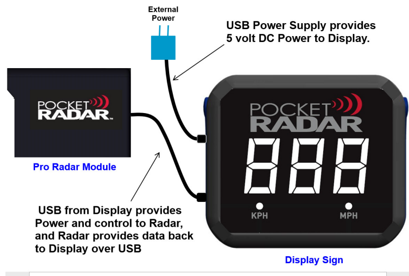
Figure 3.8-1: Setup diagram
