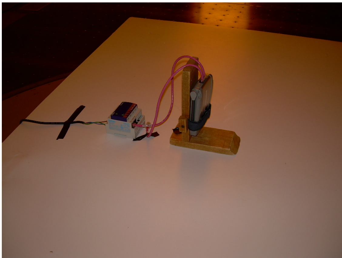
View of Test Setup - Vertical with Antenna Vertical Beside PCB
