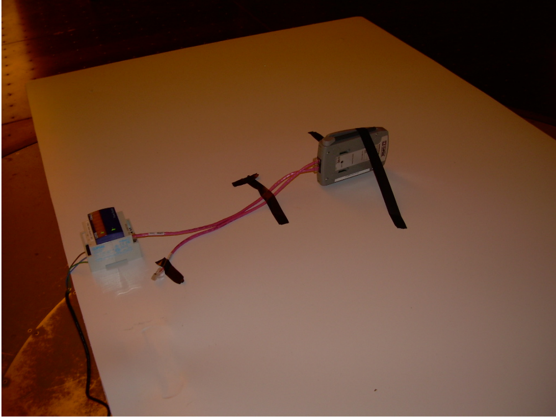
View of Test Setup - On Edge with Antenna Beside PCB
