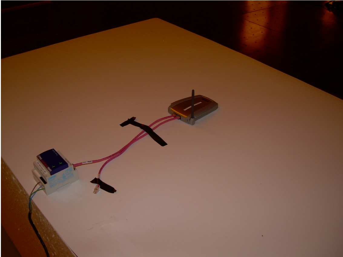
View of Test Setup - Horizontal with Antenna Vertical
