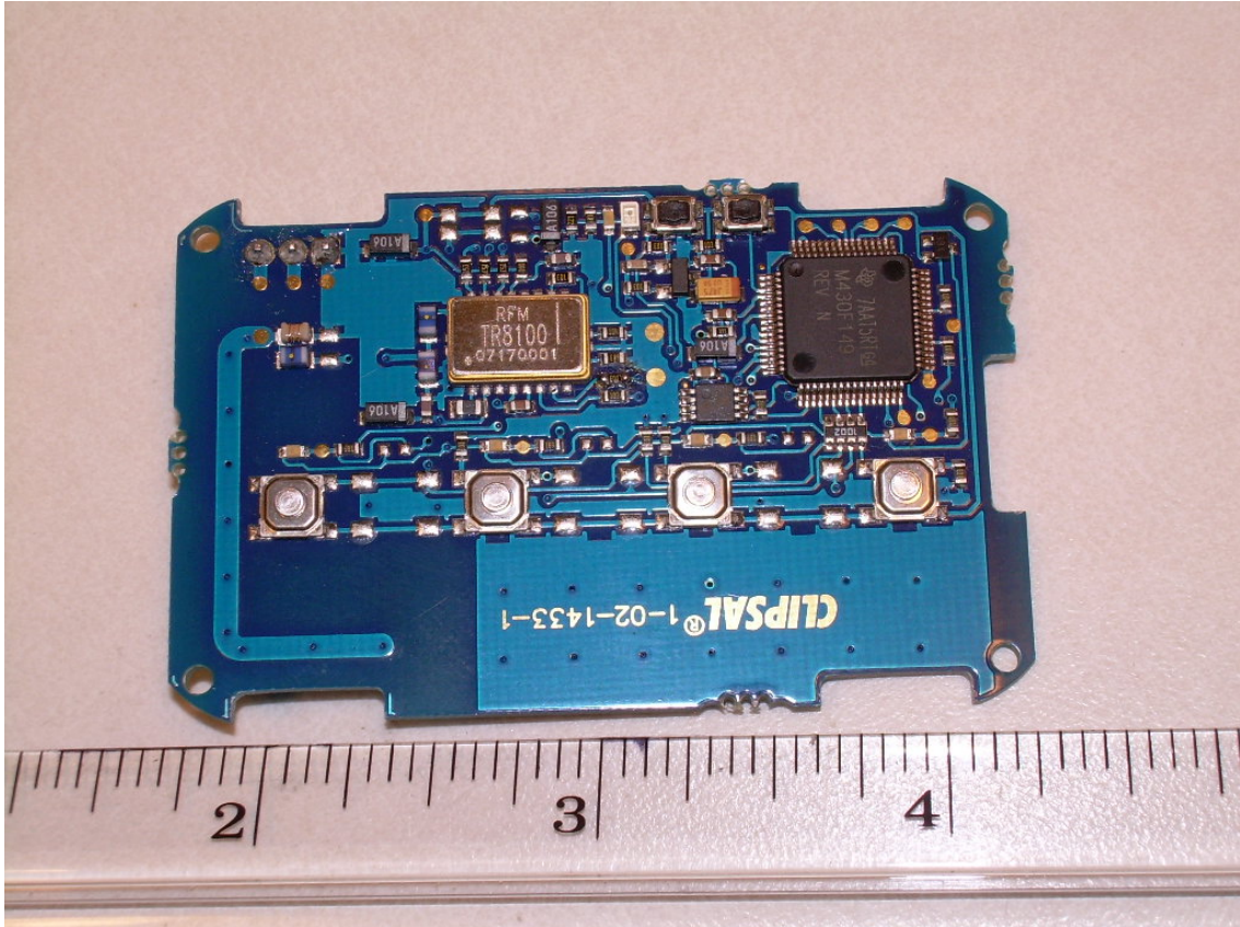
Component Side of the EUT
