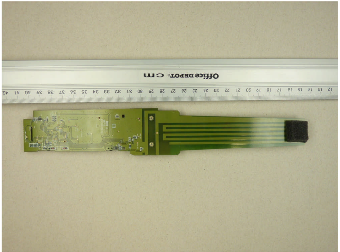
112488eut6.jpg: PCB, rear-view
