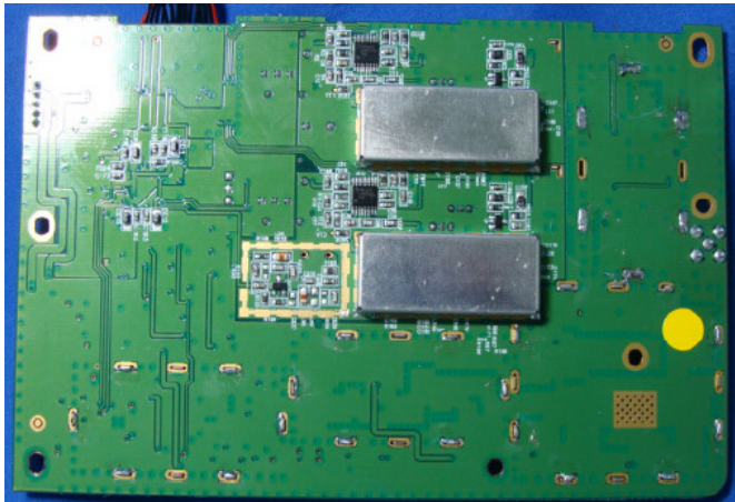
Figure 9: Bottom View of RF Module
