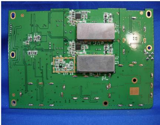
Figure 6: Bottom View of RF Module
