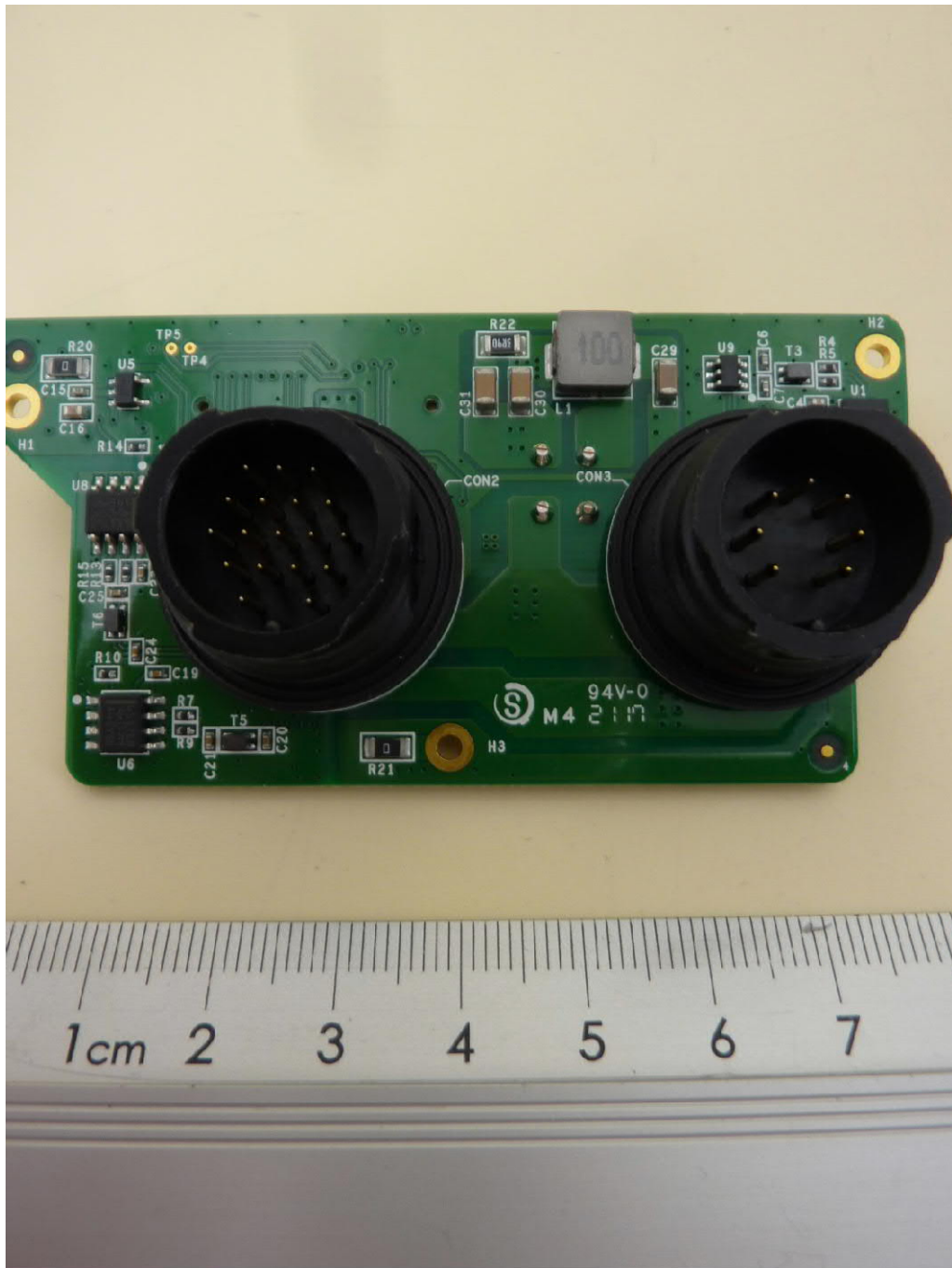
Connector PCB, top view
