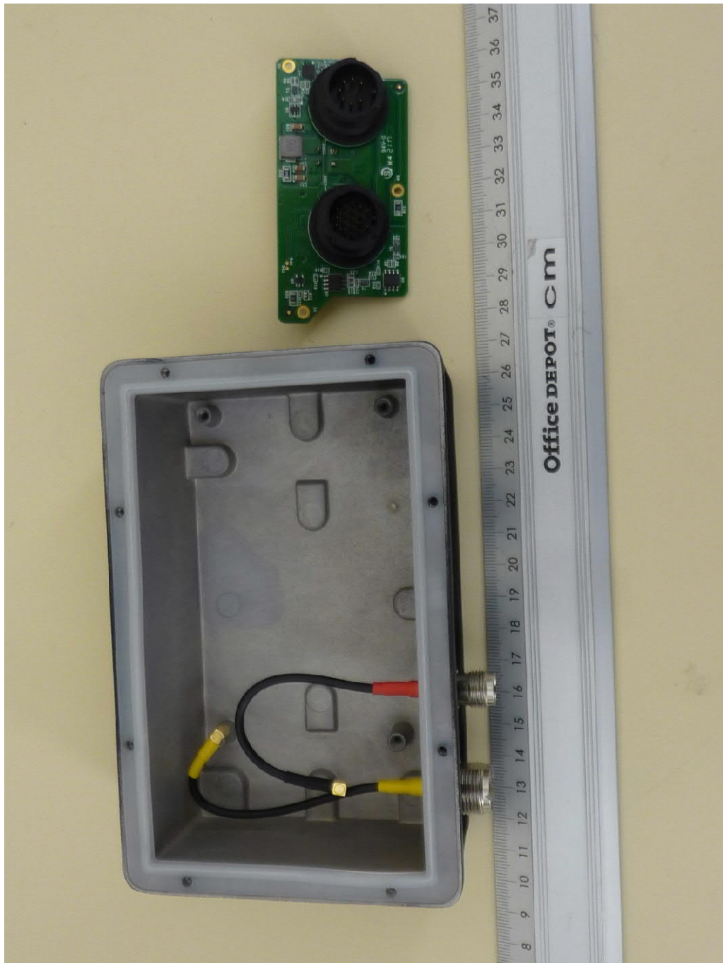
Internal view 2, connector PCB removed
