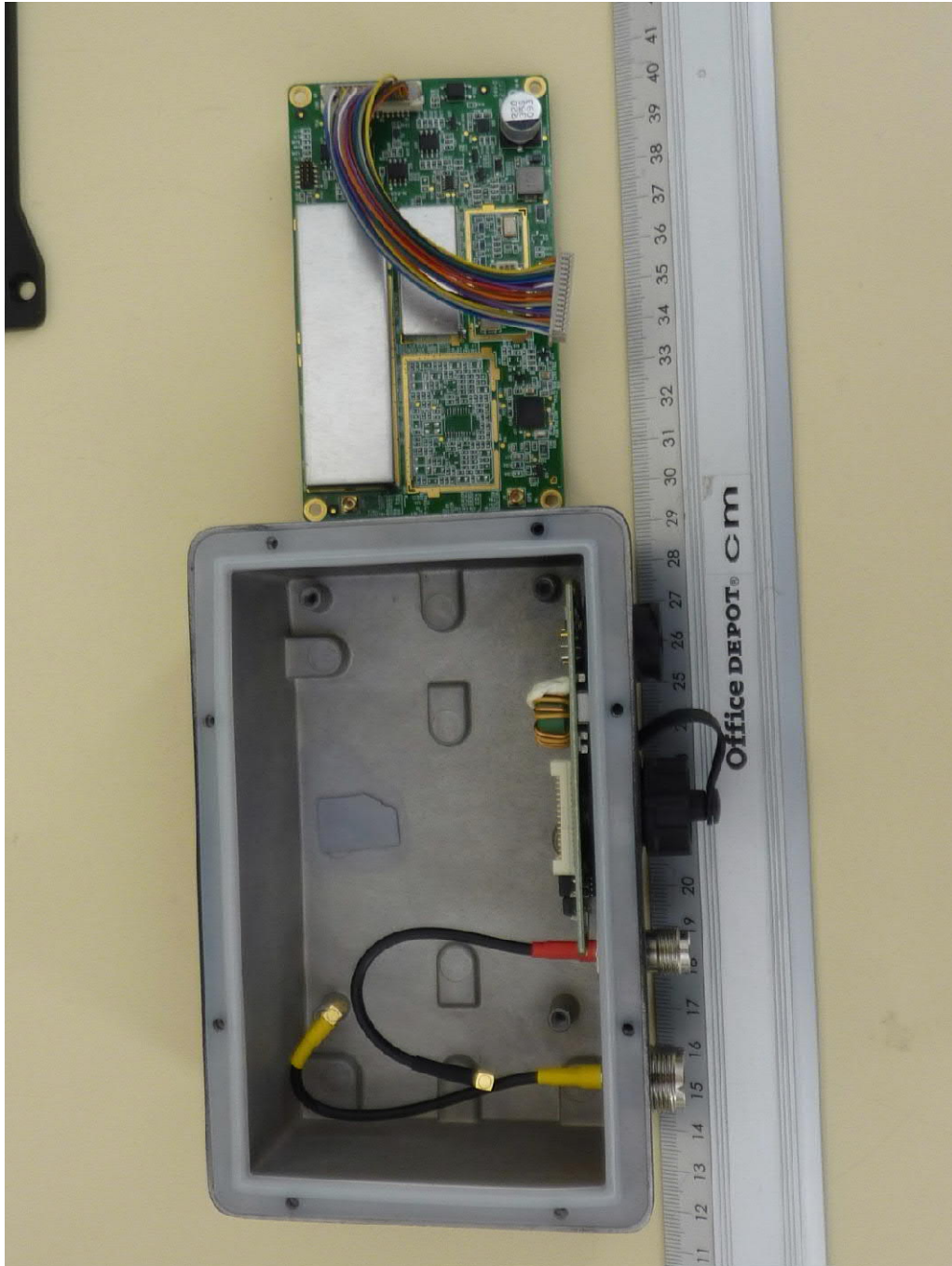
Internal view 2, main PCB removed
