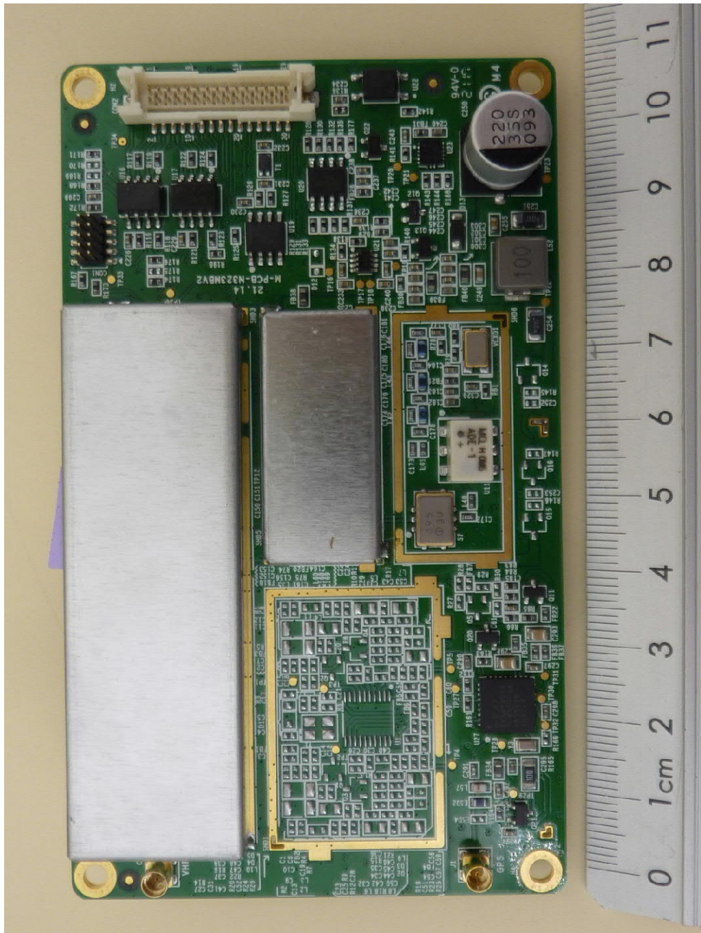
Main PCB, top view
