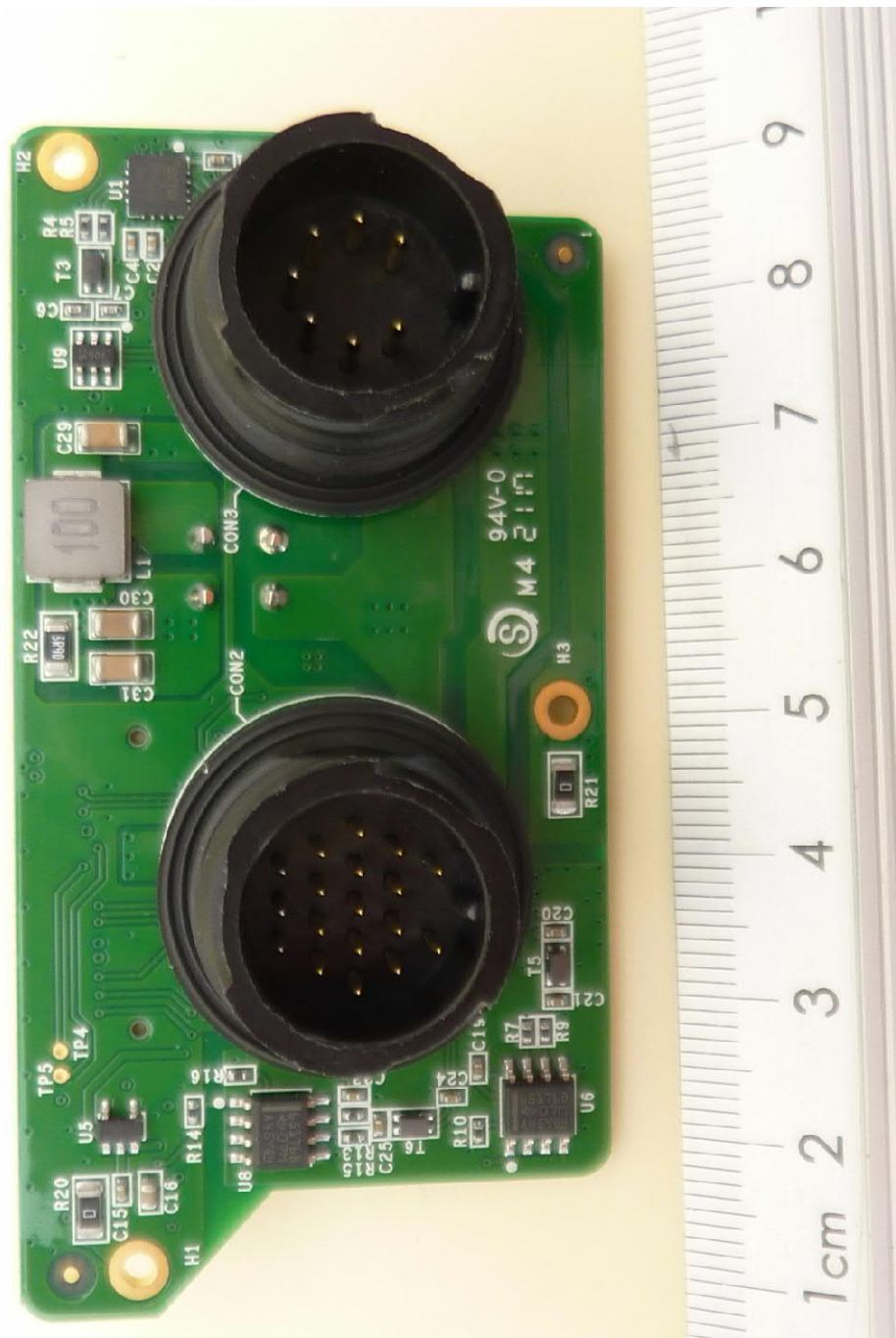
Connector PCB, top view
