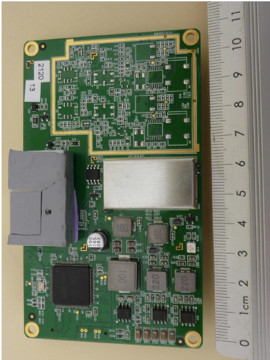
Main PCB, bottom view
