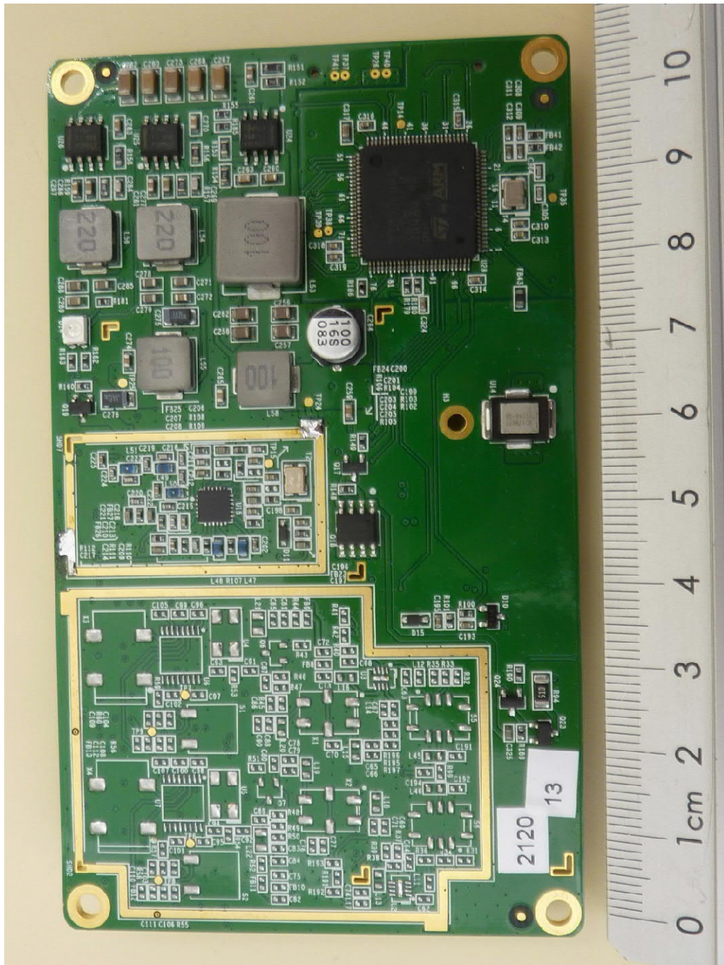
Main PCB, bottom view, shieldings removed
