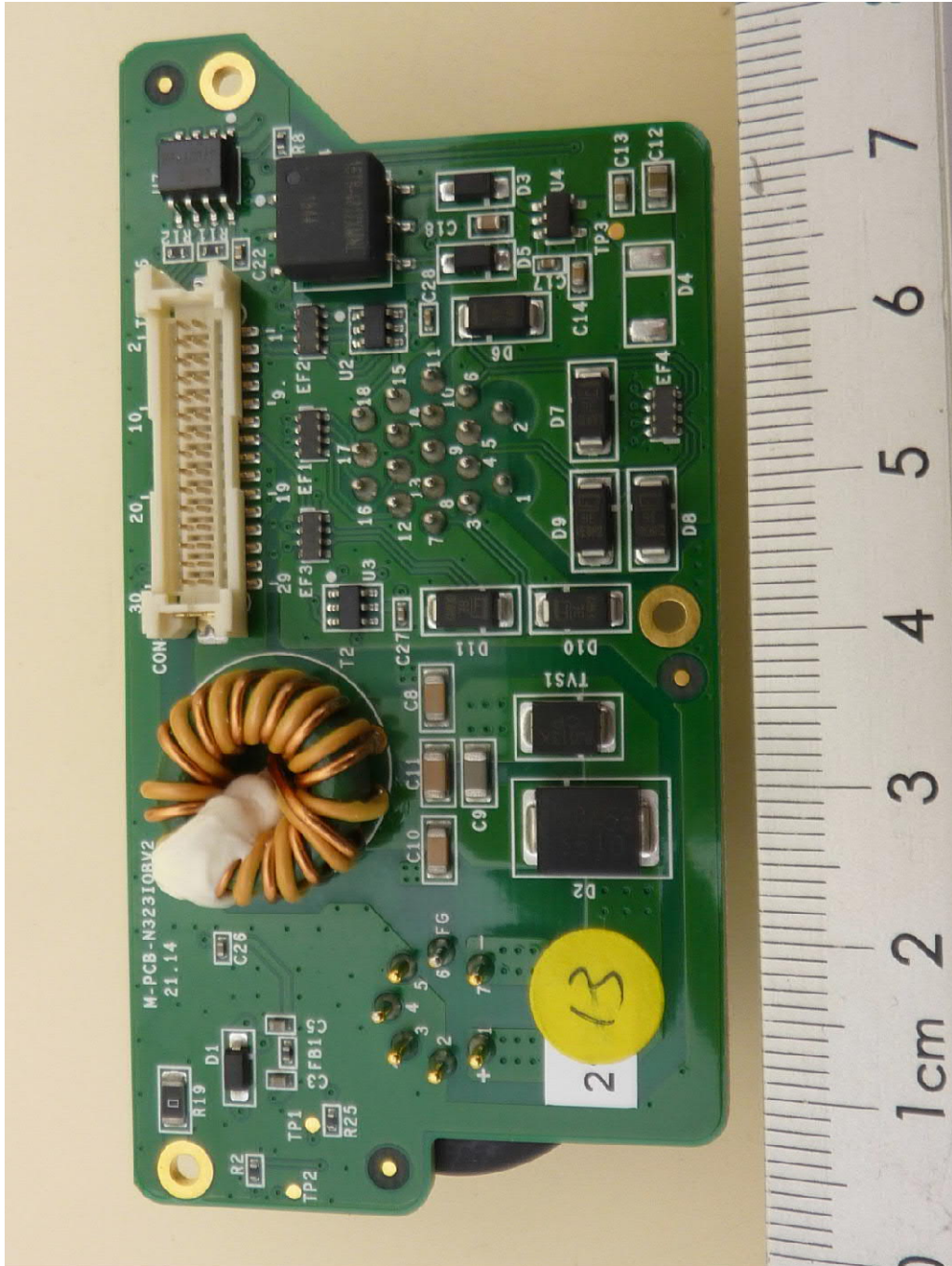
Connector PCB, bottom view
