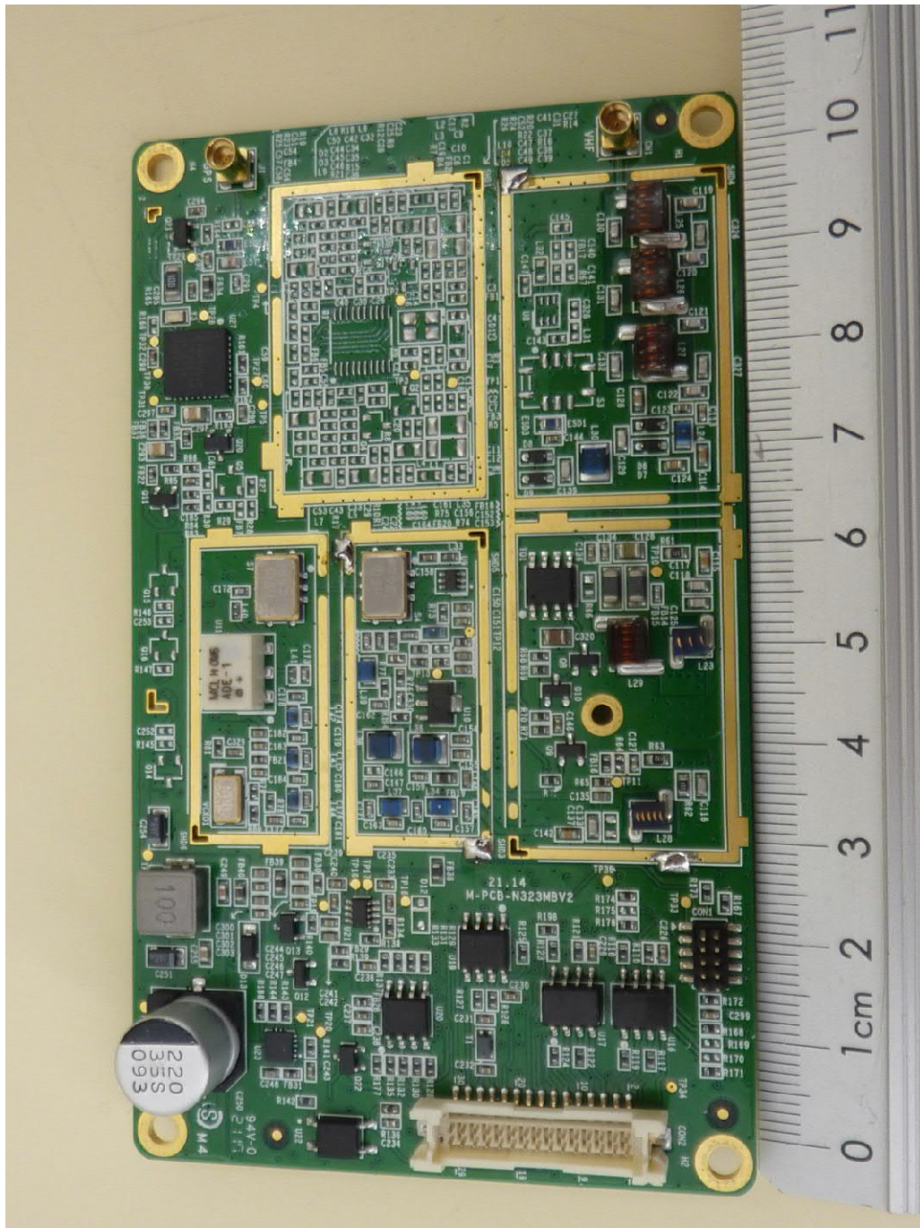
Main PCB, top view, shieldings removed
