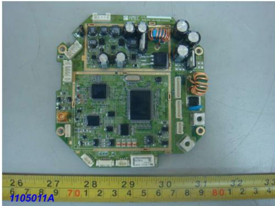
(7) Mando-303 internal photo #2
