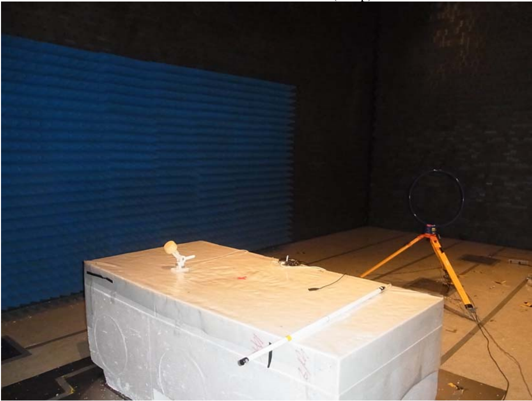
Front View of Radiated Test (Loop)
