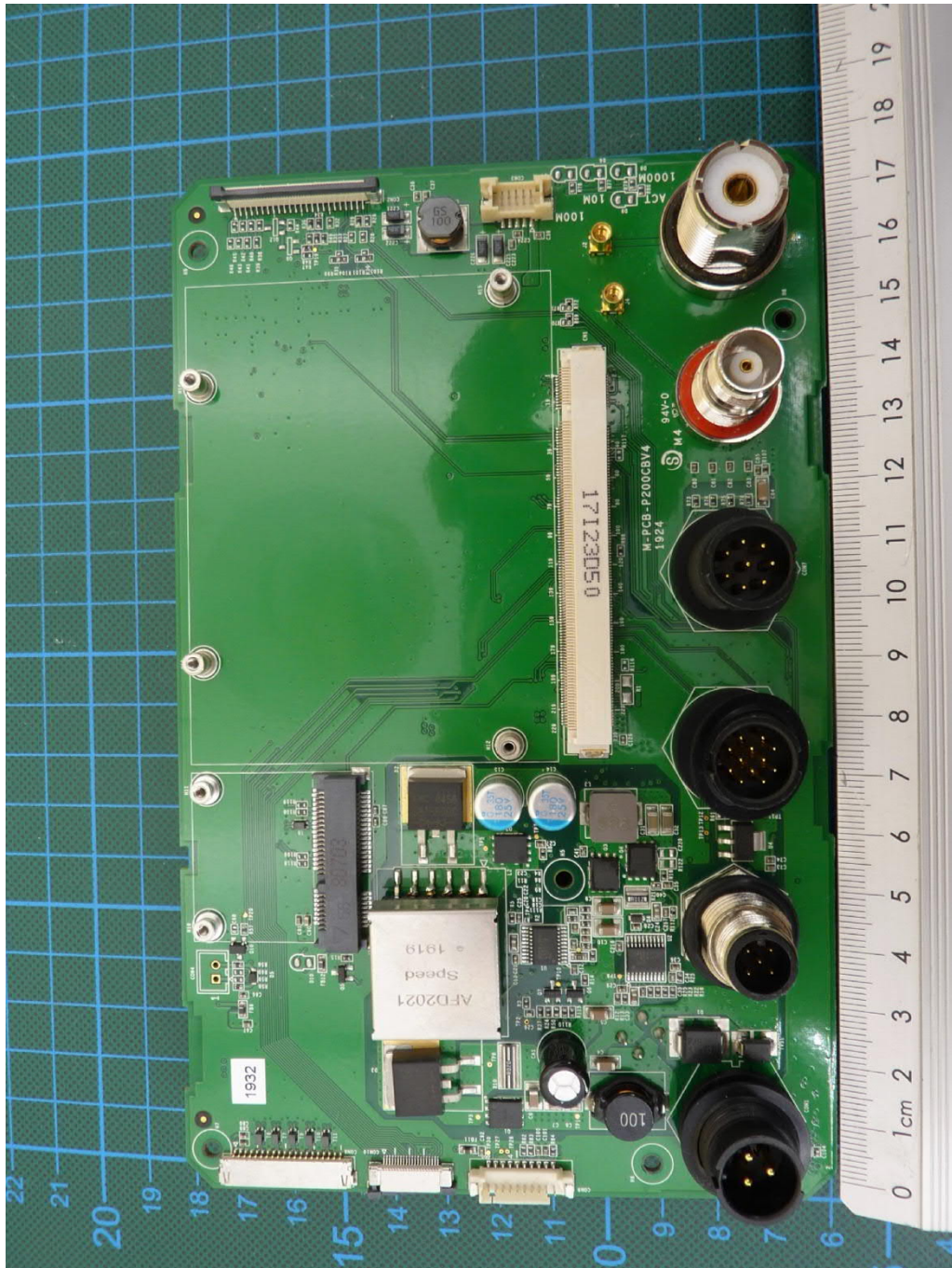
P200-SO, PCB3, top view
