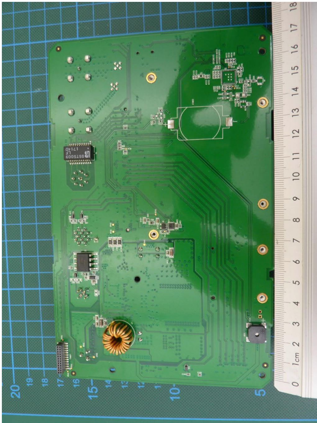
P200-SO, PCB3, bottom view
