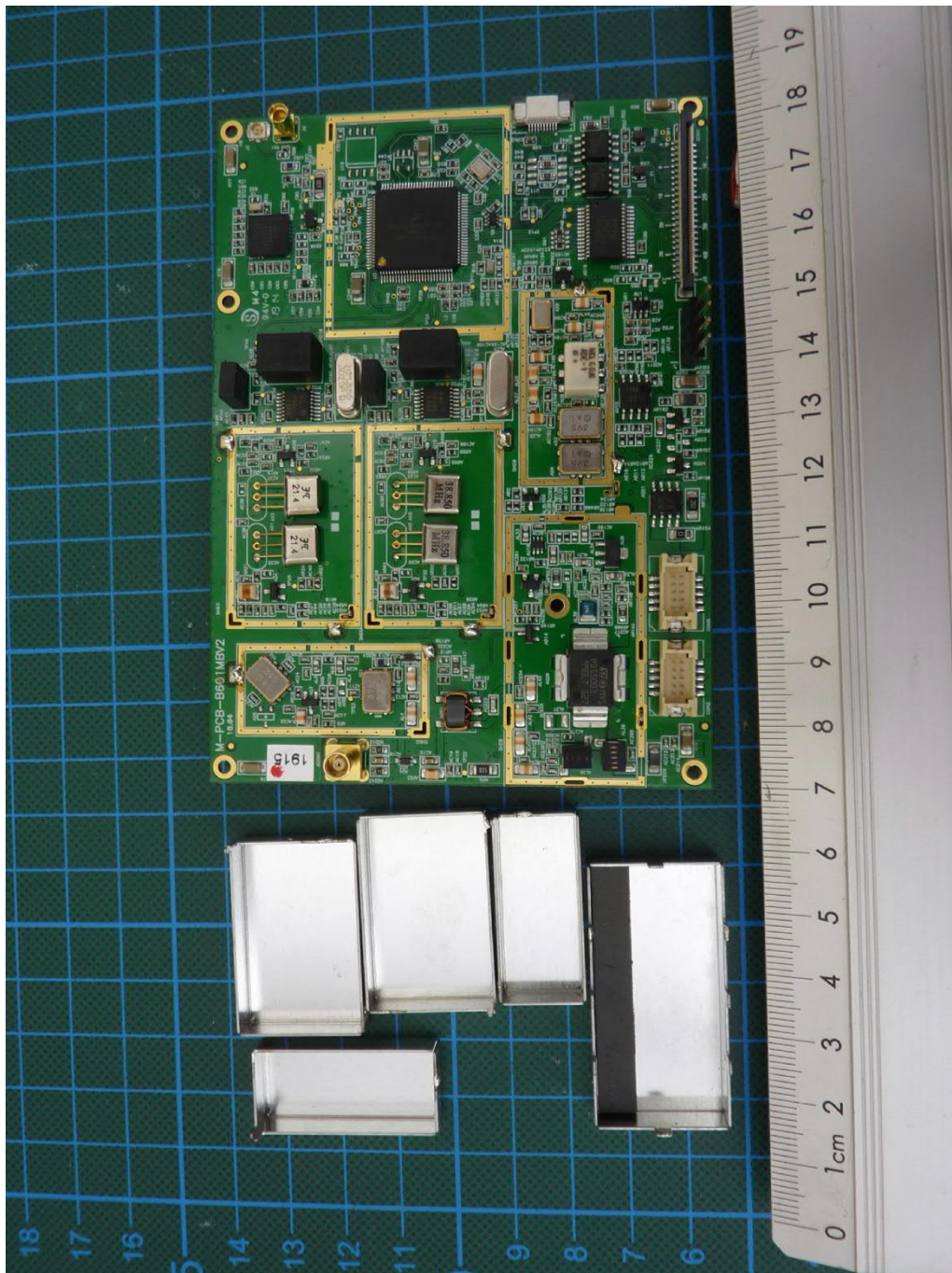
P200-SO, PCB4, top view (shielding removed)
