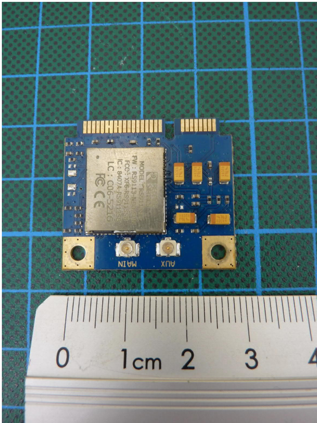
P200-SO, PCB2, top view
