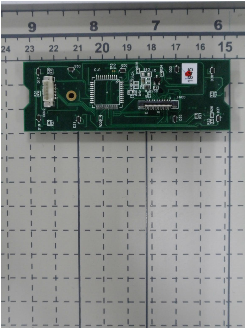
P200-SO, PCB5, bottom view Photograph supplied by the applicant
