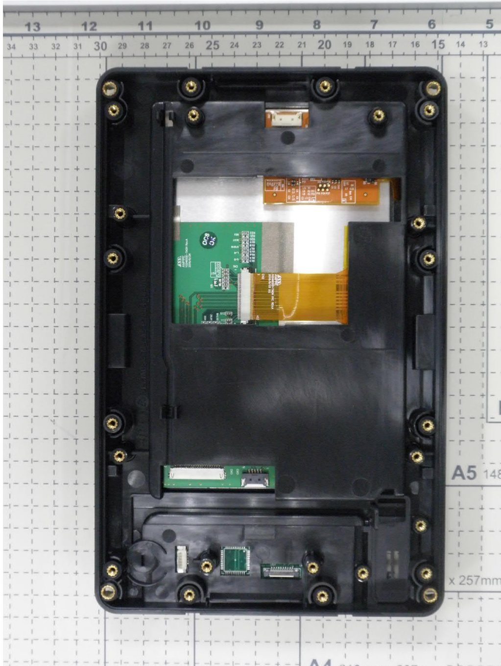
P200-SO, internal view 5 (cables removed)
