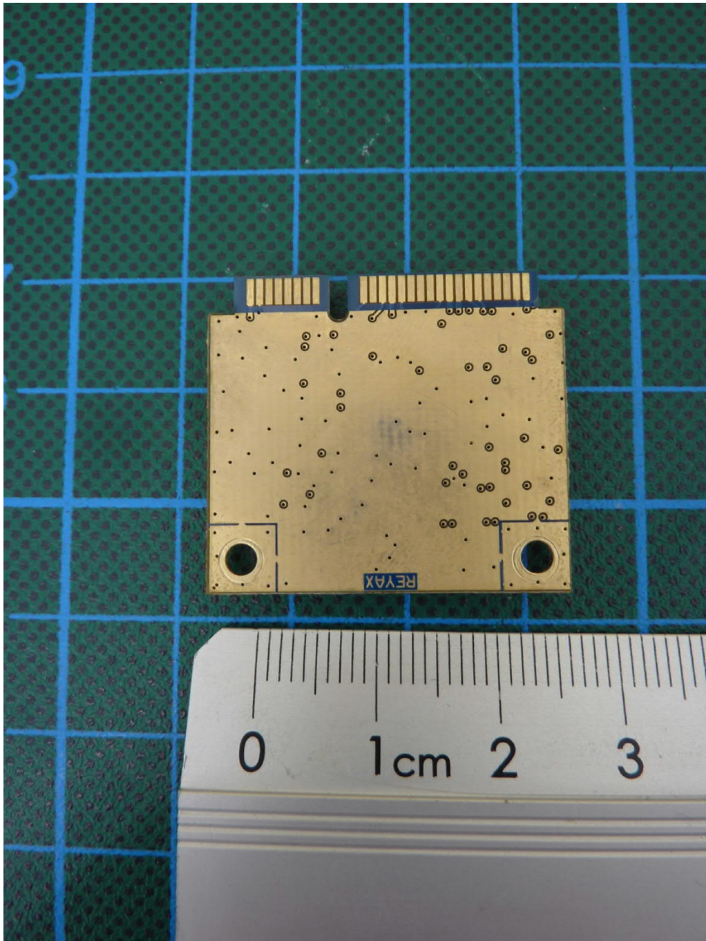
P200-SO, PCB2, bottom view
