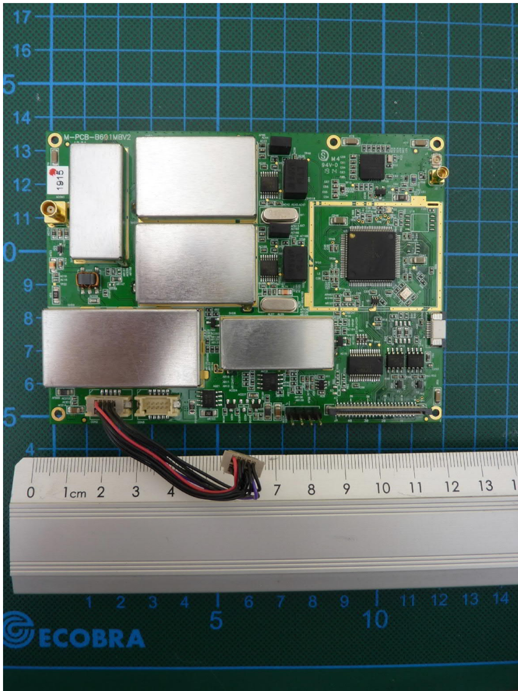
P200-SO, PCB4, top view
