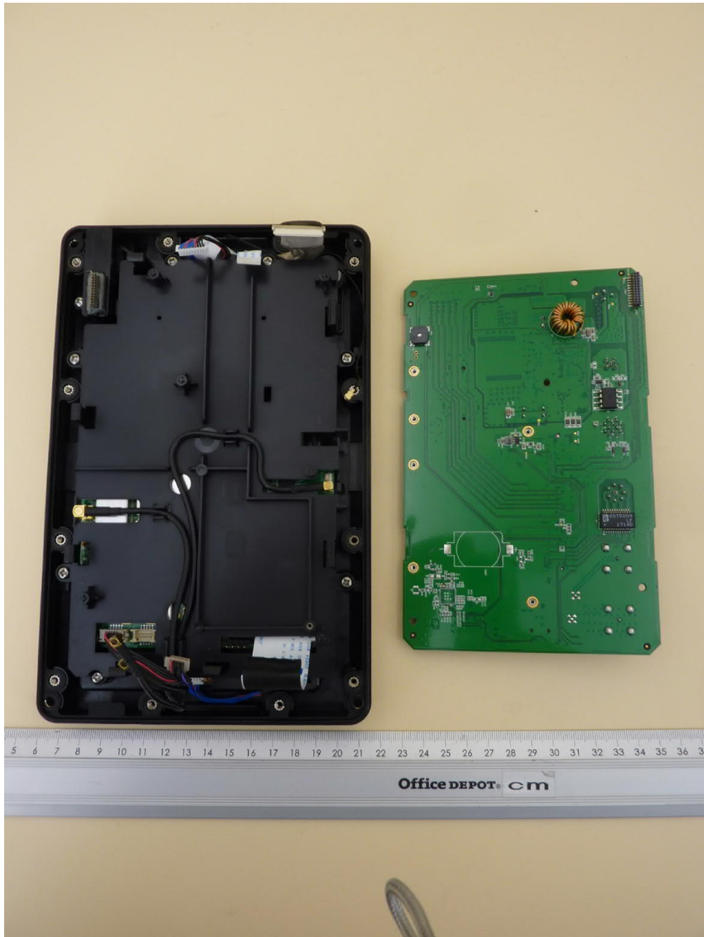
P200-SO, internal view 3 (PCB 3 removed)
