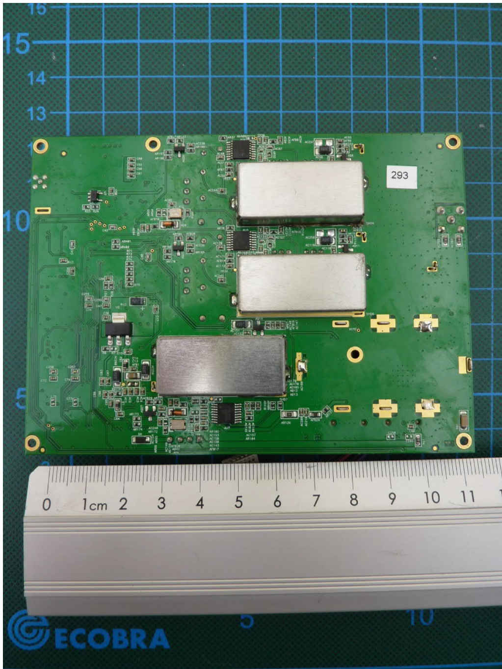
P200-SO, PCB4, bottom view
