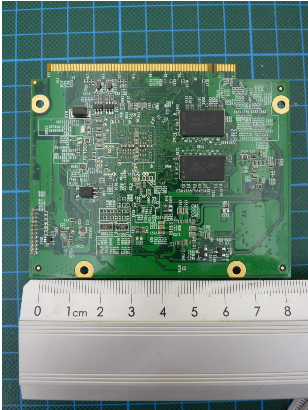
P200-SO, PCB1, bottom view
