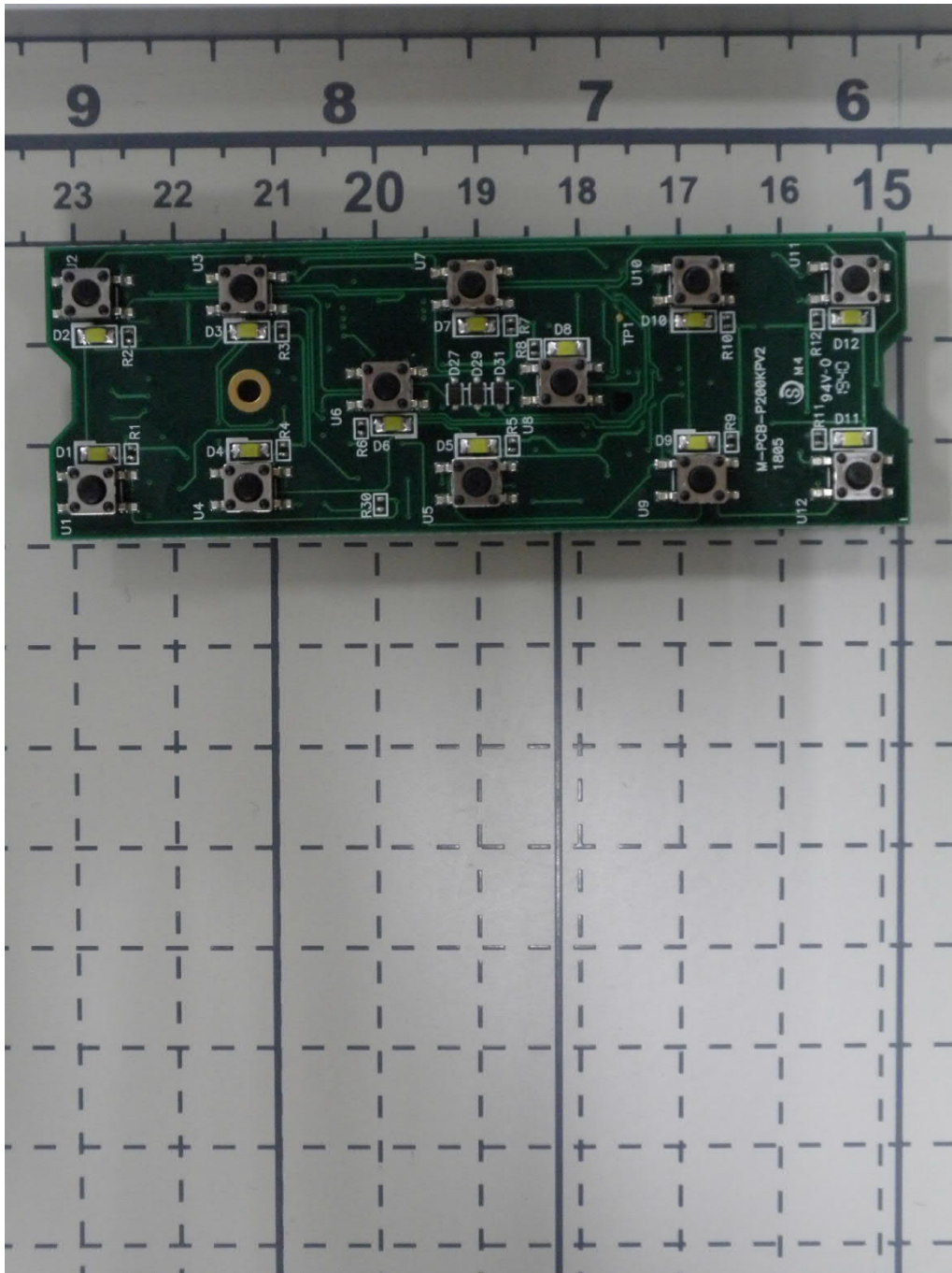
P200-CS, PCB5, top view Photograph supplied by the applicant
