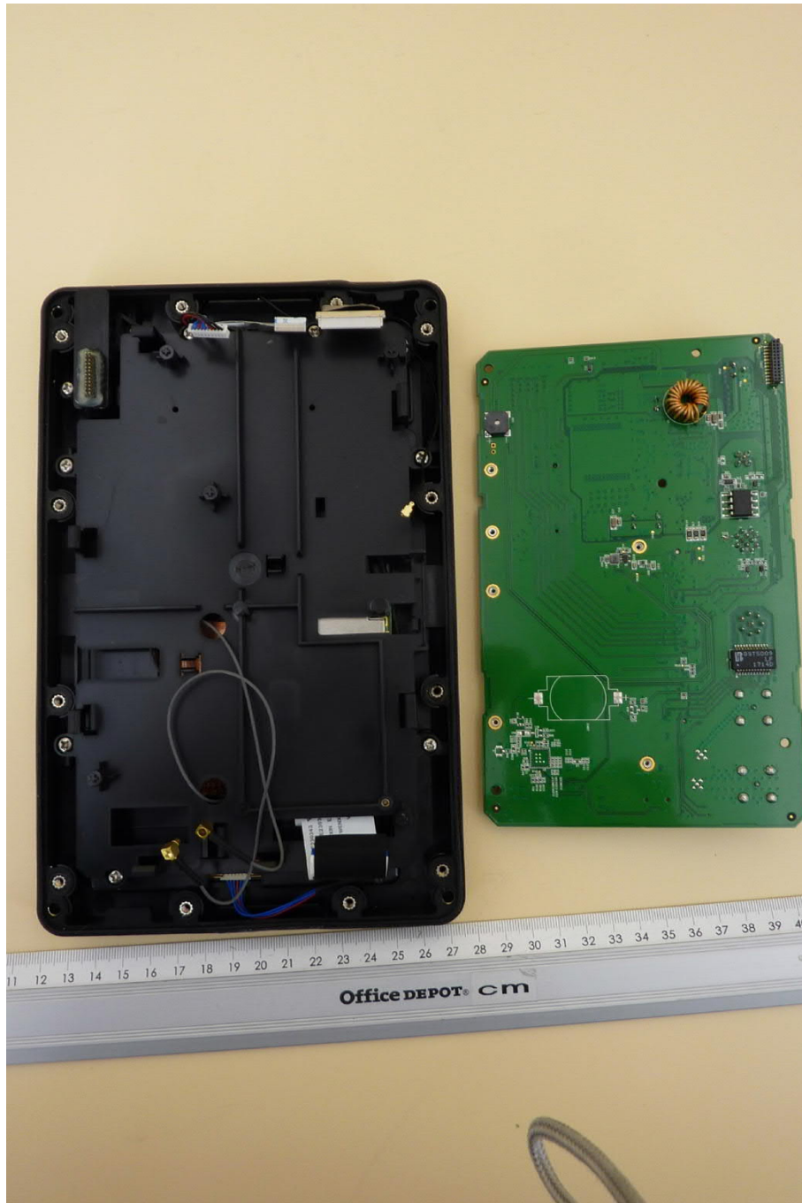
P200-CS, internal view 4 (PCB 3 removed)
