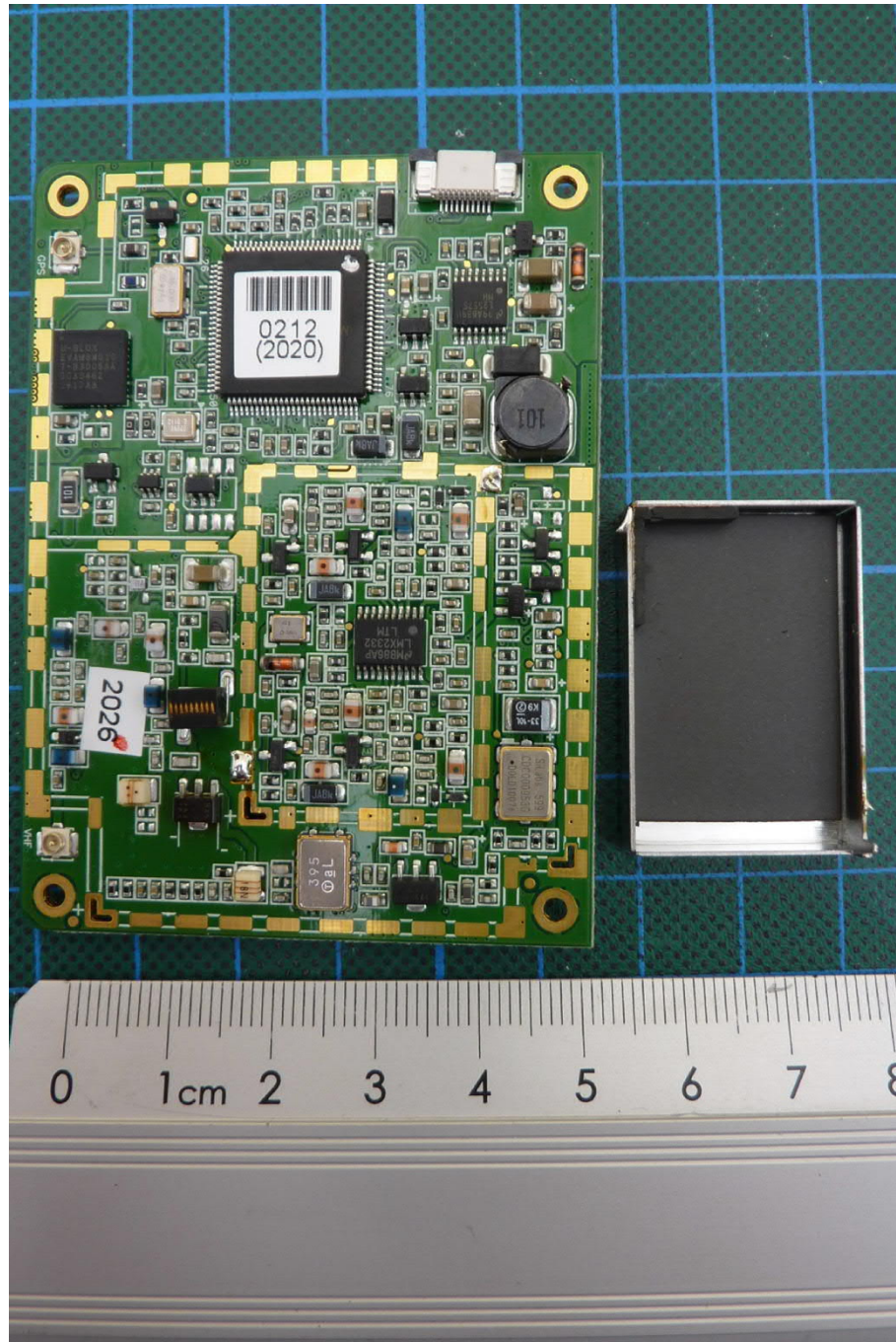
P200-CS, PCB4, bottom view (shielding removed)
