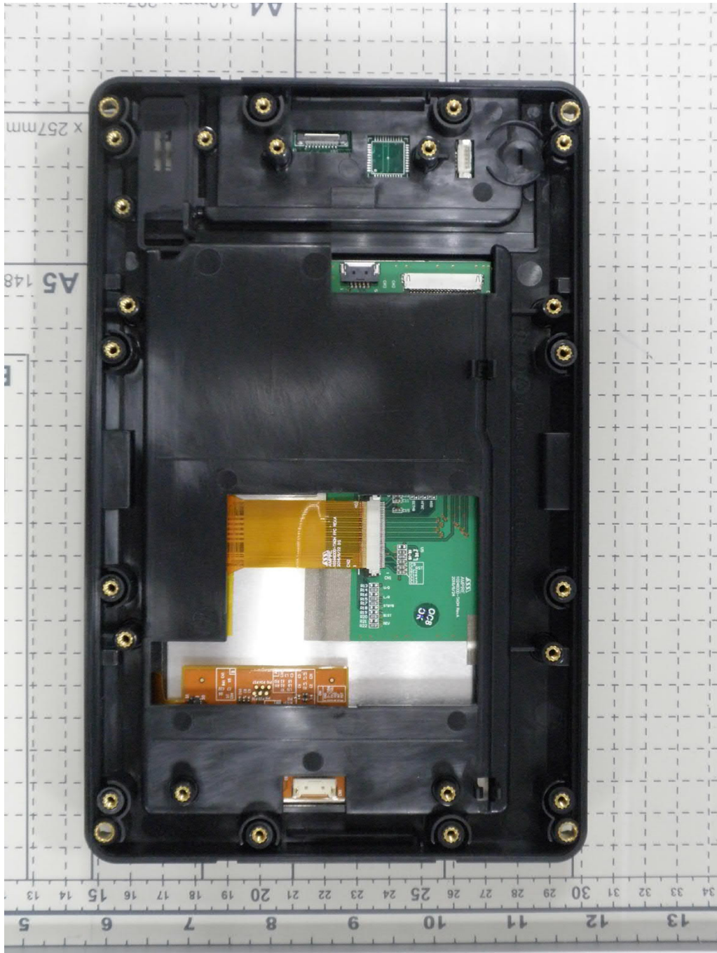
P200-CS, internal view 6 (cables removed)
