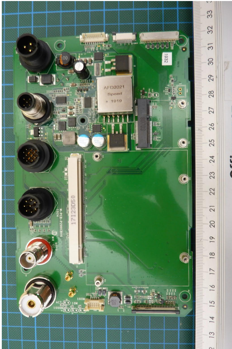
P200-CS, PCB3, top view
