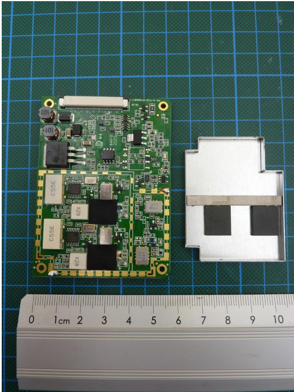
P200-CS, PCB4, top view (shielding removed)
