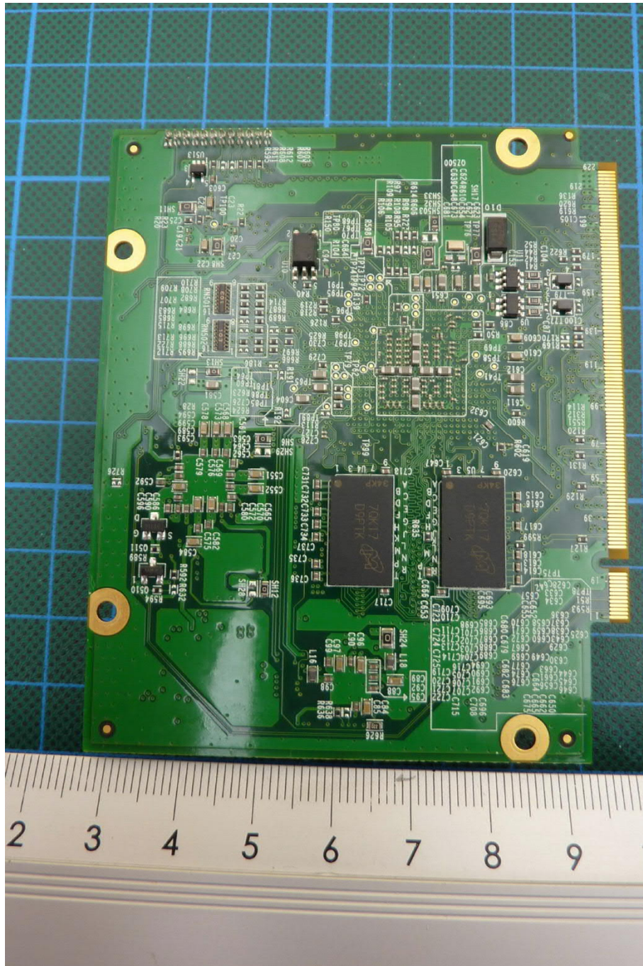
P200-CS, PCB1, bottom view
