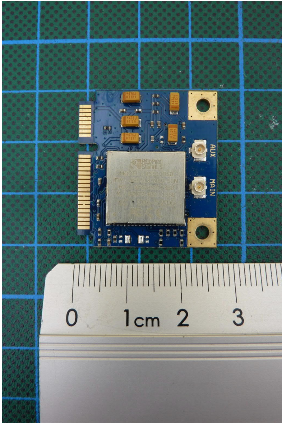
P200-CS, PCB2, top view
