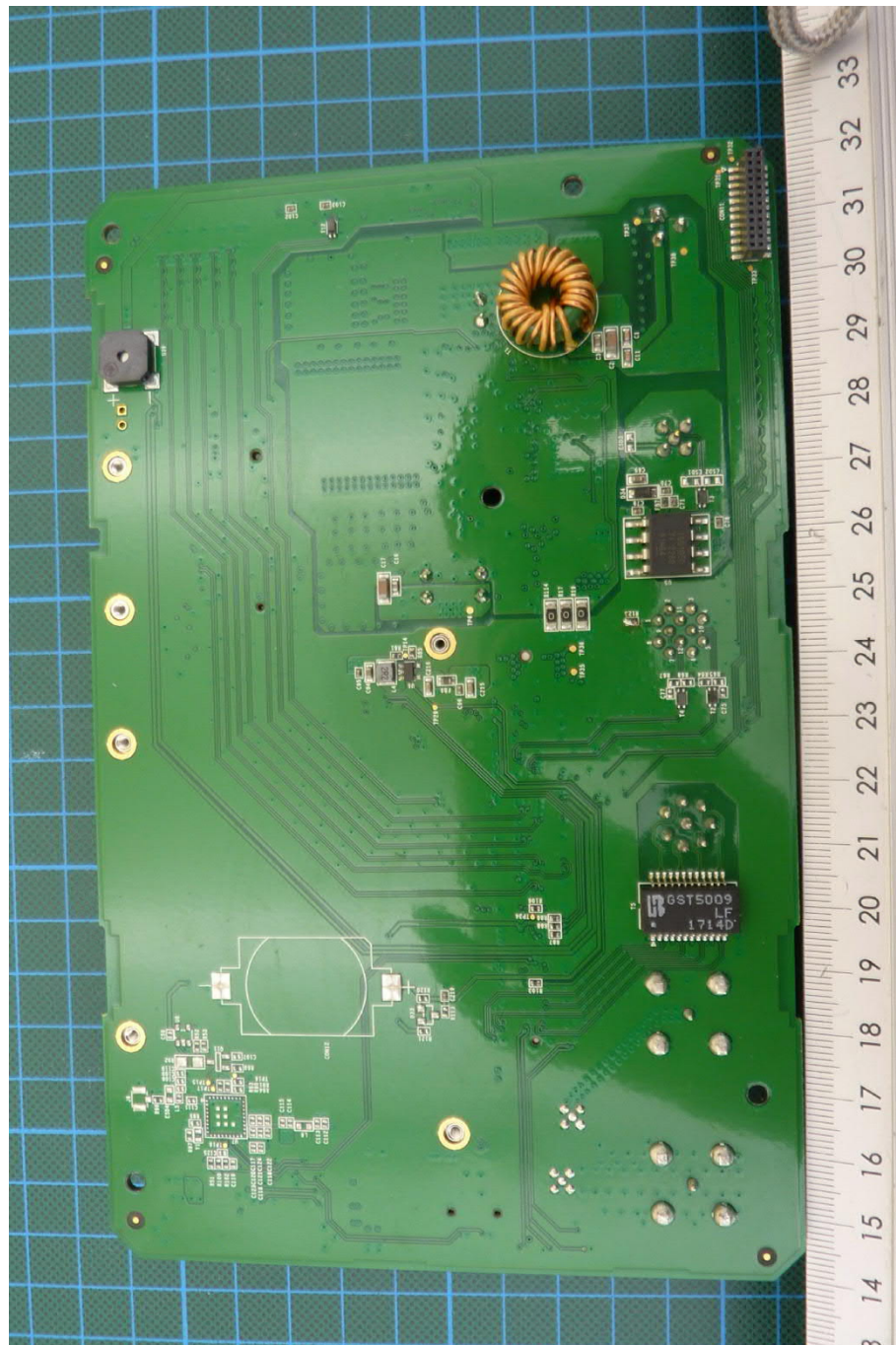
P200-CS, PCB3, bottom view
