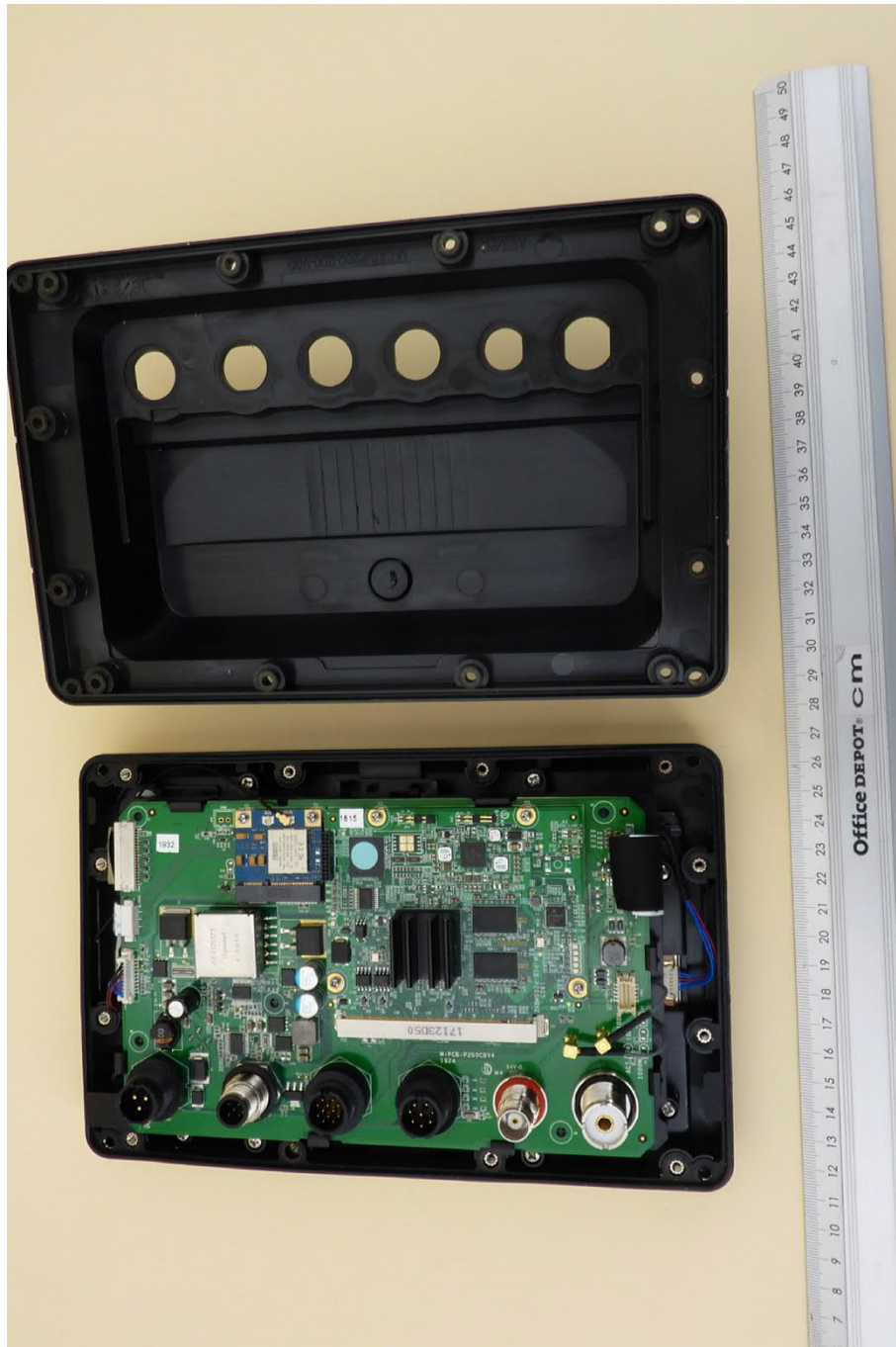
P200-CS, internal view 1 (housing opened)
