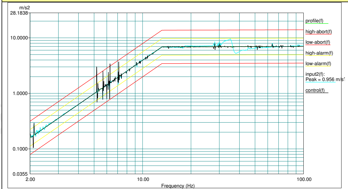
5. Vibration Test Profile (Resonance Search: Z axis)
