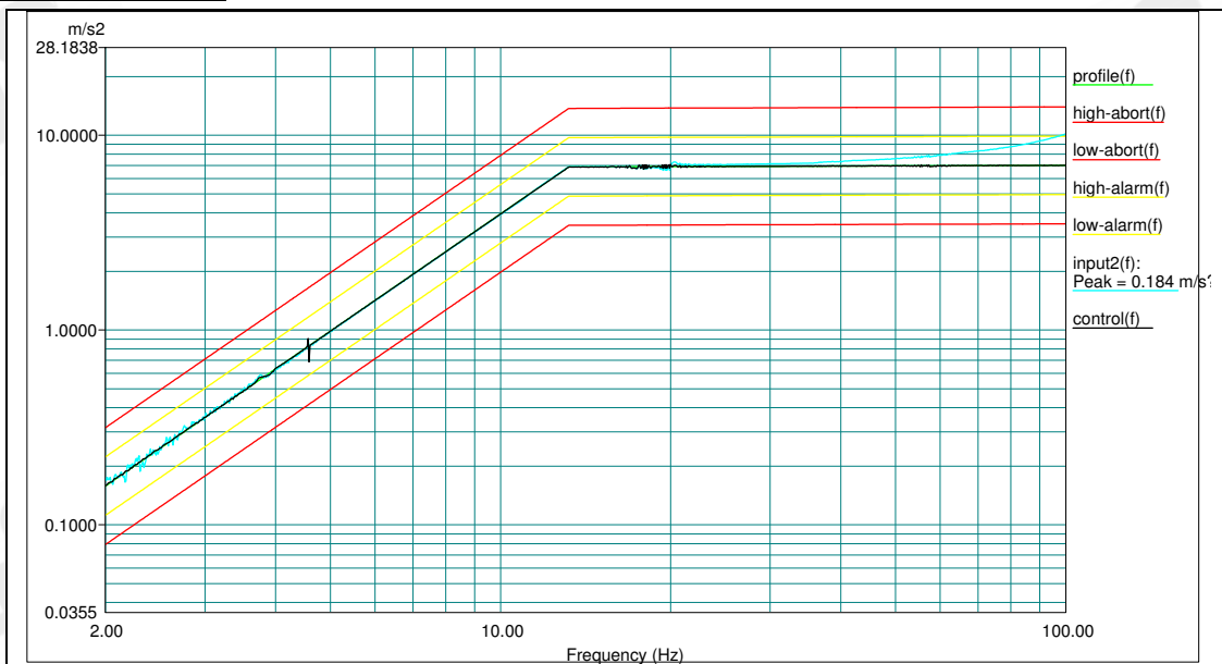
4. Vibration Test Profile (Resonance Search: Y axis)
