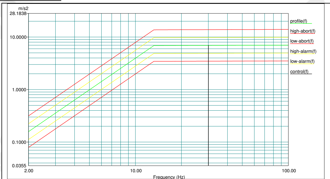
6. Vibration Test Profile (Dwell: X axis)
