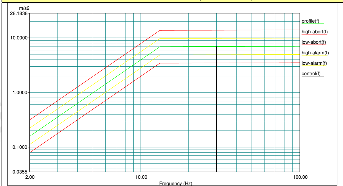
7. Vibration Test Profile (Dwell: Y axis)
