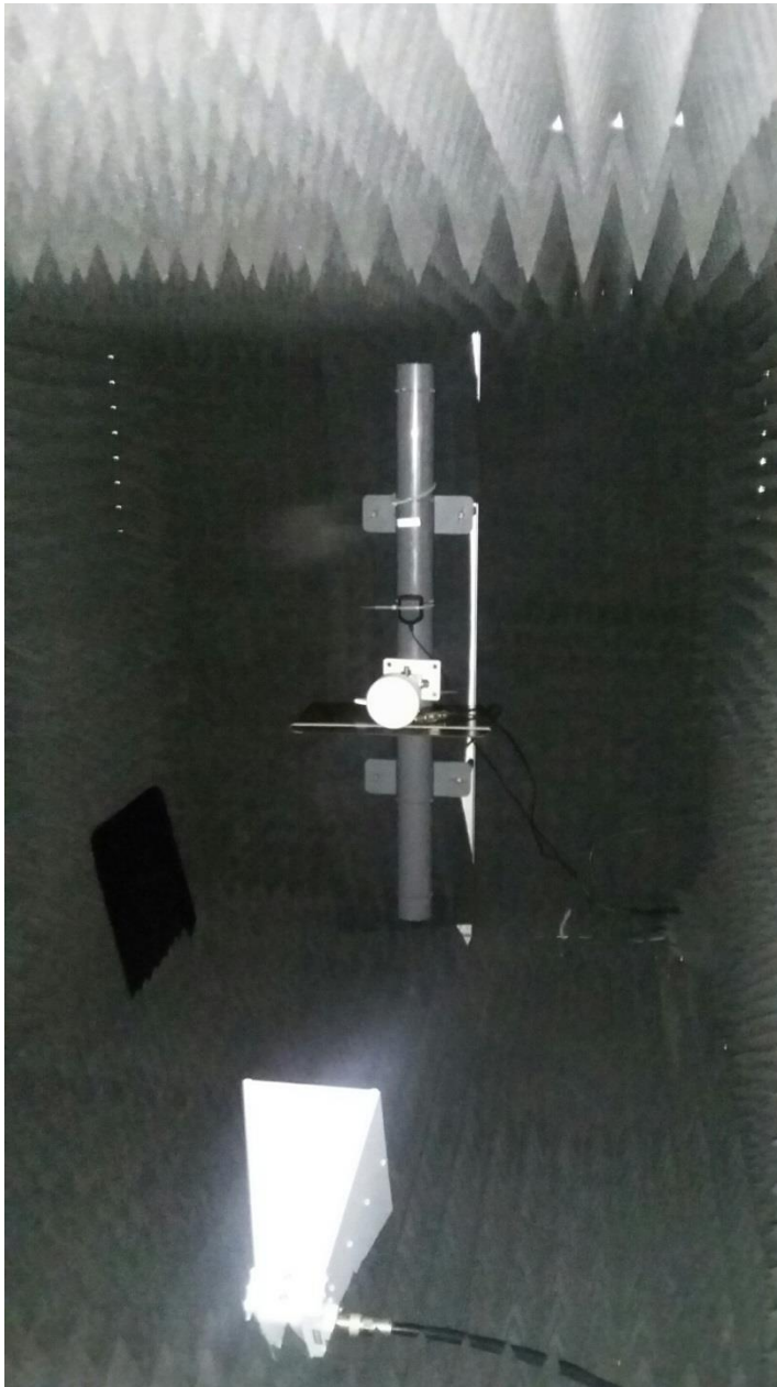
EUT antenna inside RF-Chamber
