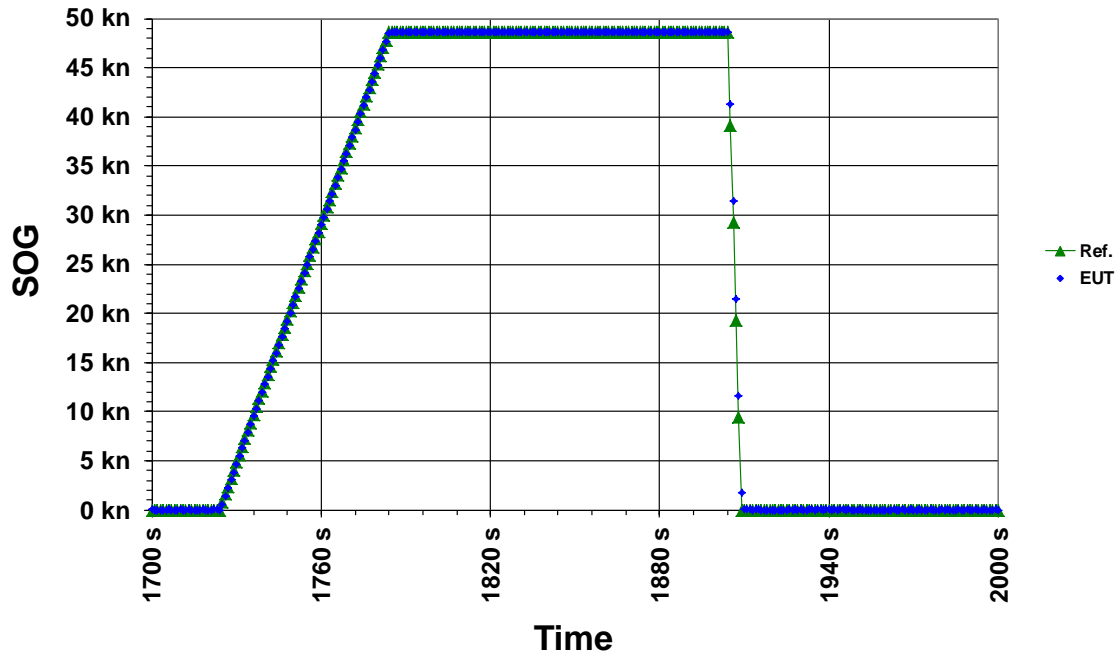
Speed over ground (SOG)
