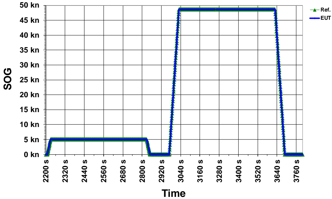
SOG vs. time for 5knots and 48.6 knots
