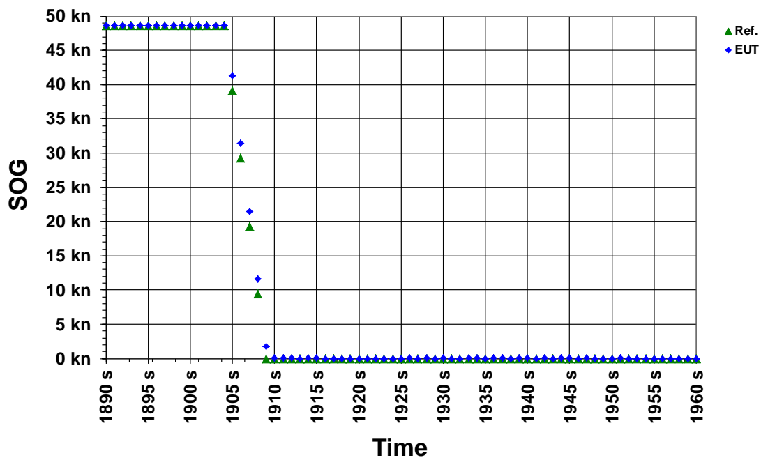
Speed over ground, coming to rest position
