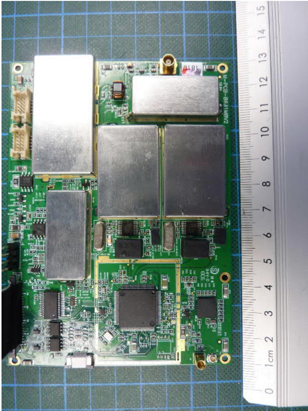
190014_9.jpg: WIDELINK B600S, PCB 3, top view
