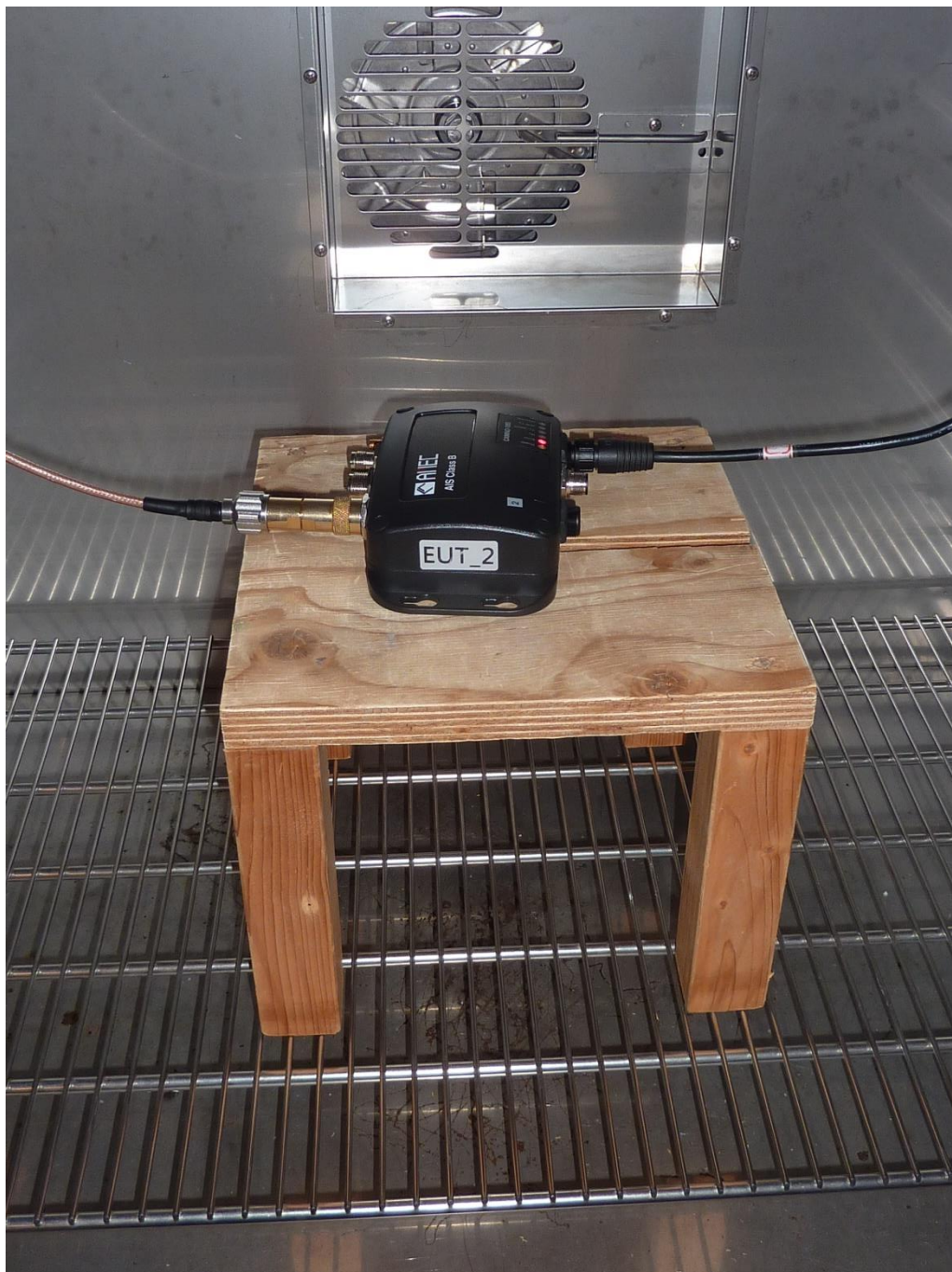
190015_c.jpg: CAMINO-108S, test setup temperature chamber
