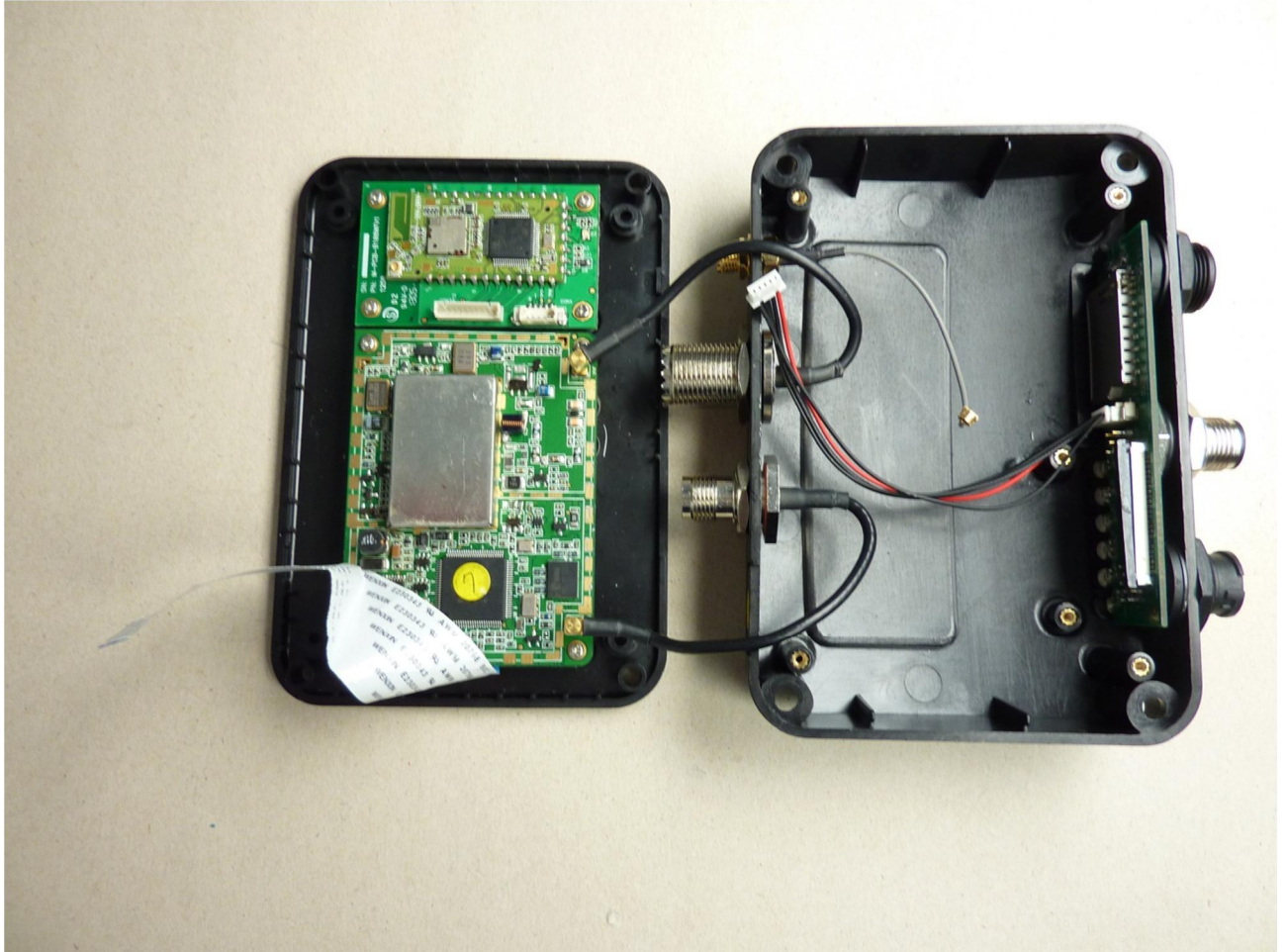
130840eut3.jpg: EUT, inside-view
