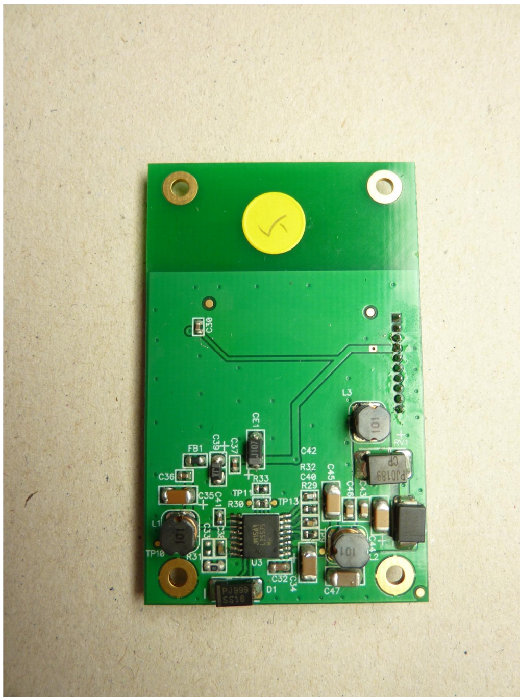
123924eut6.jpg: M-PCB, rear-view
