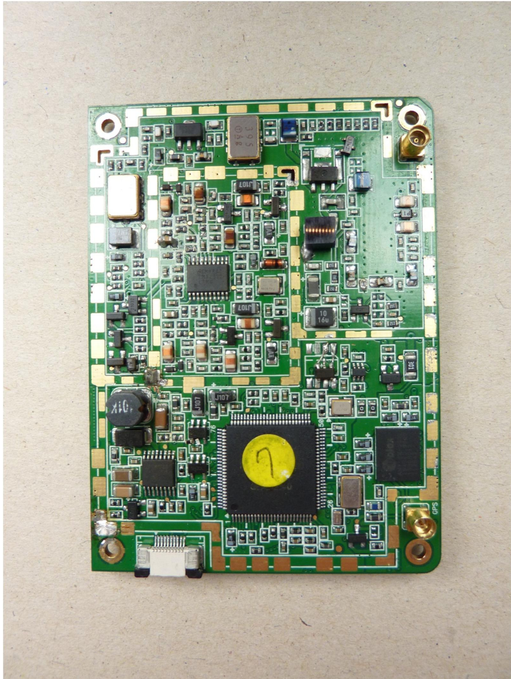
123924eut8.jpg: Main-PCB, front-view
