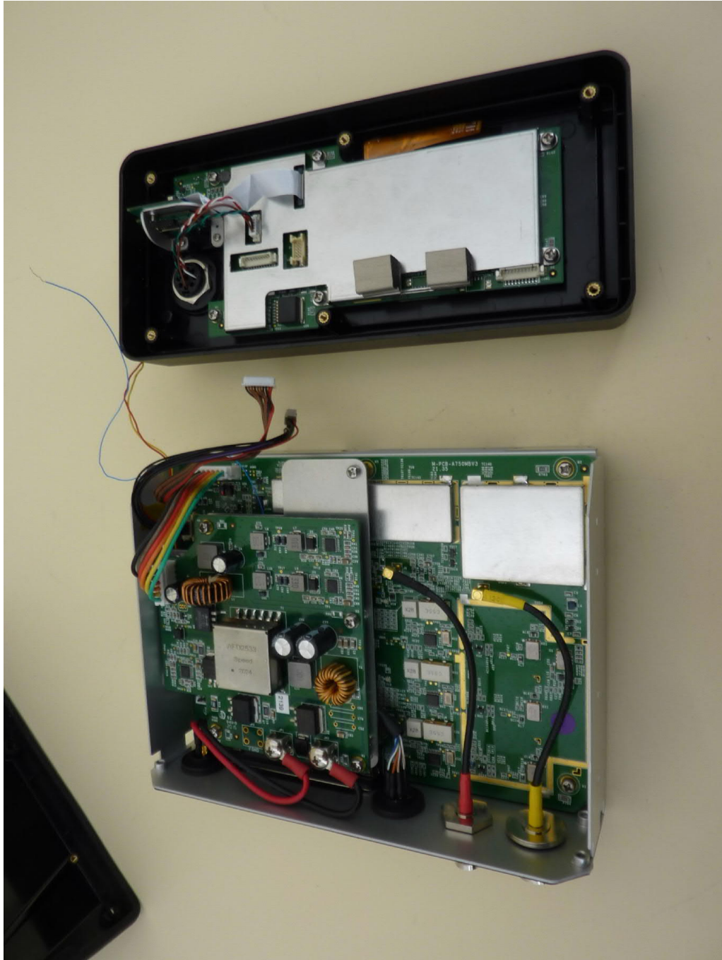
Internal view, front cover and main part
