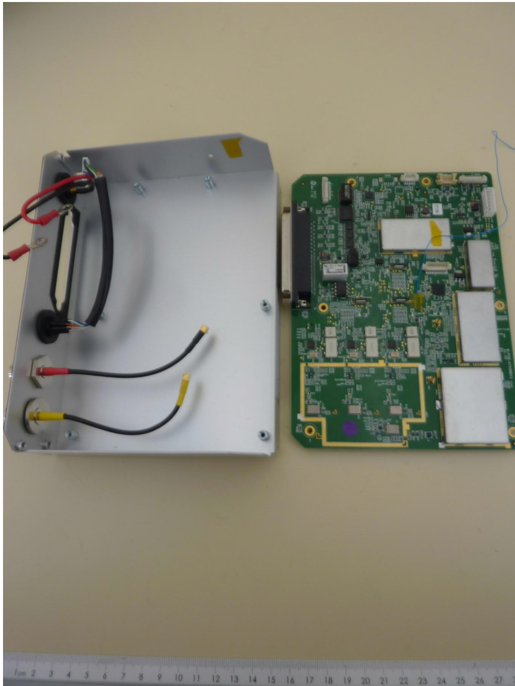
Main part, main PCB removed
