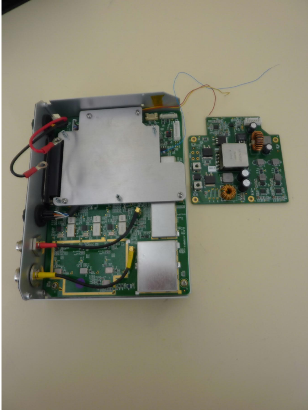
Main part, PCB 4 removed
