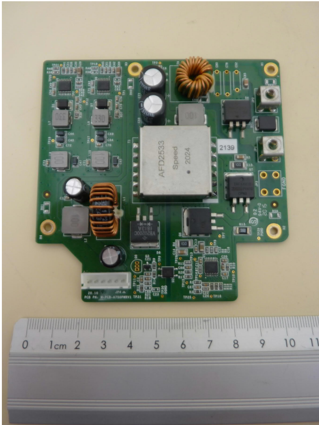
PCB 4, top view
