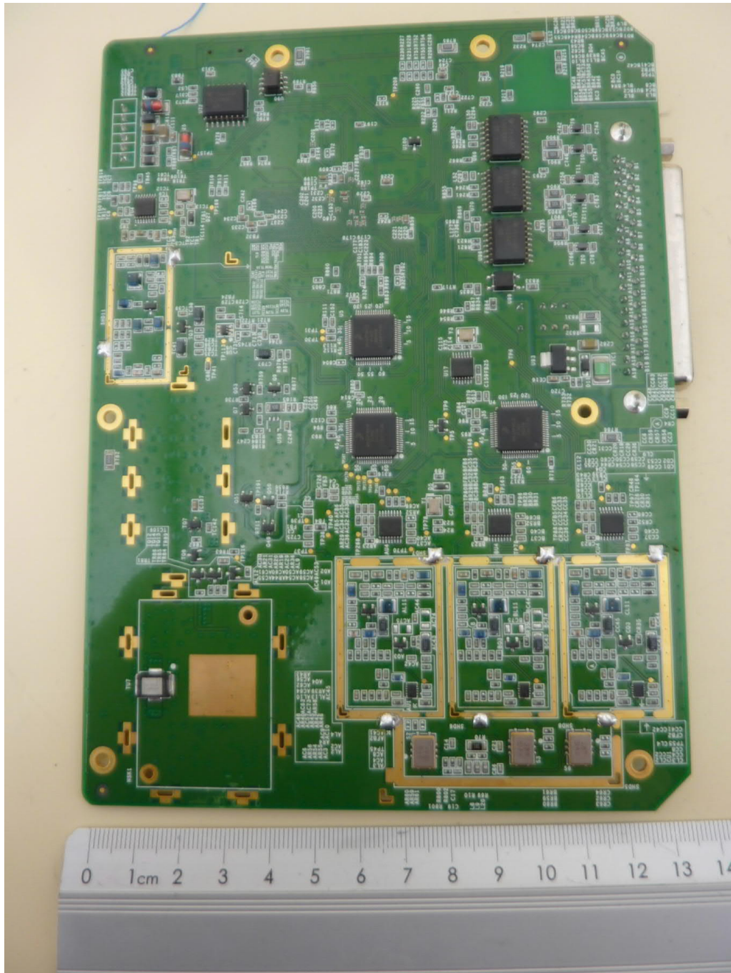
PCB 5, bottom view, shieldings removed
