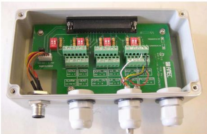
(1) Junction Box internal photo #1
