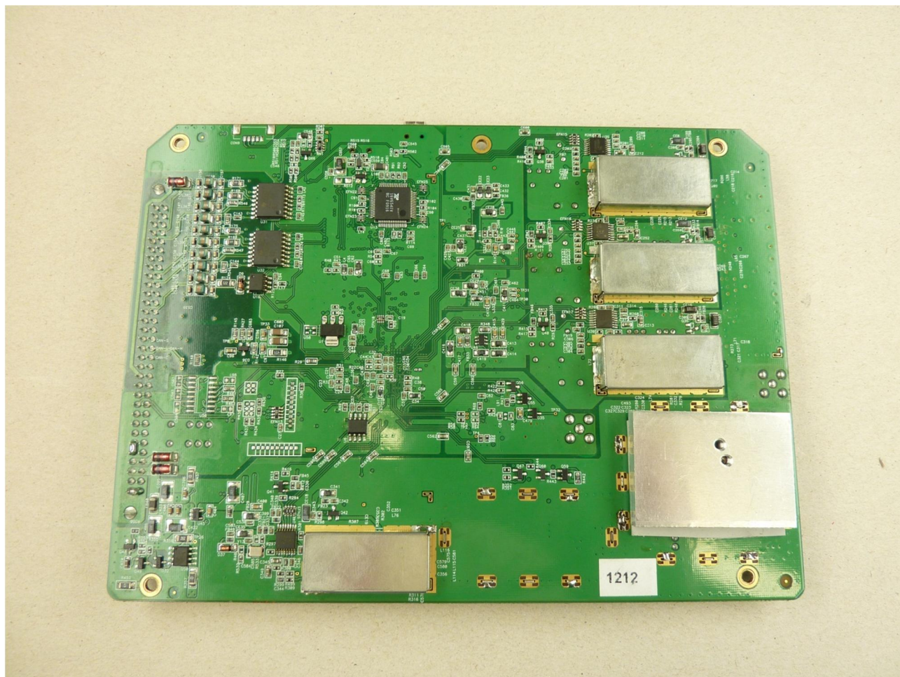
123924eut7.jpg: RF-PCB, rear view
