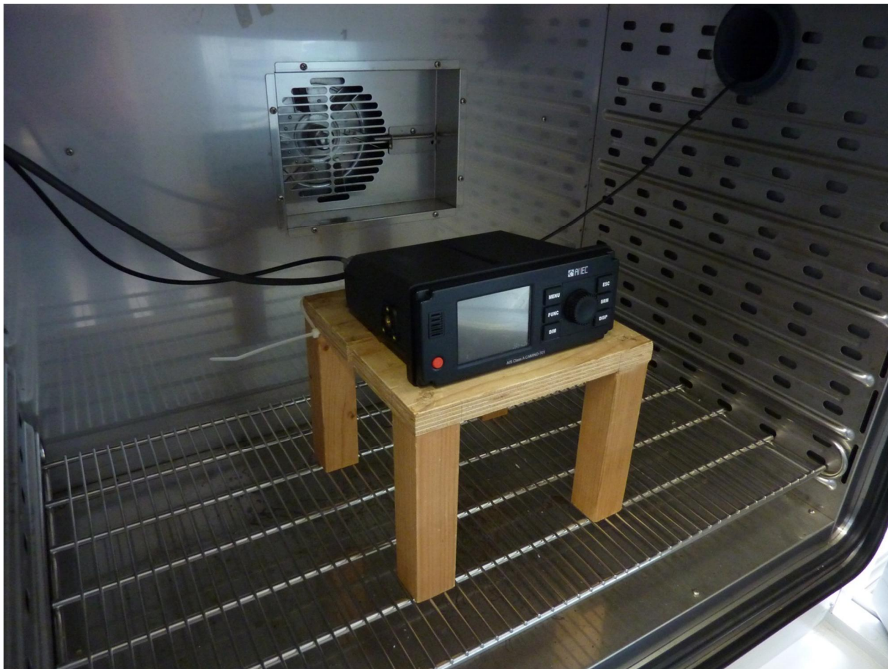
123924clima1.jpg: Test set-up climatic chamber
