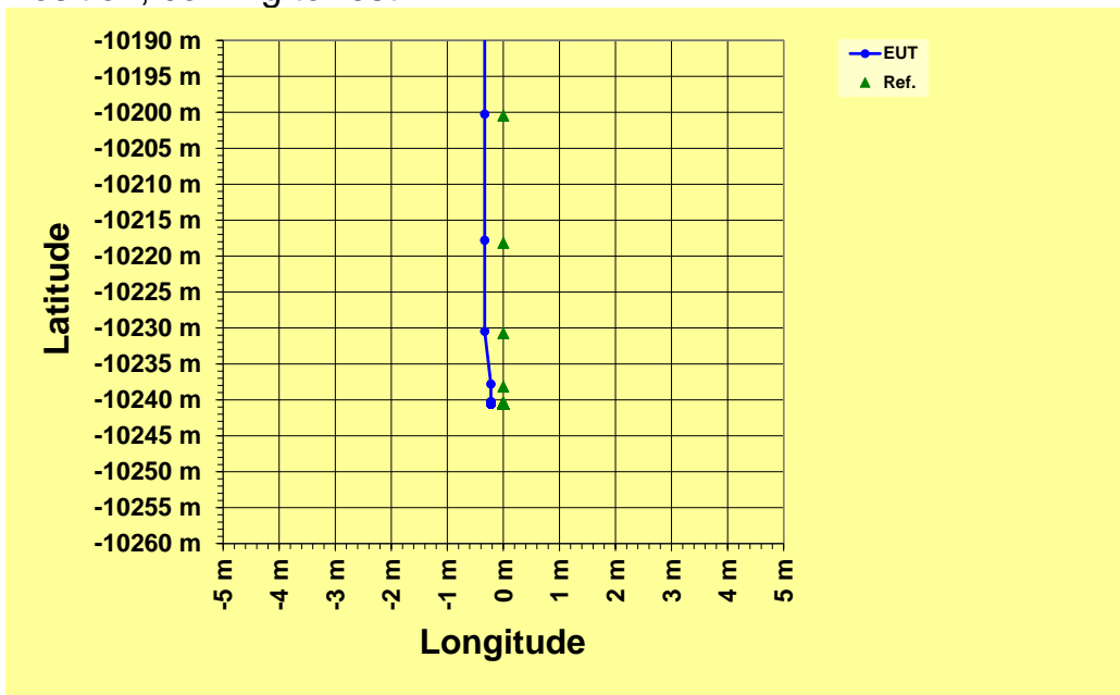
Position, coming to rest
