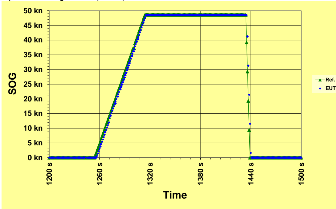
Speed over ground (SOG) vs. time
