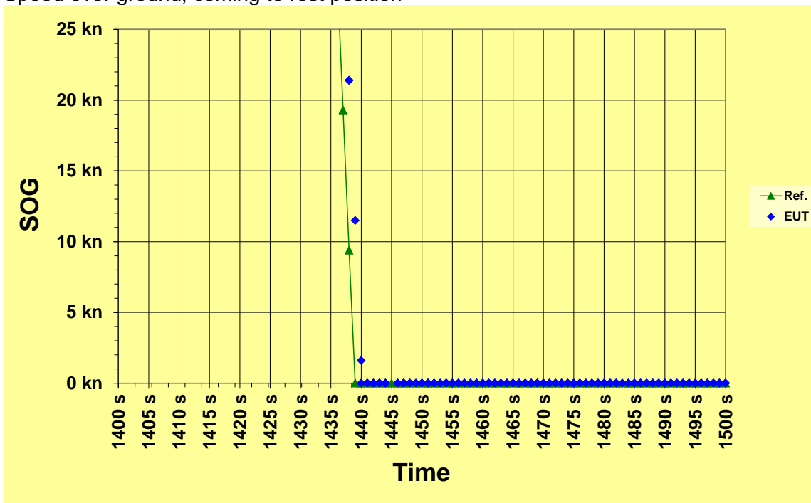
Speed over ground, coming to rest position
