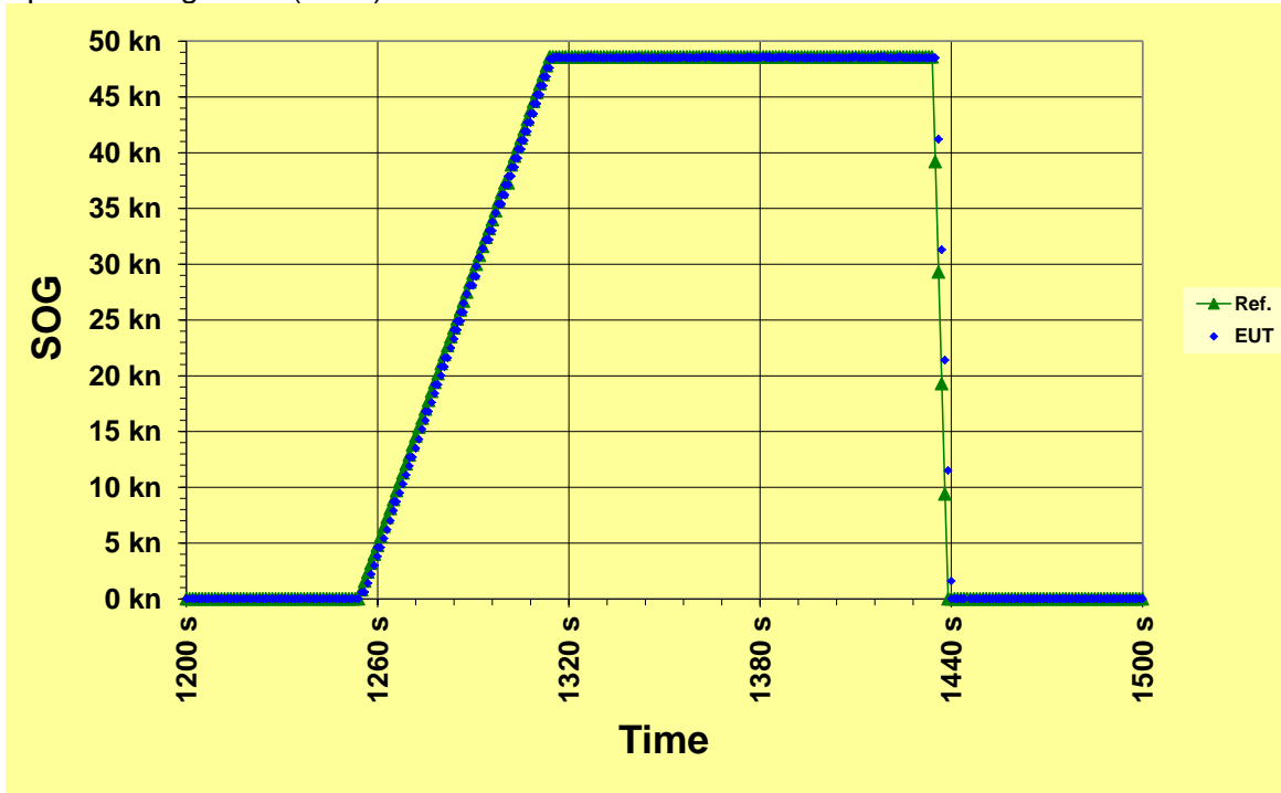
Speed over ground (SOG)
