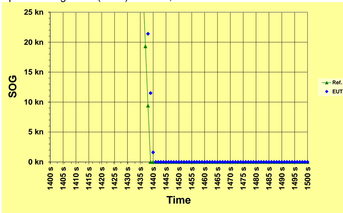
Speed over ground (SOG) vs. time, detail
