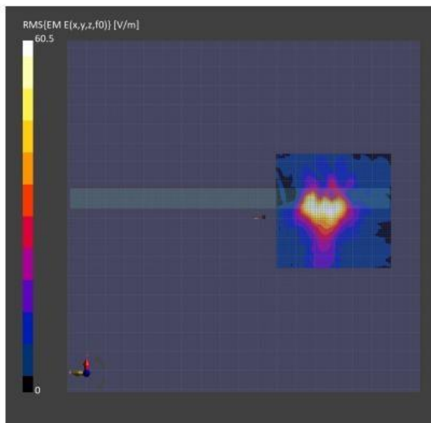
Figure8-3: 4cm 2 -averaged power density distribution measured at input.power.limit of 2.61 dBm on the Back for n260 beam 18
