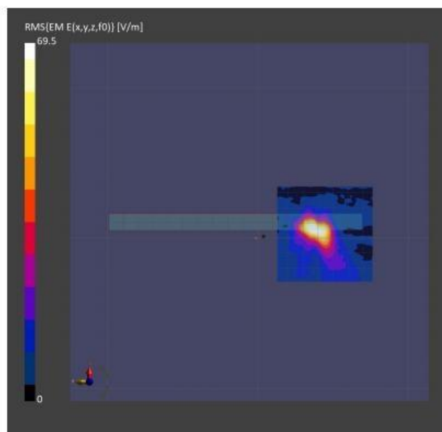
Figure 8-4: 4cm2-averaged power density distribution measured at input.power.limit of 2.35dBm on the back surface for n261 beam 15
