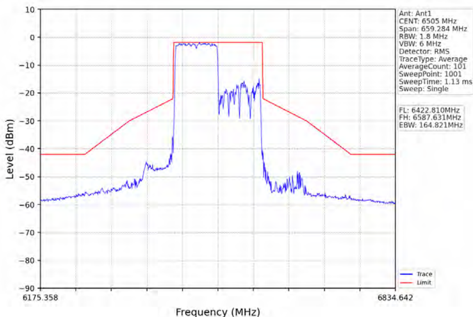
802.11ax(HEW160)_HCH_6505MHz_RU996_Right_Ant1_NTNV
