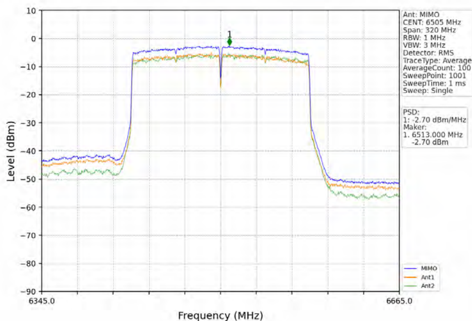
802.11ax(HEW160)_HCH_6505MHz_2xRU996_Left_MIMO_NTNV
