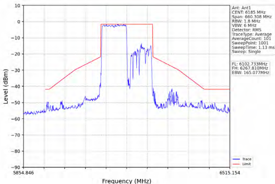
802.11ax(HEW160)_MCH_6185MHz_RU996_Right_Ant1_NTNV
