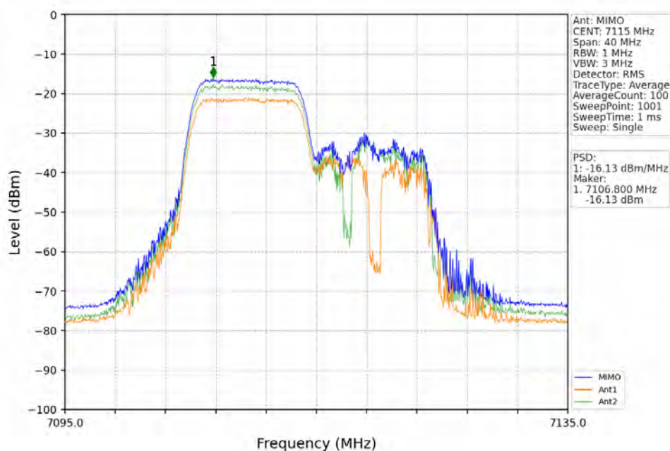
802.11ax(HEW20)_HCH_7115MHz_RU106_Right_MIMO_NTNV
