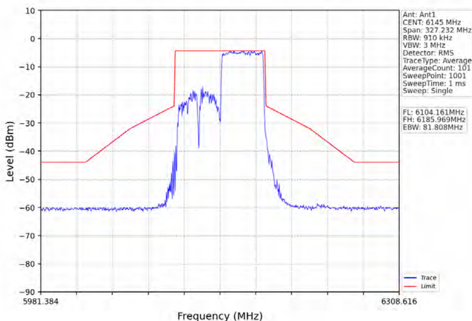
802.11ax(HEW80)_MCH_6145MHz_RU996_Left_Ant1_NTNV
