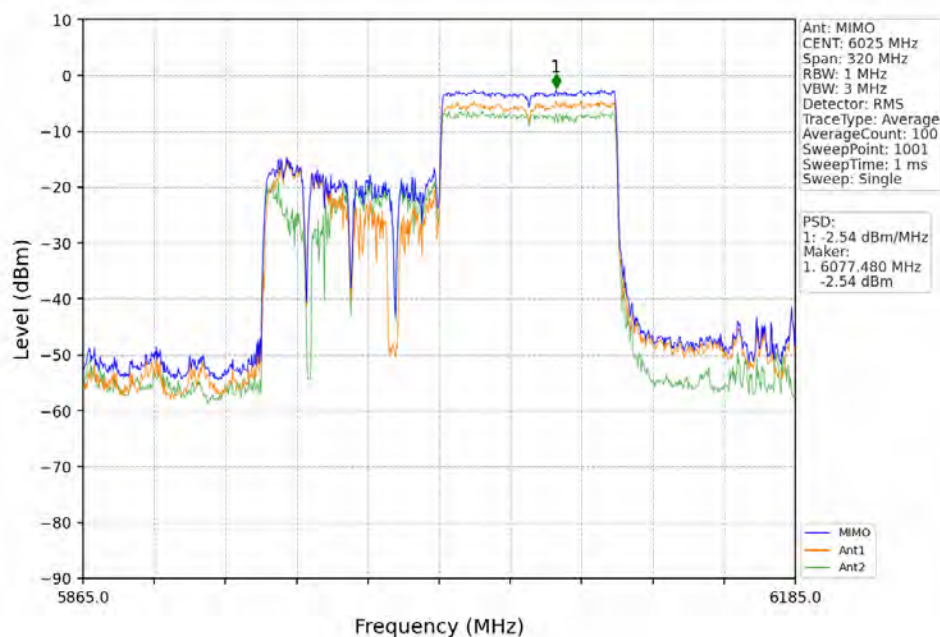
802.11ax(HEW160)_LCH_6025MHz_RU996_Left_MIMO_NTNV
