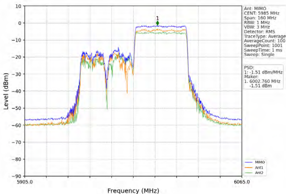
802.11ax(HEW80)_LCH_5985MHz_RU484_Right_MIMO_NTNV
