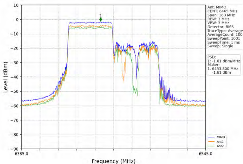
802.11ax(HEW80)_LCH_6465MHz_RU484_Left_MIMO_NTNV
