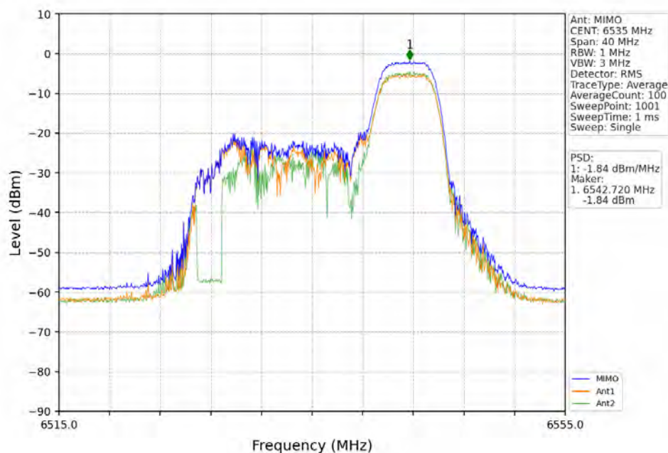
802.11ax(HEW20)_LCH_6535MHz_RU52_Right_MIMO_NTNV
