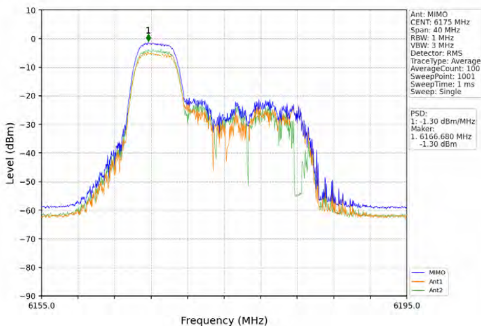
802.11ax(HEW20)_MCH_6175MHz_RU52_Left_MIMO_NTNV
