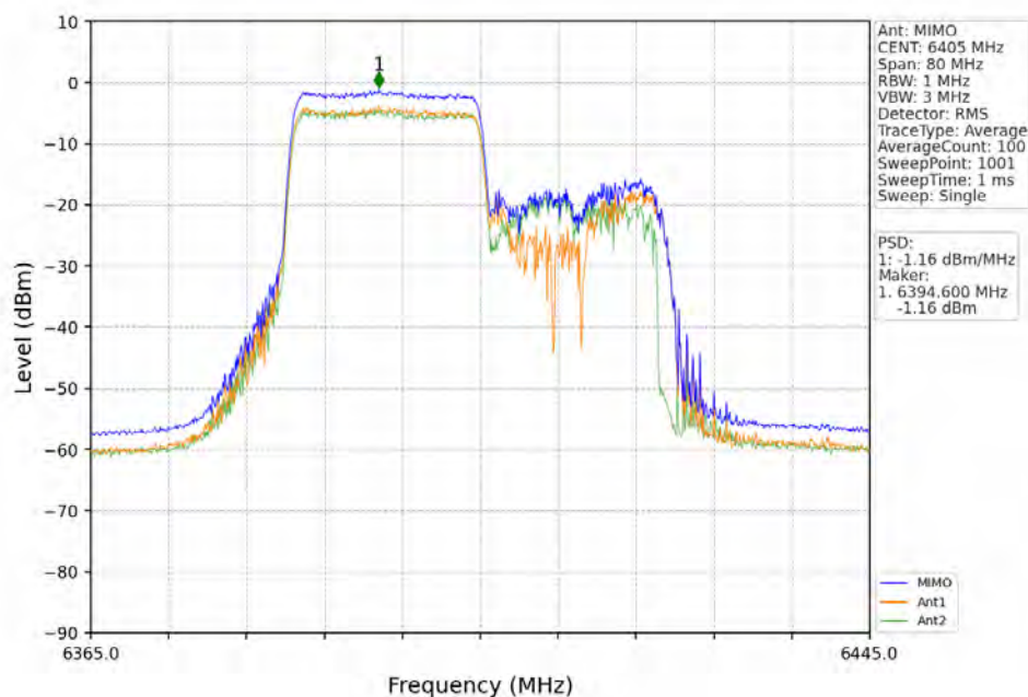
802.11ax(HEW40)_HCH_6405MHz_RU242_Left_MIMO_NTNV
