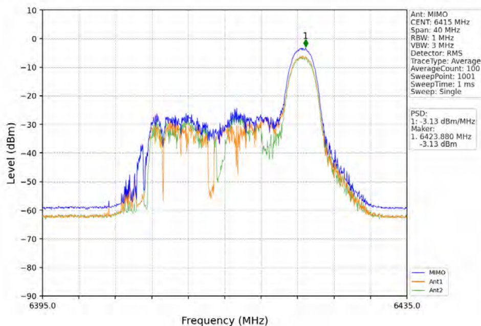
802.11ax(HEW20)_HCH_6415MHz_RU26_Right_MIMO_NTNV
