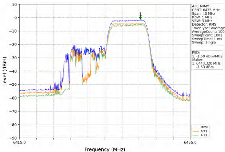
802.11ax(HEW20)_LCH_6435MHz_RU106_Right_MIMO_NTNV
