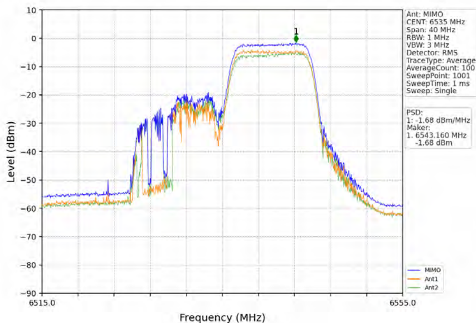
802.11ax(HEW20)_LCH_6535MHz_RU106_Right_MIMO_NTNV
