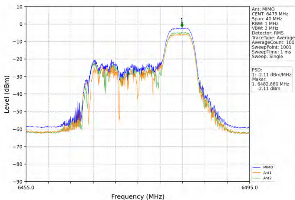
802.11ax(HEW20)_MCH_6475MHz_RU106_Left_MIMO_NTNV
