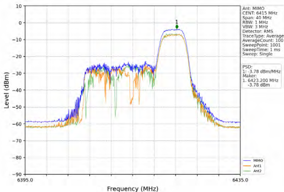
802.11ax(HEW20)_HCH_6415MHz_RU52_Right_MIMO_NTNV
