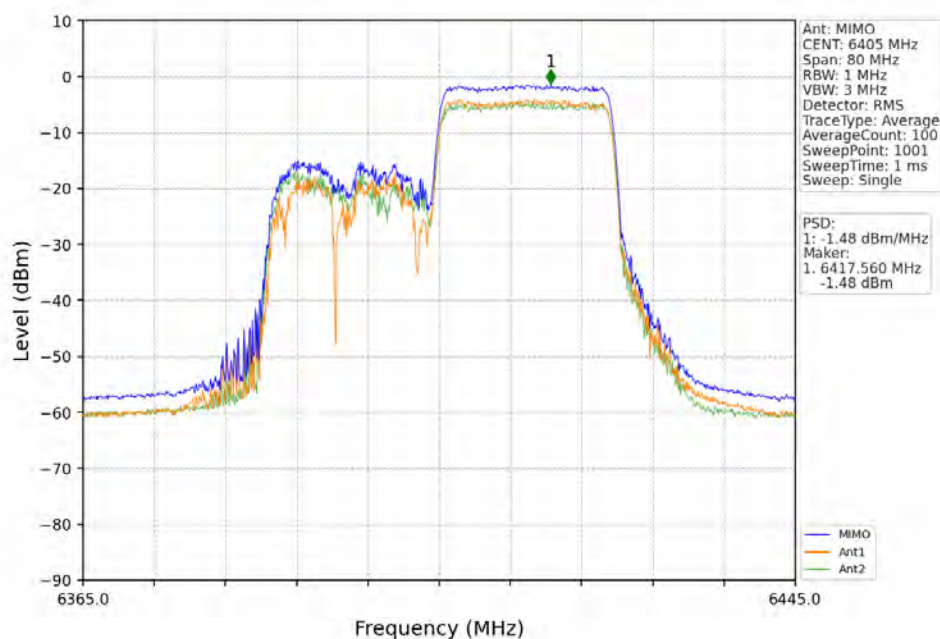
802.11ax(HEW40)_HCH_6405MHz_RU484_Left_MIMO_NTNV
