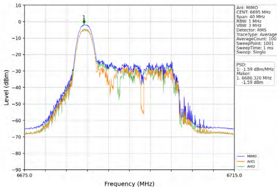
802.11ax(HEW20)_MCH_6695MHz_RU26_Left_MIMO_NTNV
