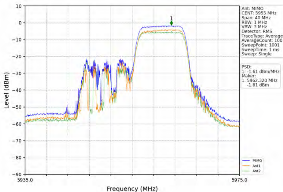
802.11ax(HEW20)_LCH_5955MHz_RU106_Right_MIMO_NTNV
