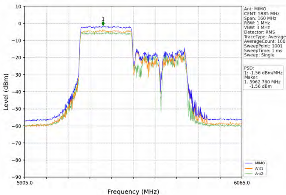
802.11ax(HEW80)_LCH_5985MHz_RU484_Right_MIMO_NTNV
