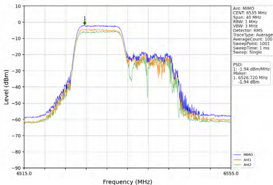
802.11ax(HEW20)_LCH_6535MHz_RU106_Right_MIMO_NTNV
