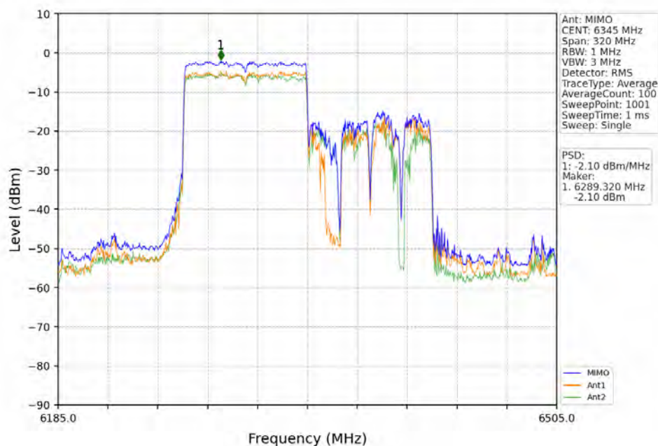
802.11ax(HEW160)_HCH_6345MHz_RU996_Left_MIMO_NTNV
