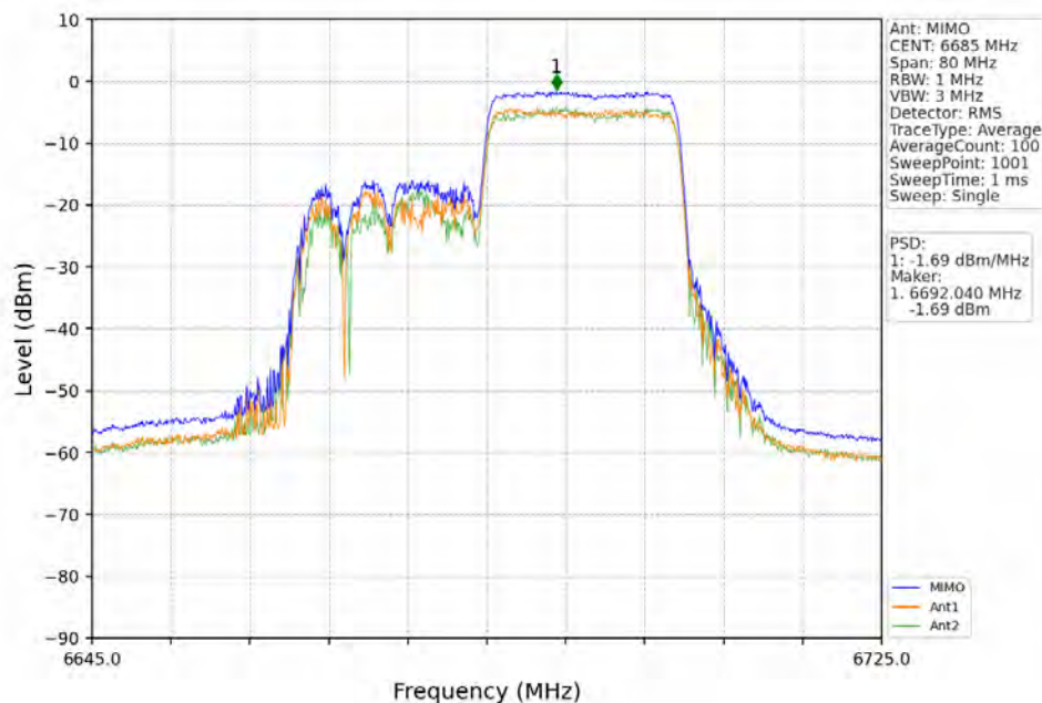
802.11ax(HEW40)_MCH_6685MHz_RU242_Right_MIMO_NTNV
