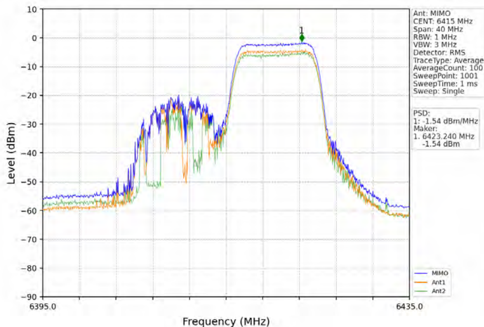
802.11ax(HEW20)_HCH_6415MHz_RU106_Right_MIMO_NTNV
