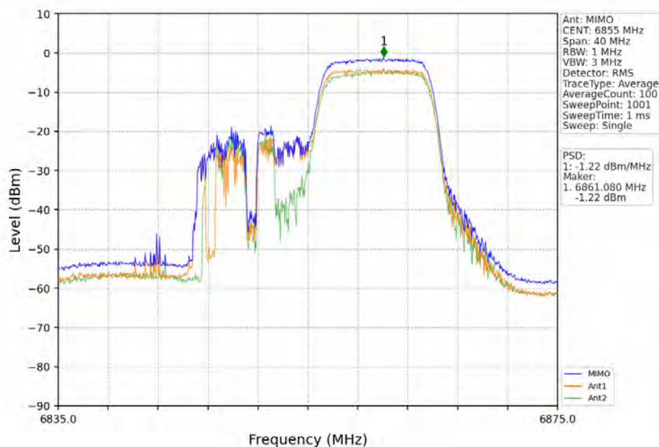
802.11ax(HEW20)_HCH_6855MHz_RU106_Right_MIMO_NTNV
