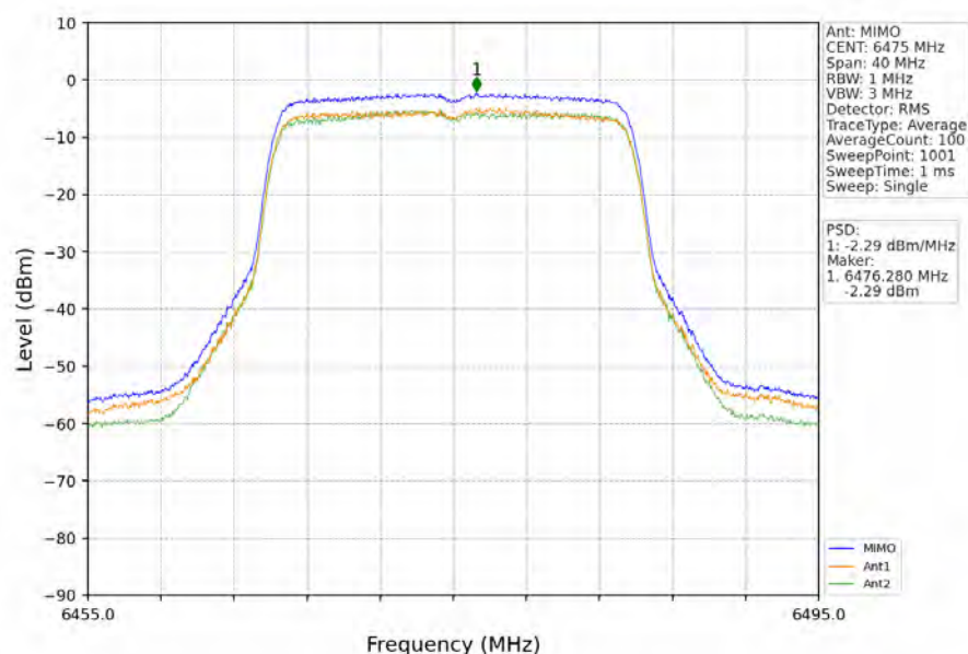
802.11ax(HEW20)_MCH_6475MHz_RU242_Left_MIMO_NTNV
