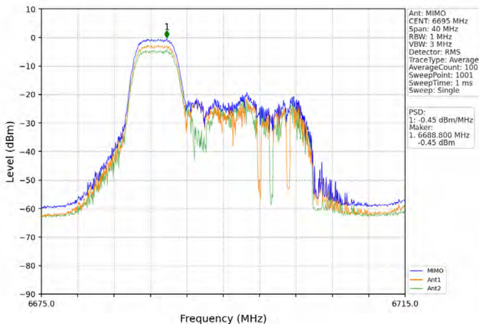
802.11ax(HEW20)_MCH_6695MHz_RU52_Left_MIMO_NTNV
