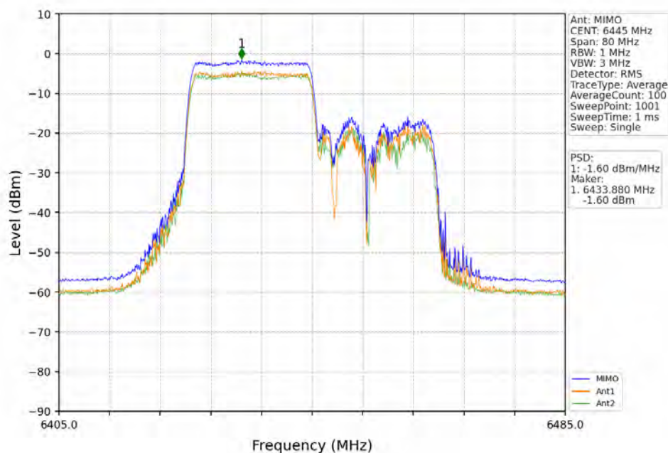
802.11ax(HEW40)_LCH_6445MHz_RU242_Left_MIMO_NTNV
