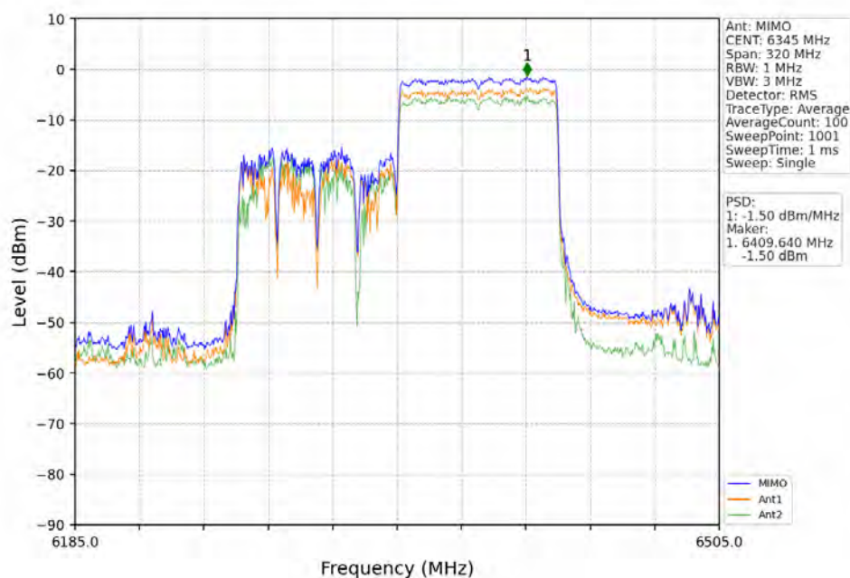
802.11ax(HEW160)_HCH_6345MHz_2xRU996_Left_MIMO_NTNV
