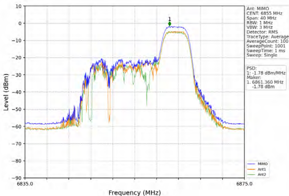
802.11ax(HEW20)_HCH_6855MHz_RU52_Right_MIMO_NTNV
