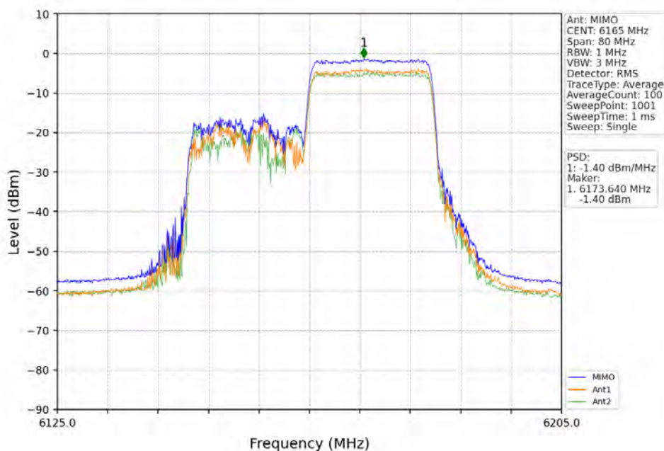
802.11ax(HEW40)_MCH_6165MHz_RU242_Right_MIMO_NTNV
