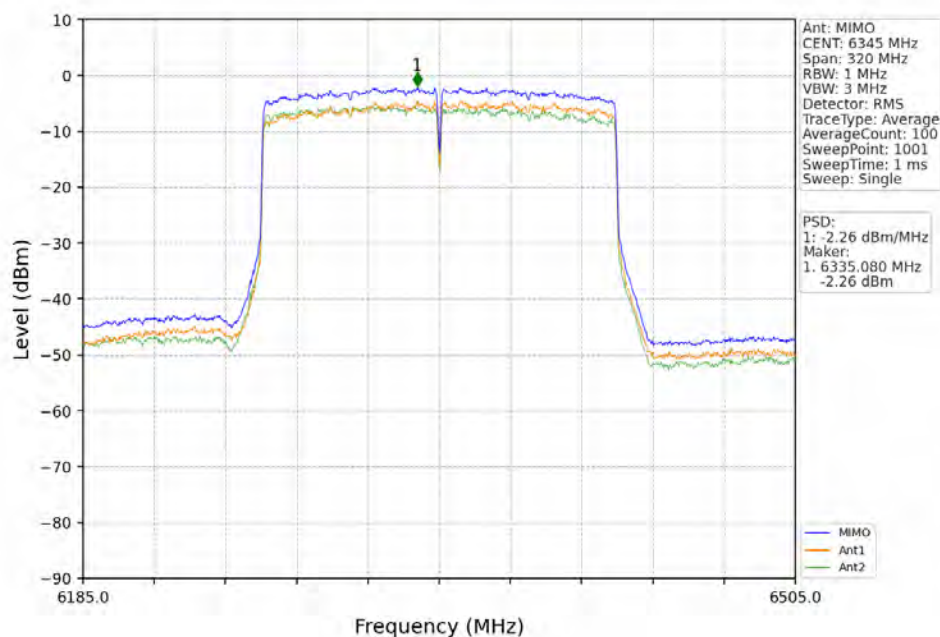
802.11ax(HEW160)_HCH_6345MHz_2xRU996_Left_MIMO_NTNV
