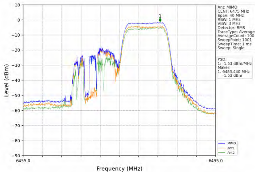
802.11ax(HEW20)_MCH_6475MHz_RU242_Left_MIMO_NTNV
