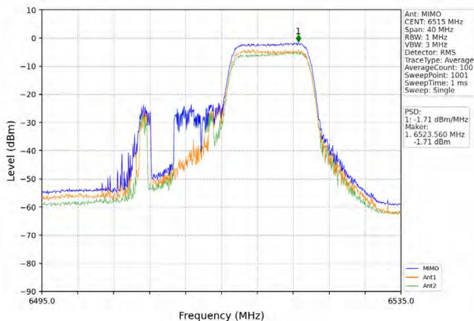
802.11ax(HEW20)_HCH_6515MHz_RU106_Right_MIMO_NTNV
