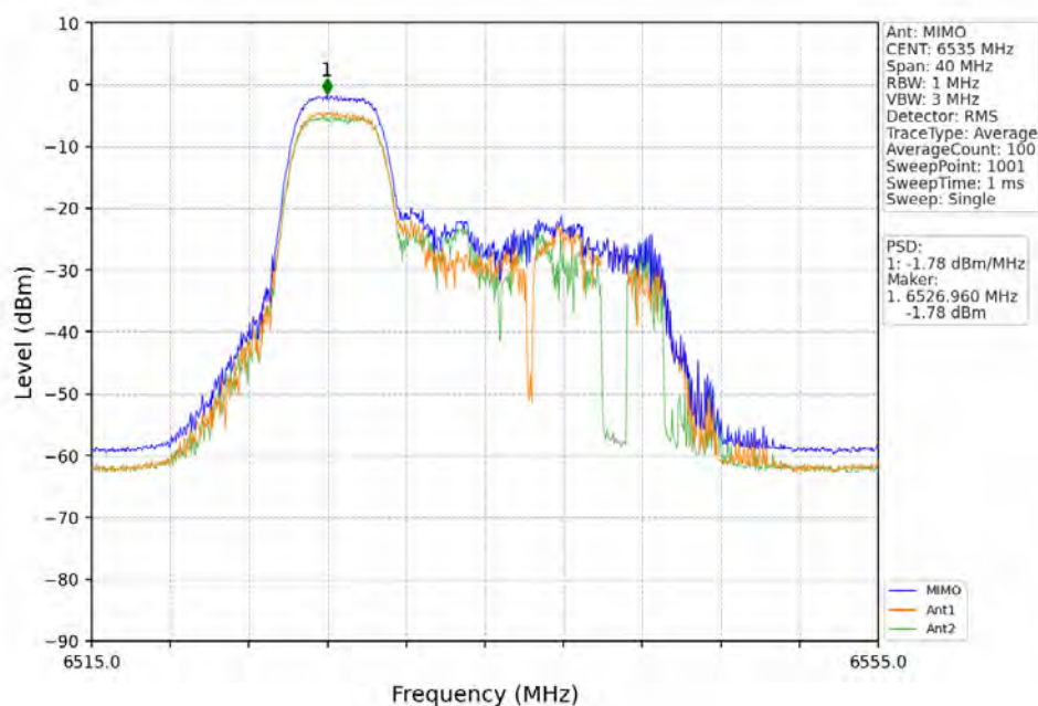
802.11ax(HEW20)_LCH_6535MHz_RU52_Right_MIMO_NTNV
