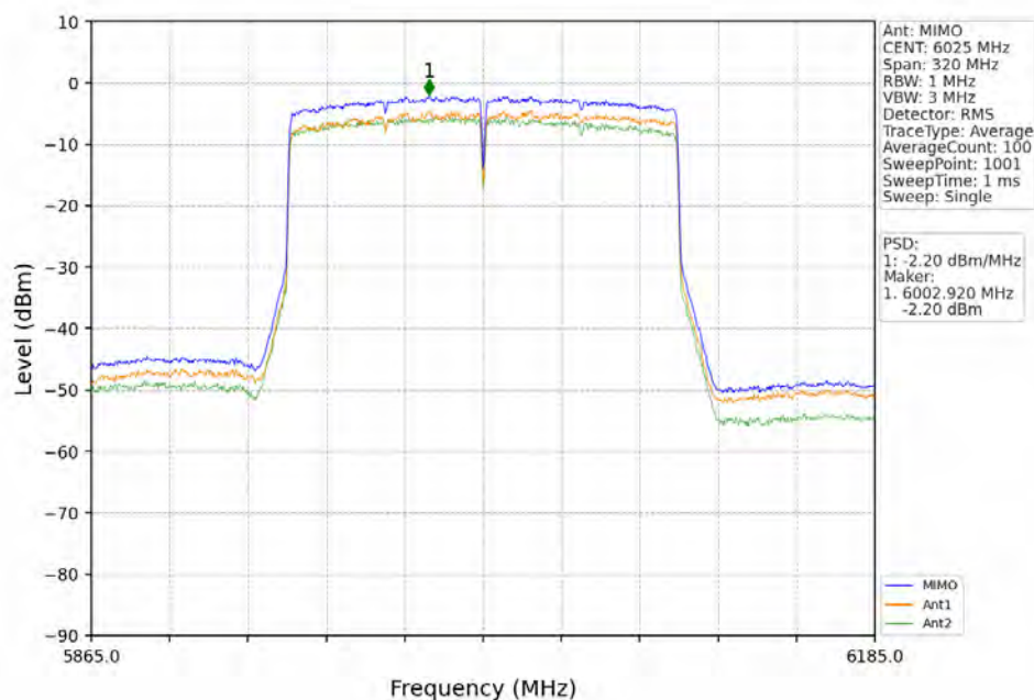
802.11ax(HEW160)_LCH_6025MHz_2xRU996_Left_MIMO_NTNV
