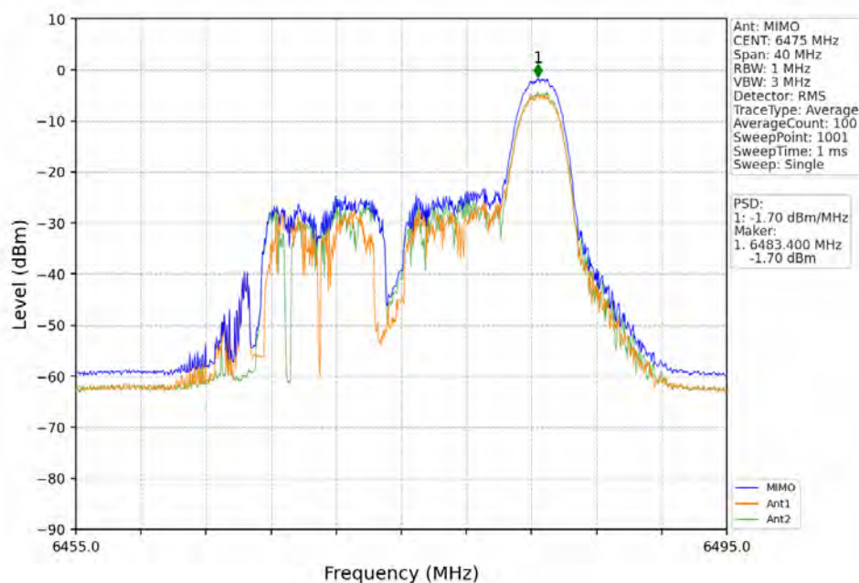
802.11ax(HEW20)_MCH_6475MHz_RU52_Left_MIMO_NTNV
