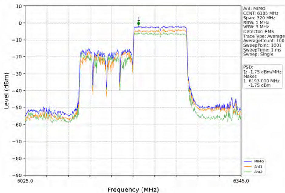
802.11ax(HEW160)_MCH_6185MHz_RU996_Right_MIMO_NTNV
