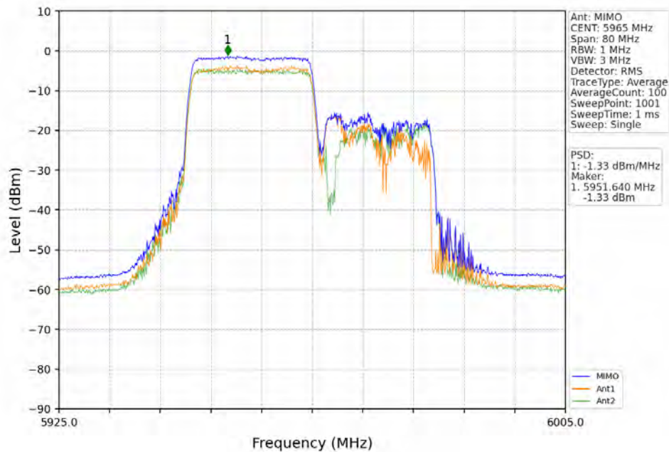
802.11ax(HEW40)_LCH_5965MHz_RU242_Left_MIMO_NTNV
