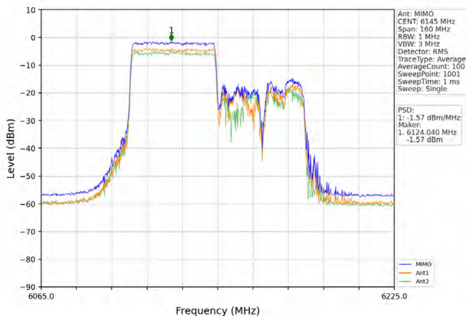
802.11ax(HEW80)_MCH_6145MHz_RU484_Left_MIMO_NTNV
