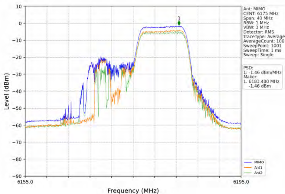
802.11ax(HEW20)_MCH_6175MHz_RU242_Left_MIMO_NTNV
