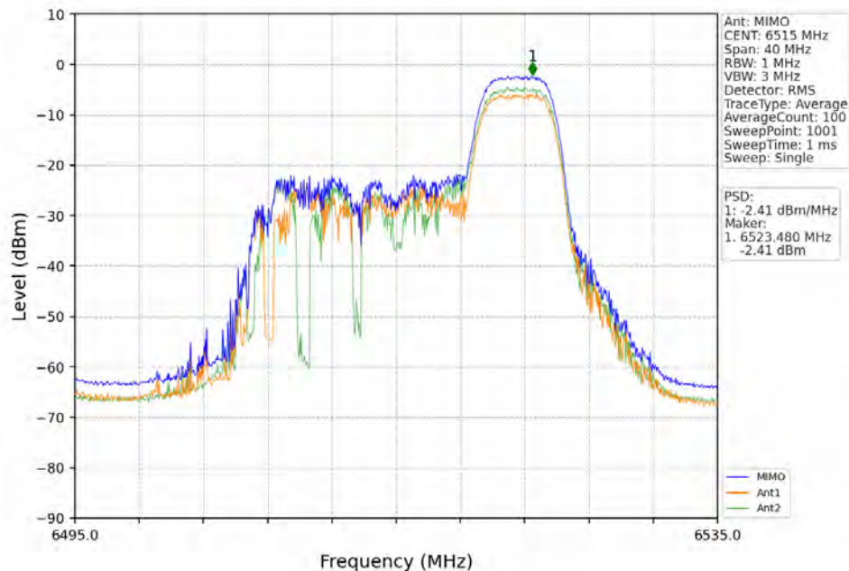
802.11ax(HEW20)_HCH_6515MHz_RU52_Right_MIMO_NTNV
