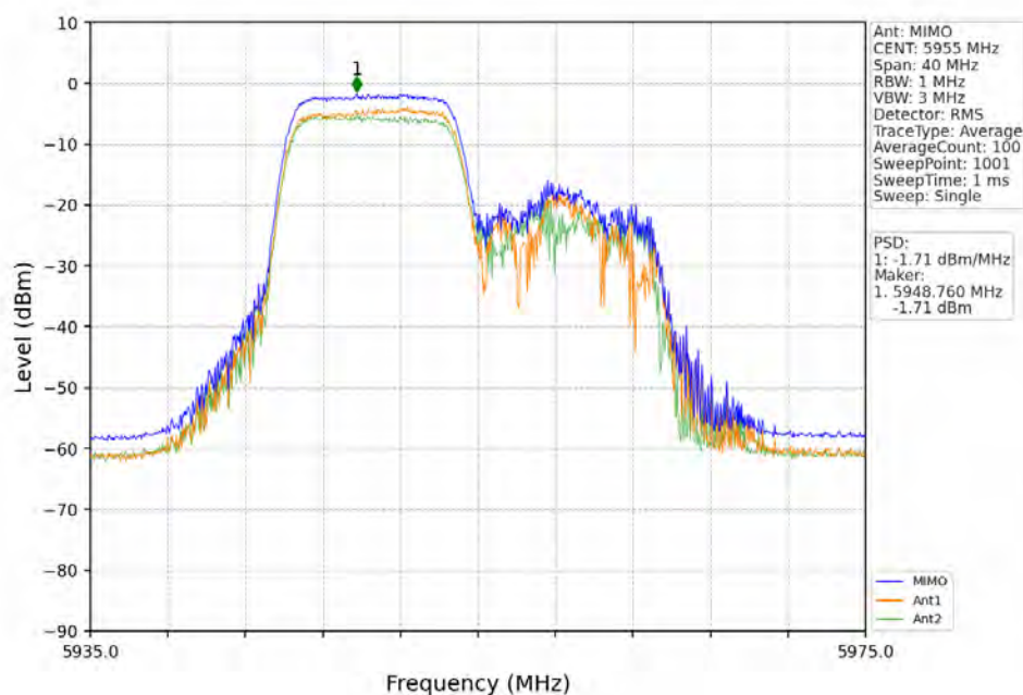
802.11ax(HEW20)_LCH_5955MHz_RU106_Right_MIMO_NTNV
