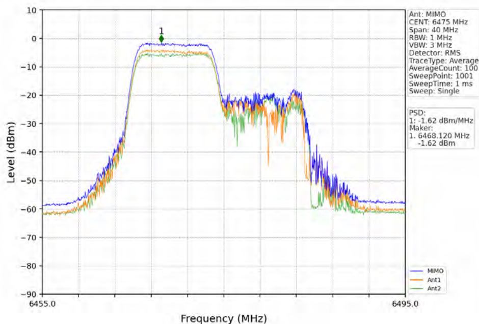
802.11ax(HEW20)_MCH_6475MHz_RU106_Left_MIMO_NTNV
