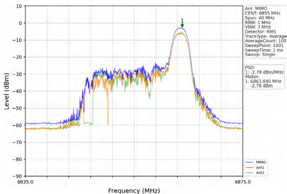
802.11ax(HEW20)_HCH_6855MHz_RU26_Right_MIMO_NTNV
