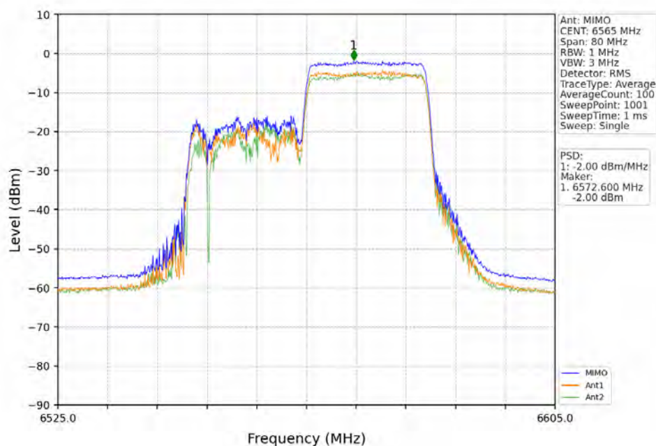
802.11ax(HEW40)_LCH_6565MHz_RU484_Left_MIMO_NTNV
