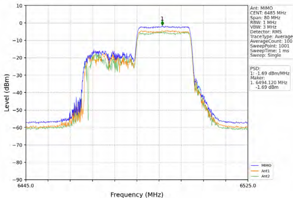
802.11ax(HEW40)_MCH_6485MHz_RU242_Right_MIMO_NTNV
