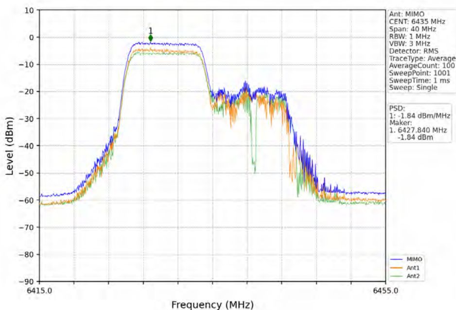
802.11ax(HEW20)_LCH_6435MHz_RU106_Right_MIMO_NTNV
