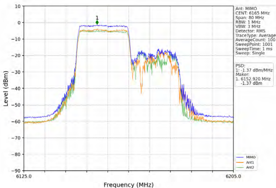
802.11ax(HEW40)_MCH_6165MHz_RU242_Right_MIMO_NTNV
