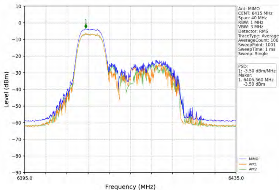
802.11ax(HEW20)_HCH_6415MHz_RU52_Right_MIMO_NTNV
