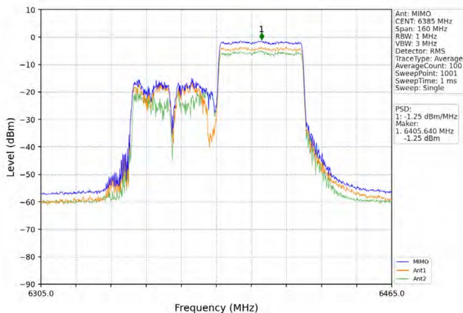
802.11ax(HEW80)_HCH_6385MHz_RU484_Right_MIMO_NTNV
