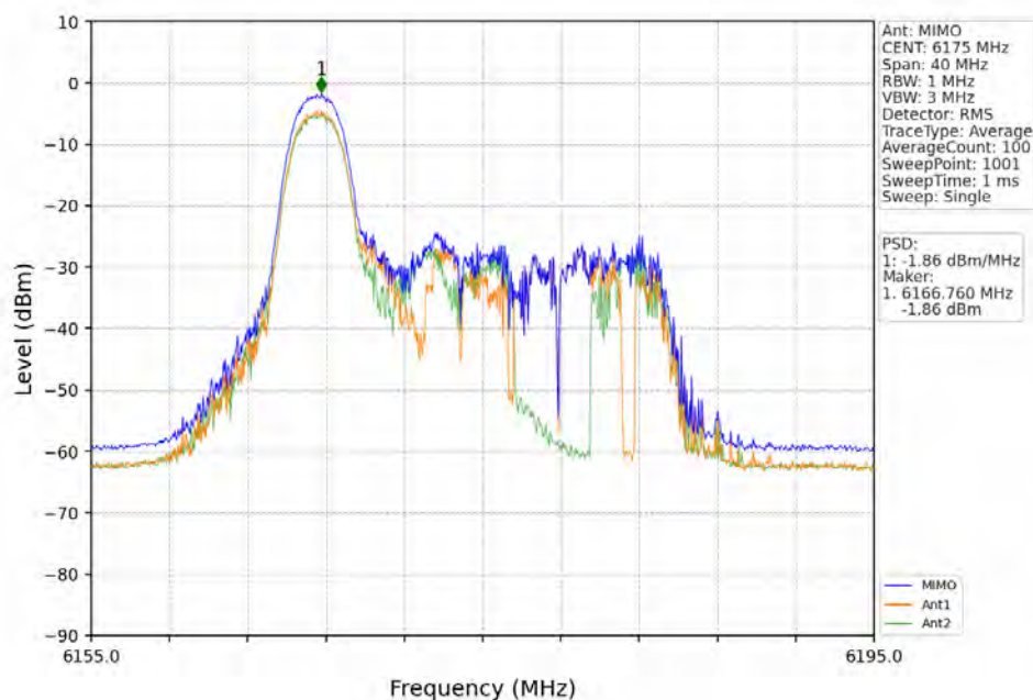
802.11ax(HEW20)_MCH_6175MHz_RU26_Left_MIMO_NTNV
