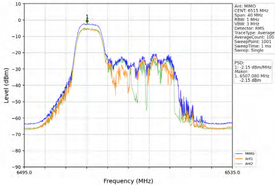
802.11ax(HEW20)_HCH_6515MHz_RU52_Right_MIMO_NTNV
