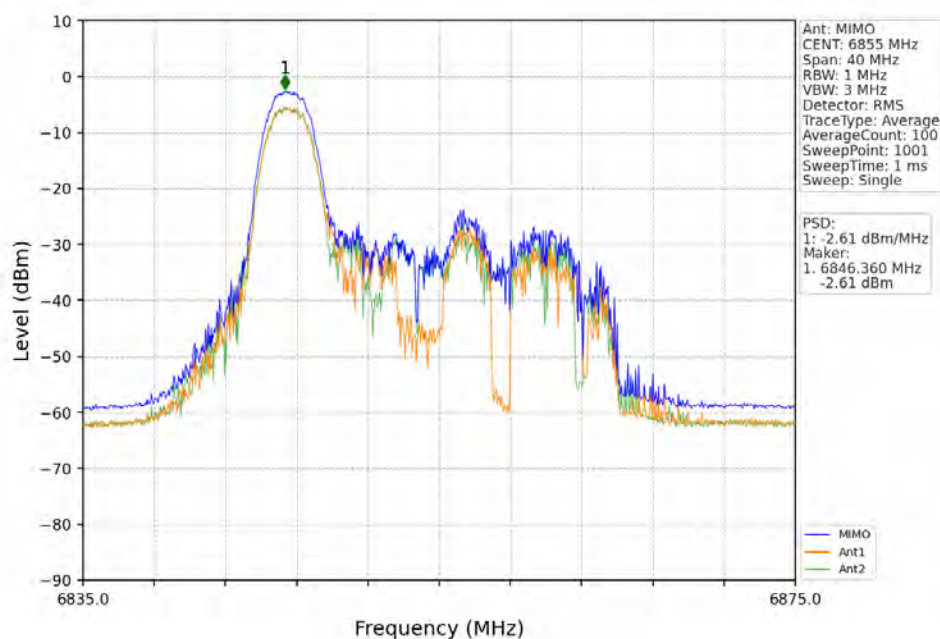
802.11ax(HEW20)_HCH_6855MHz_RU26_Right_MIMO_NTNV
