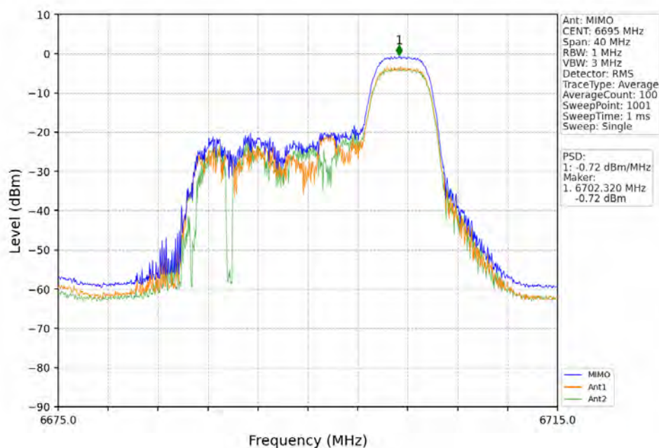
802.11ax(HEW20)_MCH_6695MHz_RU106_Left_MIMO_NTNV
