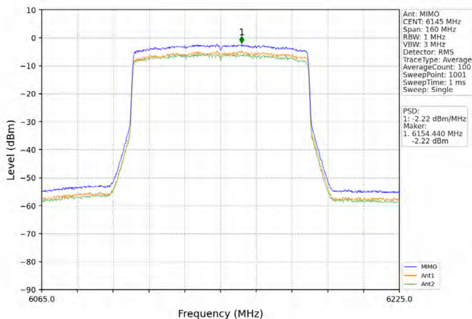
802.11ax(HEW80)_MCH_6145MHz_RU996_Left_MIMO_NTNV
