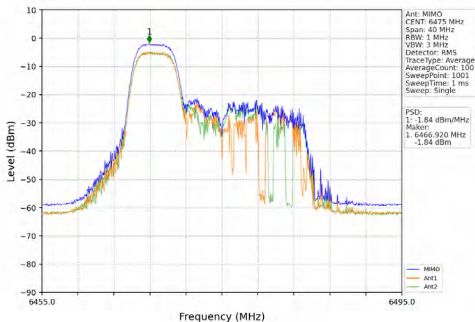
802.11ax(HEW20)_MCH_6475MHz_RU52_Left_MIMO_NTNV
