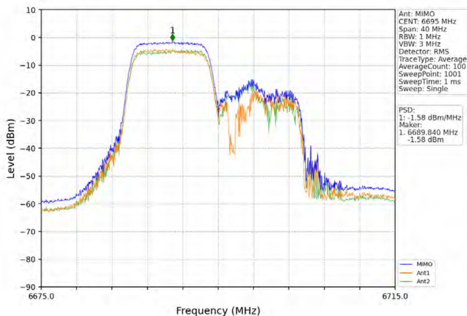
802.11ax(HEW20)_MCH_6695MHz_RU106_Left_MIMO_NTNV
