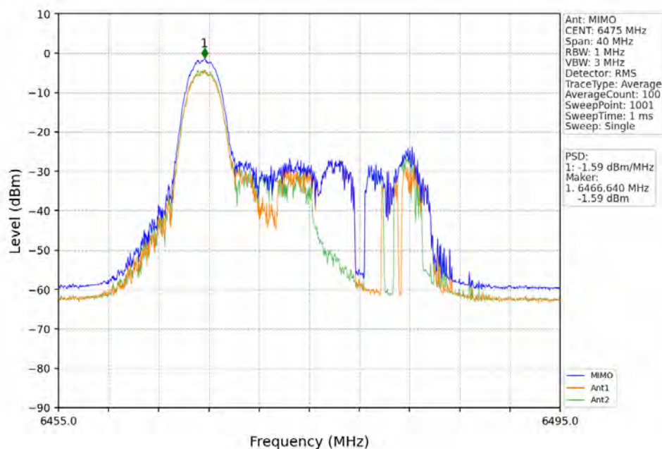
802.11ax(HEW20)_MCH_6475MHz_RU26_Left_MIMO_NTNV
