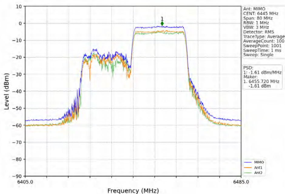
802.11ax(HEW40)_LCH_6445MHz_RU484_Left_MIMO_NTNV
