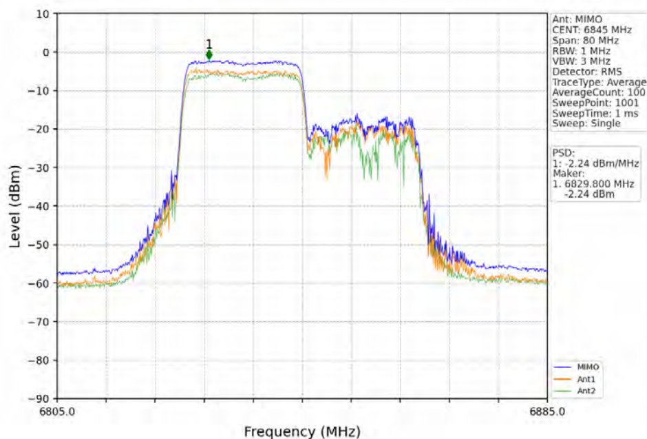
802.11ax(HEW40)_HCH_6845MHz_RU242_Left_MIMO_NTNV
