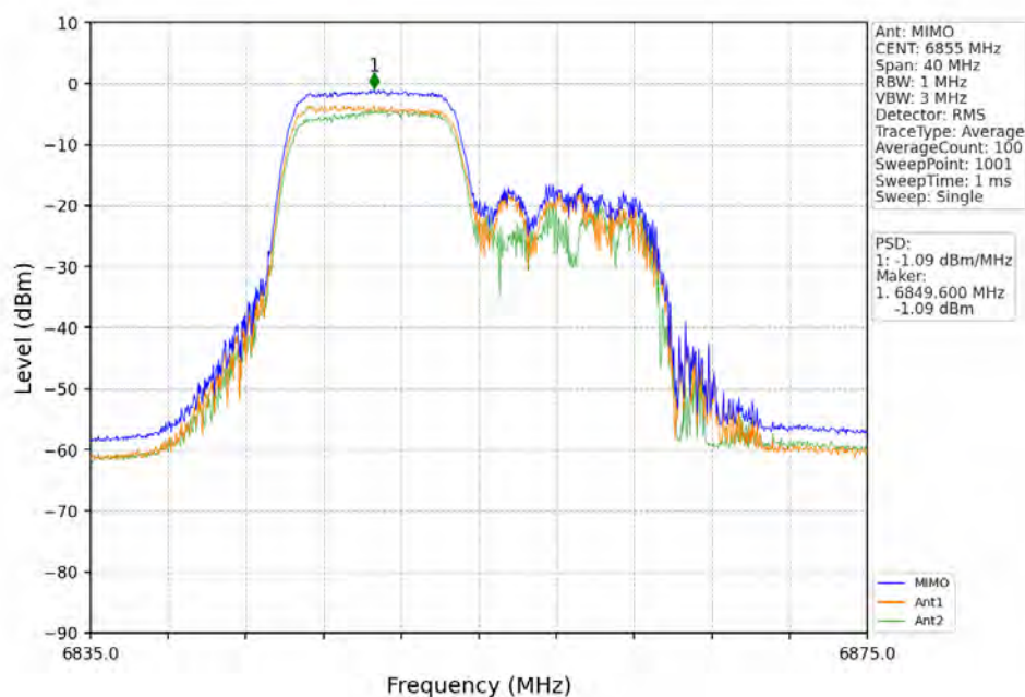
802.11ax(HEW20)_HCH_6855MHz_RU106_Right_MIMO_NTNV
