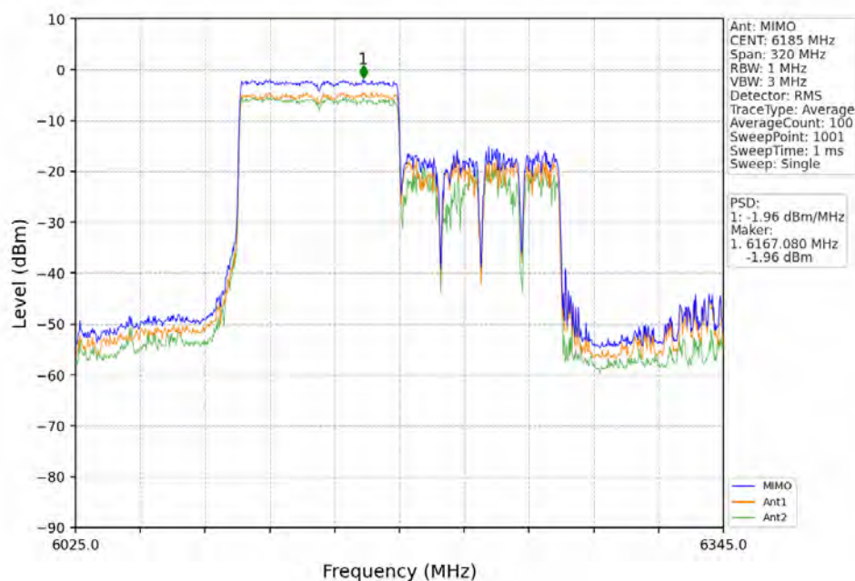
802.11ax(HEW160)_MCH_6185MHz_RU996_Right_MIMO_NTNV
