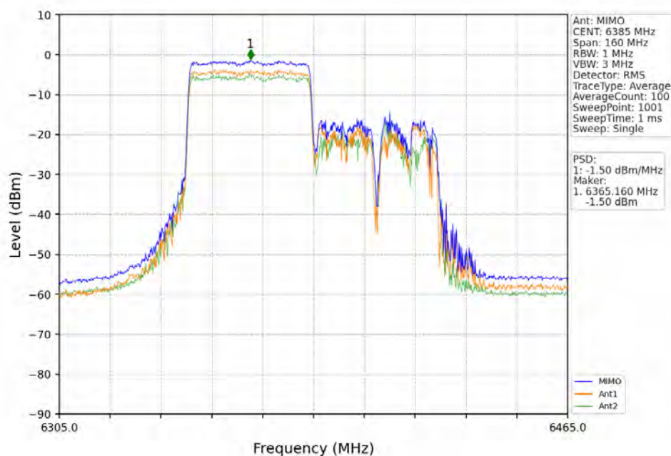
802.11ax(HEW80)_HCH_6385MHz_RU484_Right_MIMO_NTNV
