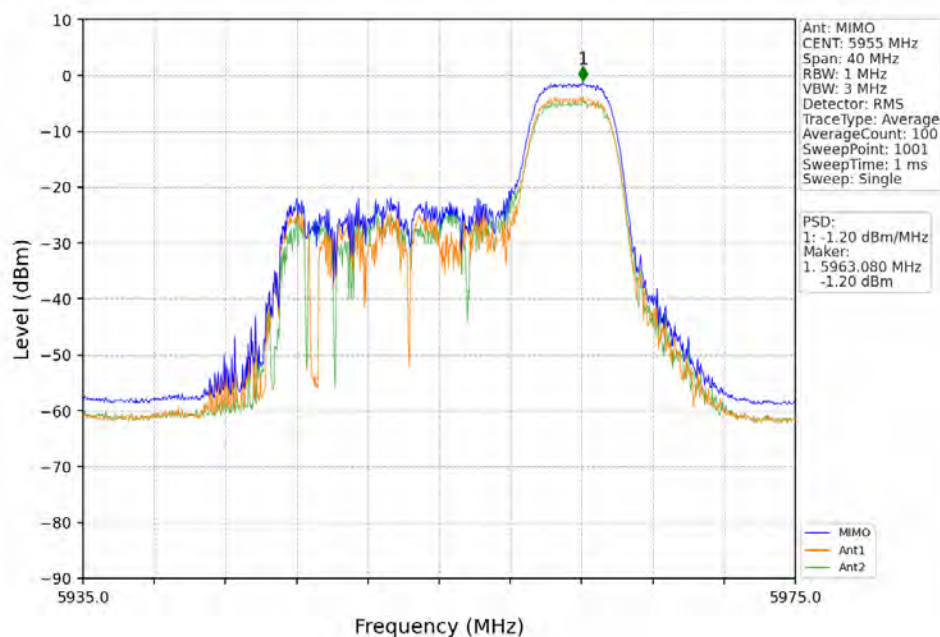
802.11ax(HEW20)_LCH_5955MHz_RU52_Right_MIMO_NTNV
