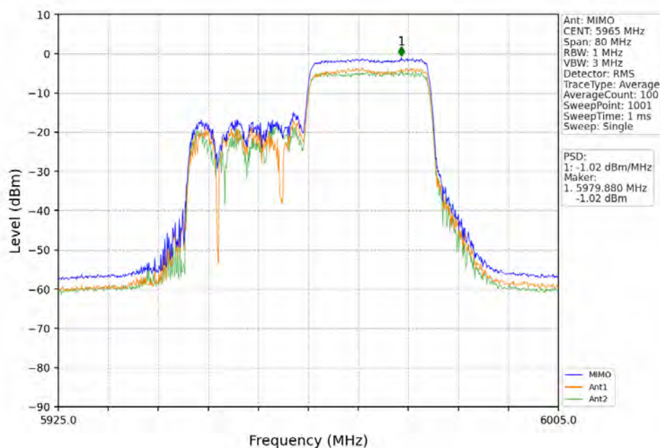
802.11ax(HEW40)_LCH_5965MHz_RU484_Left_MIMO_NTNV
