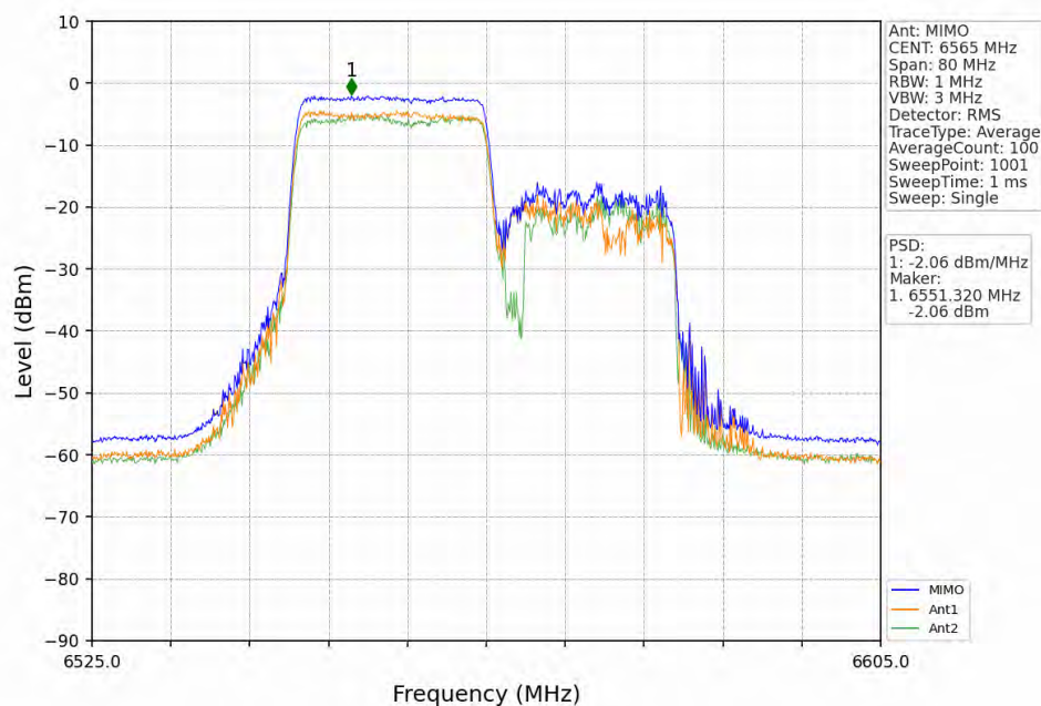
802.11ax(HEW40)_LCH_6565MHz_RU242_Left_MIMO_NTNV
