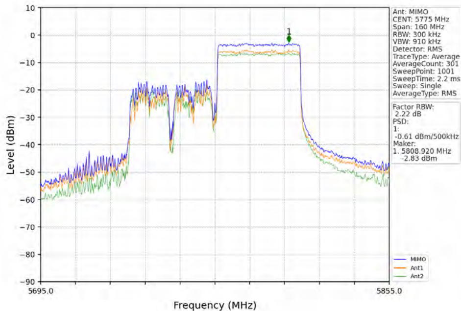
802.11ax(HEW80)_MCH_5775MHz_RU484_Right_MIMO_NTNV
