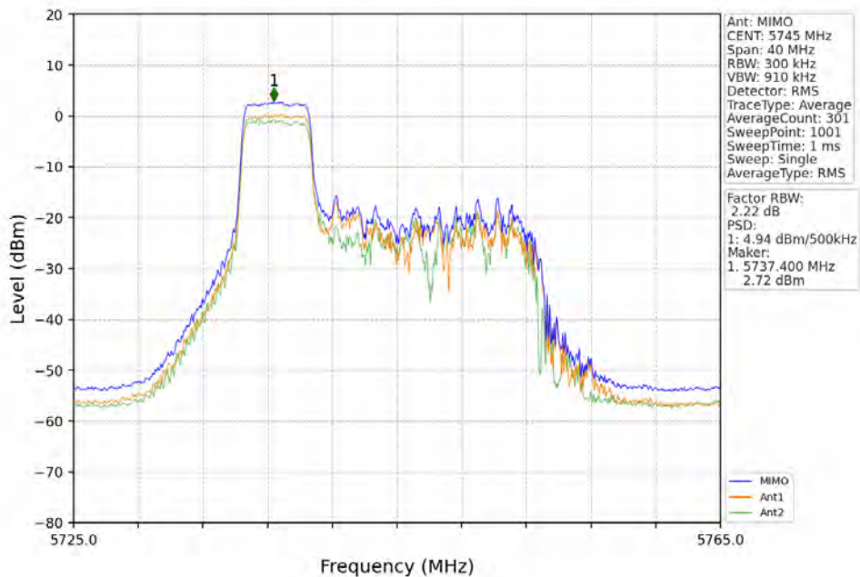
802.11ax(HEW20)_LCH_5745MHz_RU52_Left_MIMO_NTNV
