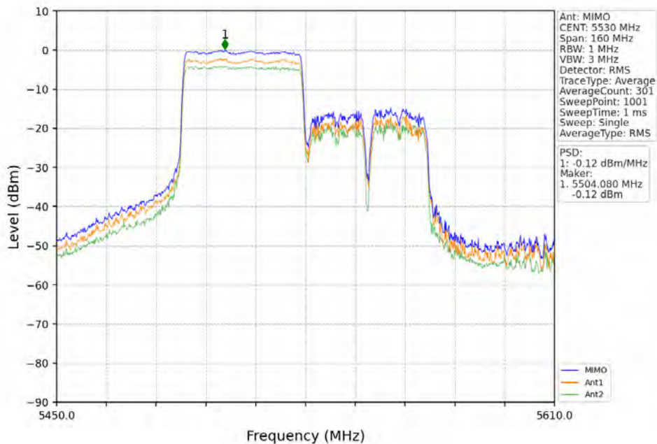
802.11ax(HEW80)_LCH_5530MHz_RU484_Left_MIMO_NTNV
