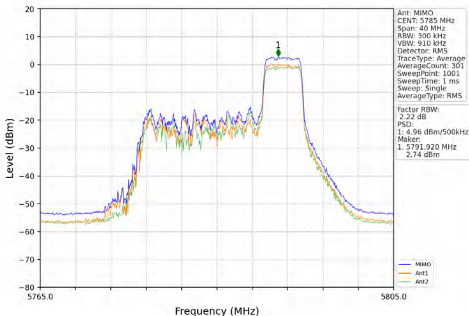
802.11ax(HEW20)_MCH_5785MHz_RU52_Right_MIMO_NTNV
