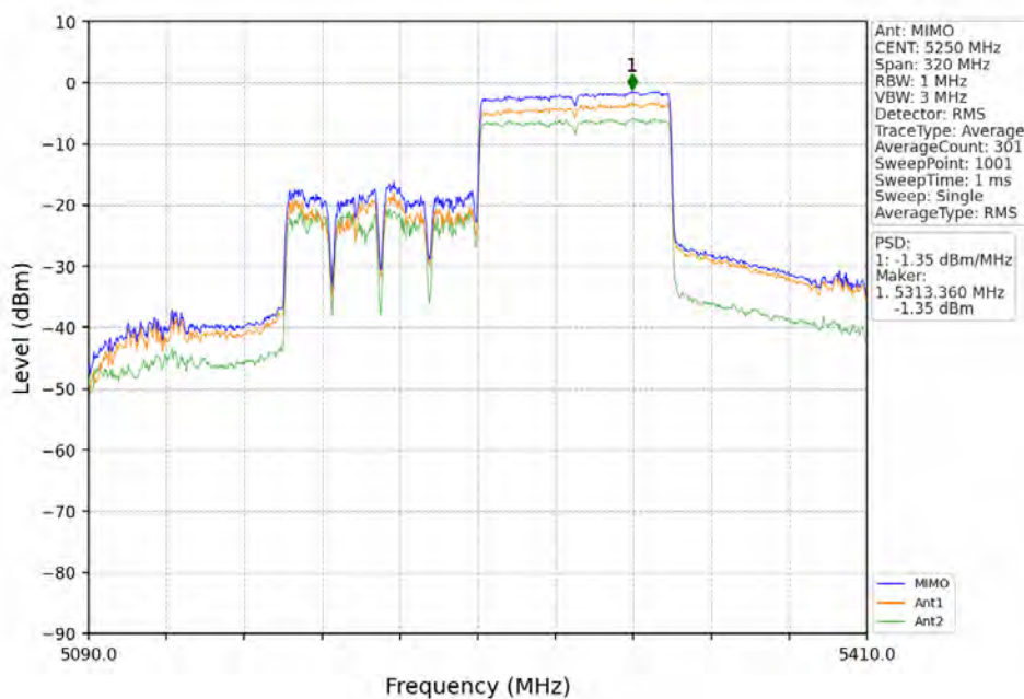
802.11ax(HEW160) MCH 5250MHz RU996 Right MIMO NTNV
