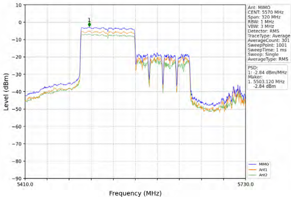
802.11ax(HEW160)_MCH_5570MHz_RU996_Left_MIMO_NTNV
