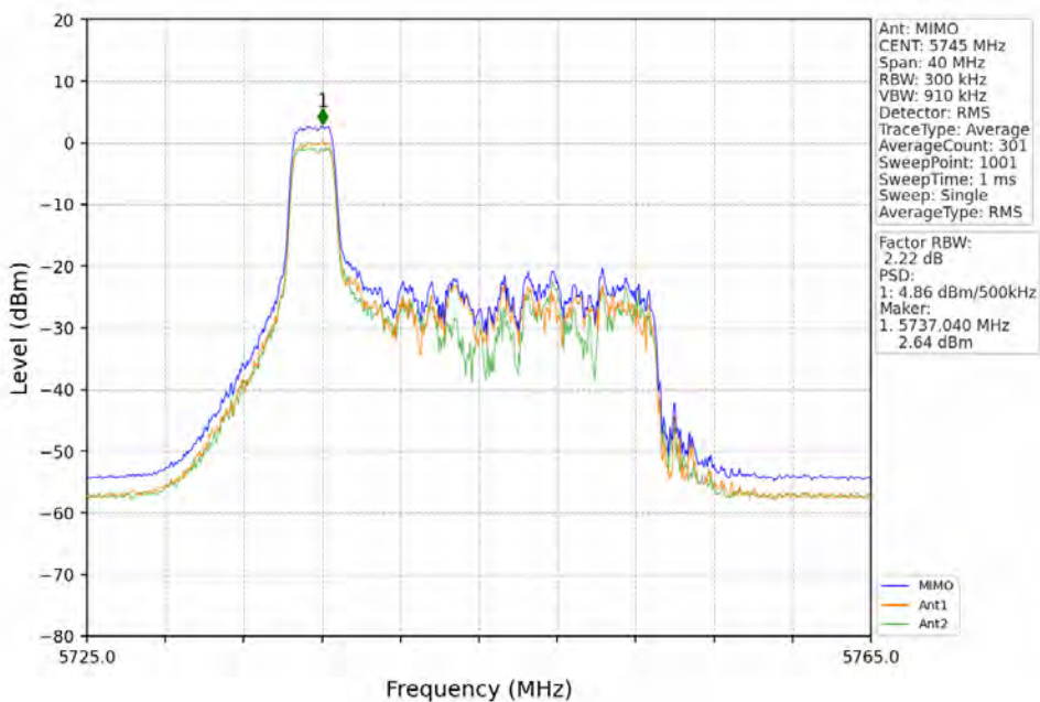
802.11ax(HEW20)_LCH_5745MHz_RU26_Left_MIMO_NTNV
