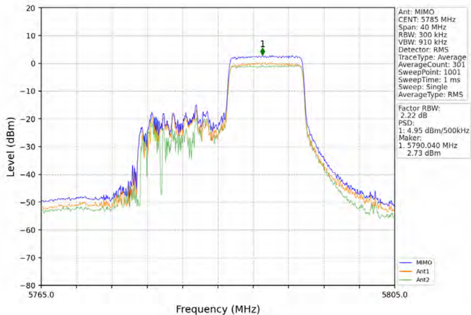
802.11ax(HEW20)_MCH_5785MHz_RU106_Right_MIMO_NTNV
