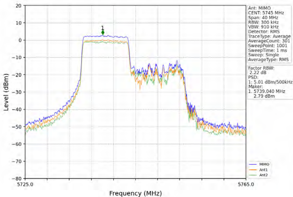
802.11ax(HEW20)_LCH_5745MHz_RU106_Left_MIMO_NTNV
