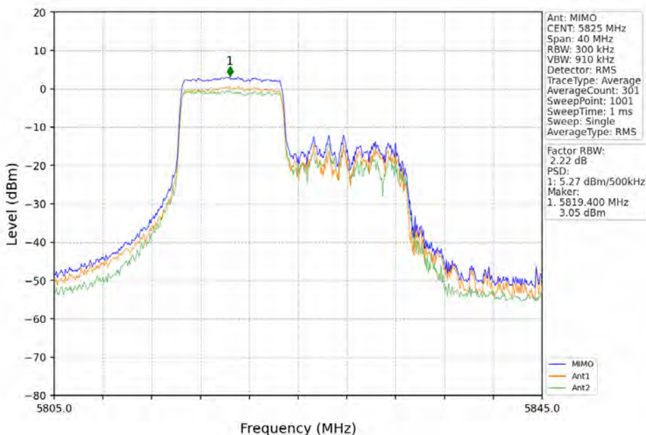
802.11ax(HEW20)_HCH_5825MHz_RU106_Left_MIMO_NTNV
