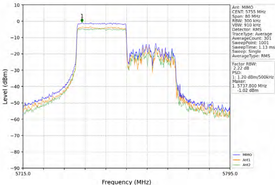
802.11ax(HEW40)_LCH_5755MHz_RU242_Right_MIMO_NTNV
