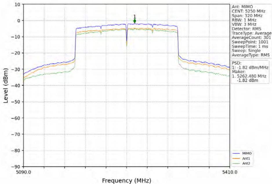
802.11ax(HEW160)_MCH_5250MHz_2xRU996_Left_MIMO_NTNV
