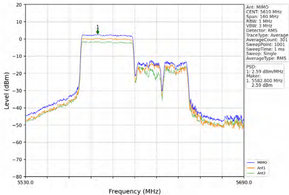
802.11ax(HEW80)_HCH_5610MHz_RU484_Right_MIMO_NTNV
