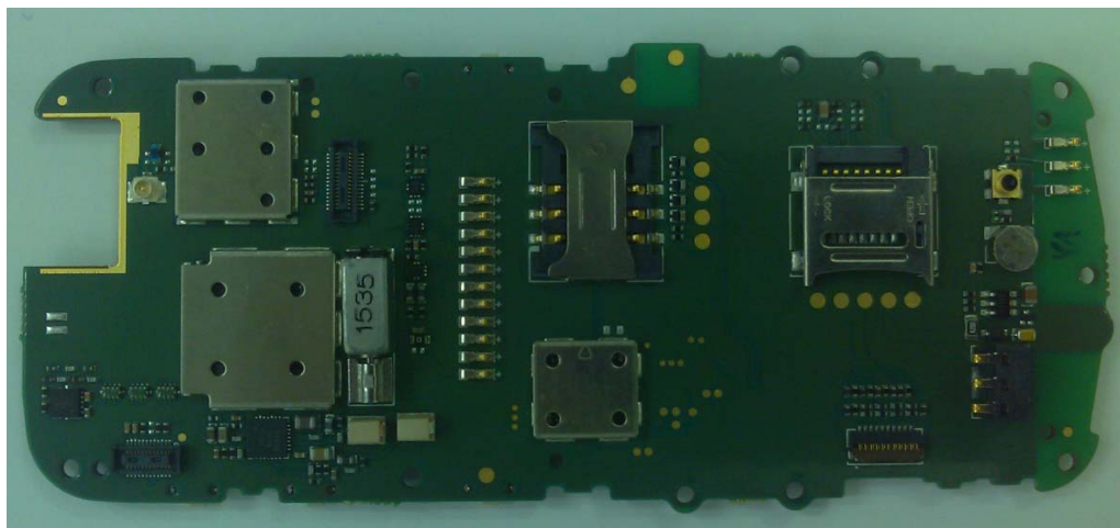
Picture 2: the top view of the PCB with the shielding cover removed
