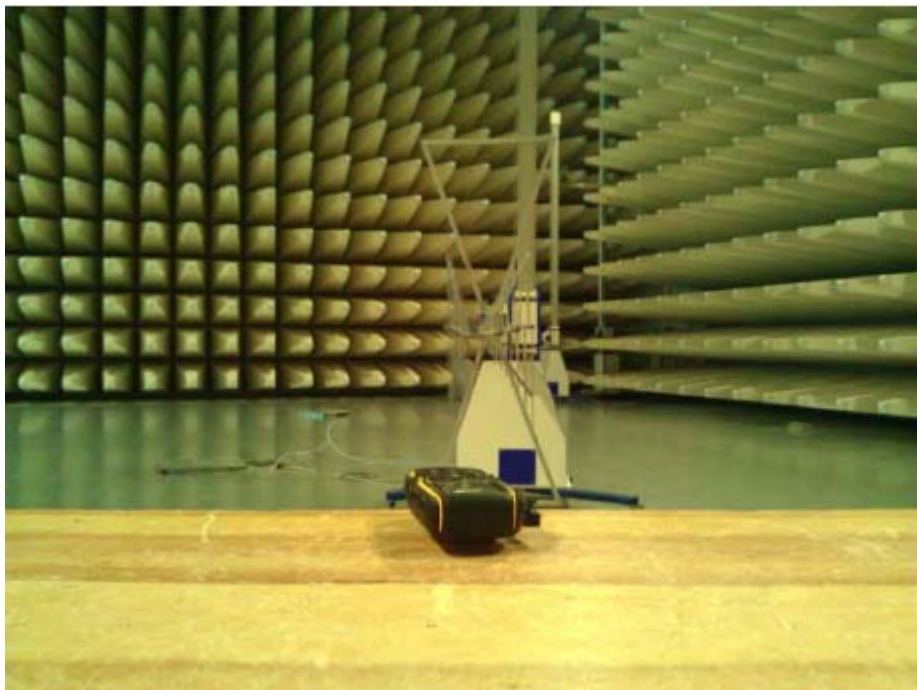
RF Receiver Spurious Emission Test Setup
