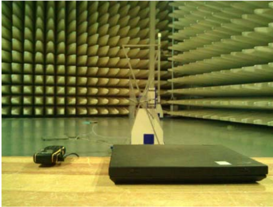
Part15B: Radiated Emissions Test Setup (below 1GHz)
