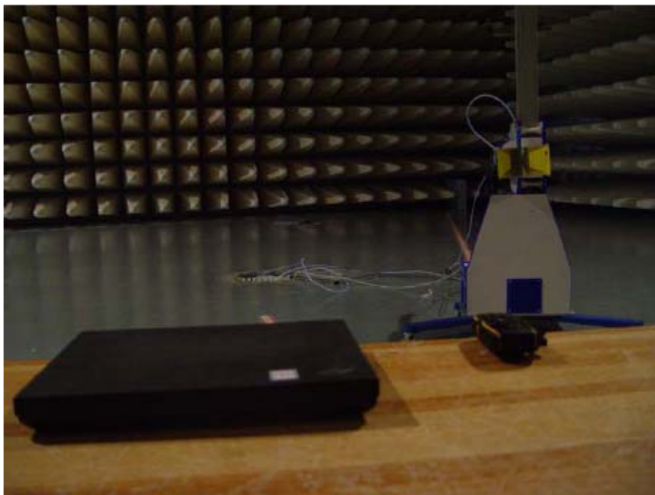
Part15B: Radiated Emissions Test Setup (above 1GHz)
