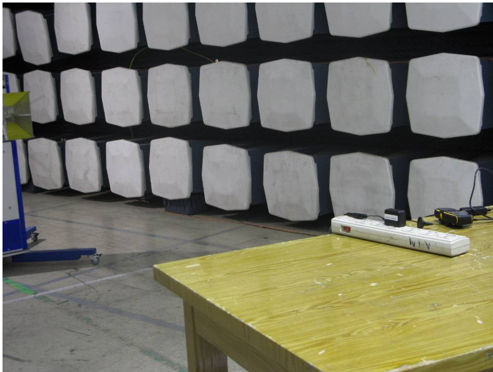
Part15C Radiated Emissions Test Setup
