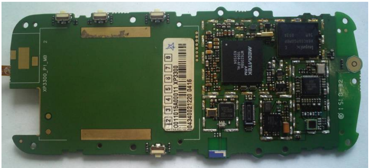
Picture 2: the top view of the PCB with the shielding cover removed
