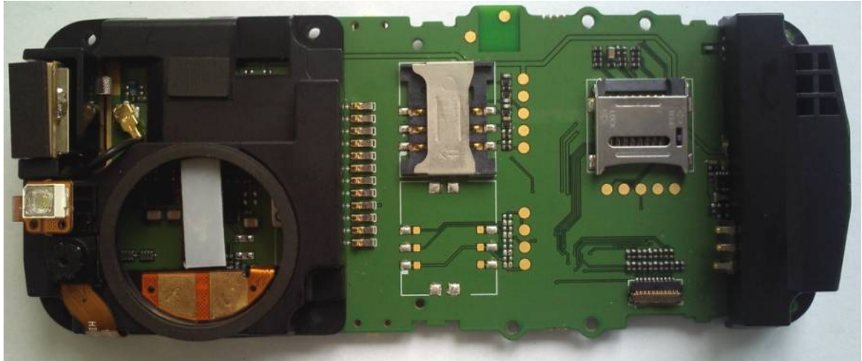
Picture 3: the back view of the PCB
