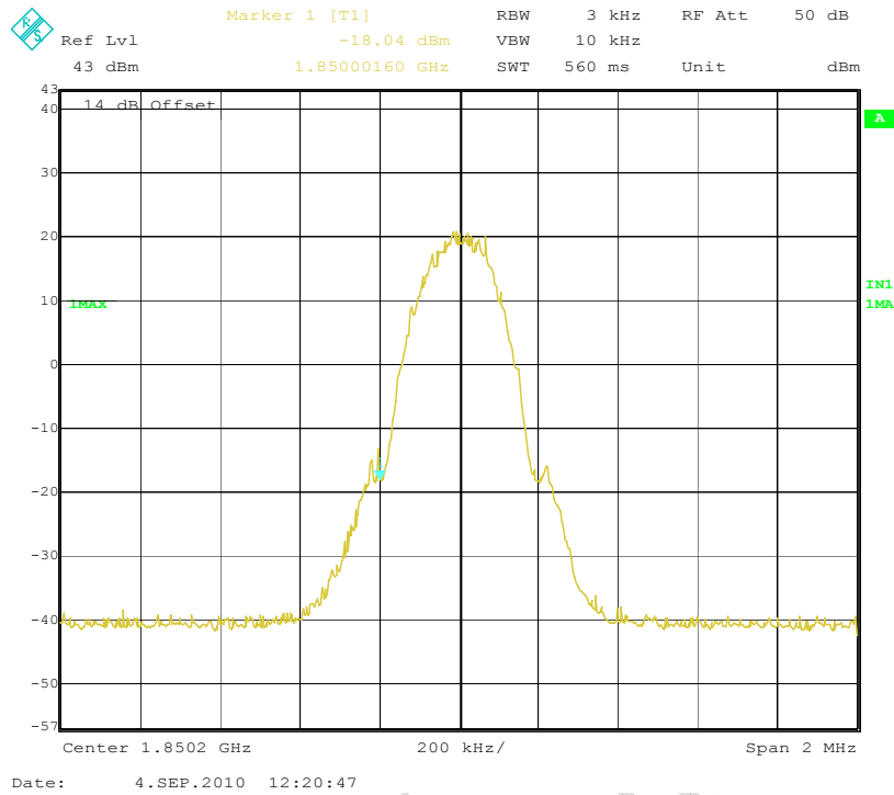
Channel 512 Left band edge (GSM)
