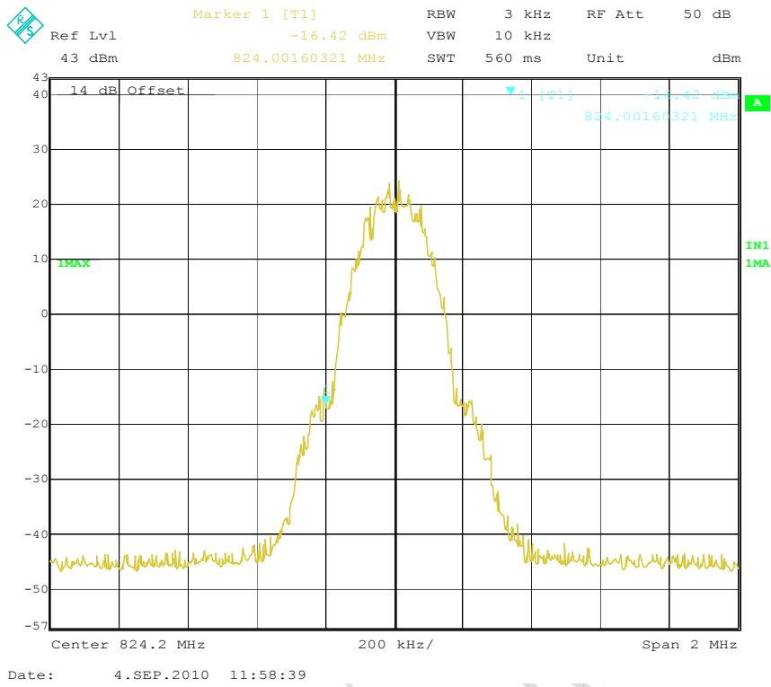
Channel 128 Left band edge (GPRS)
