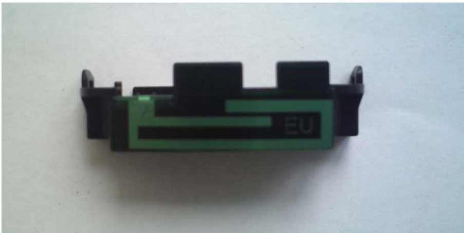
Picture 5: The antenna
