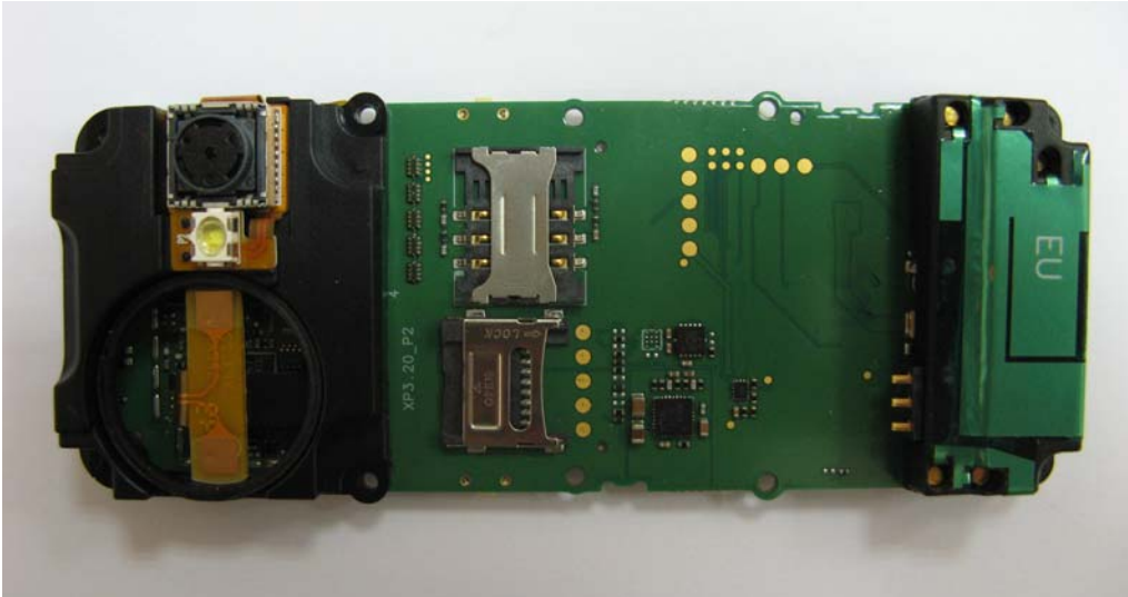
Picture 3: the back view of the PCB
