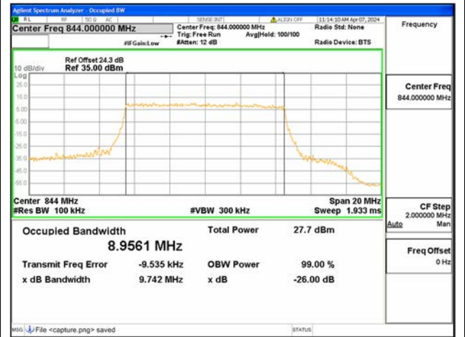
B26 Part22 / 10MHz / 64QAM/ High CH
