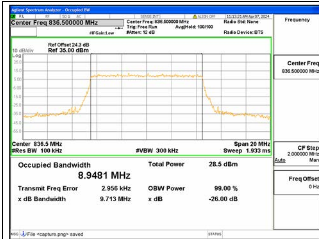
B26 Part22 / 10MHz / QPSK/ Mid CH
