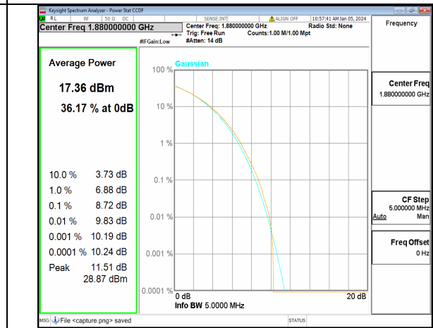
n2 5M CP-OFDM 256QAM Outer_Full Mid
