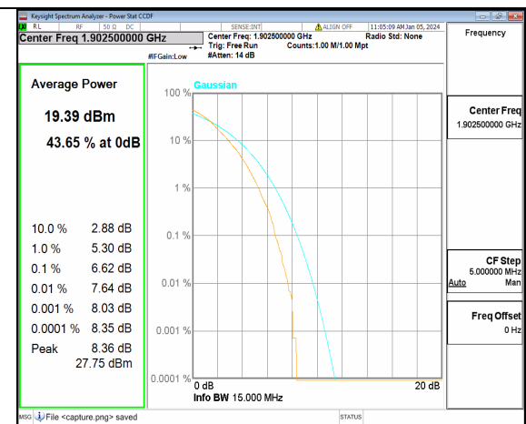
n2 15M DFT-s-OFDM 256QAM Outer_Full High
