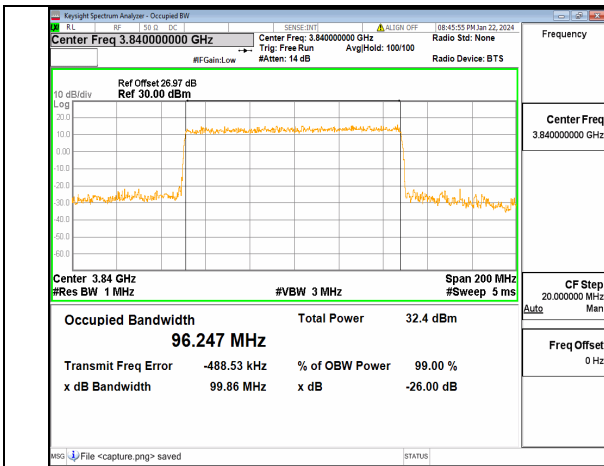
n77(3700-3980MHz) 100M DFT-s-OFDM 16QAM Outer_Full Mid
