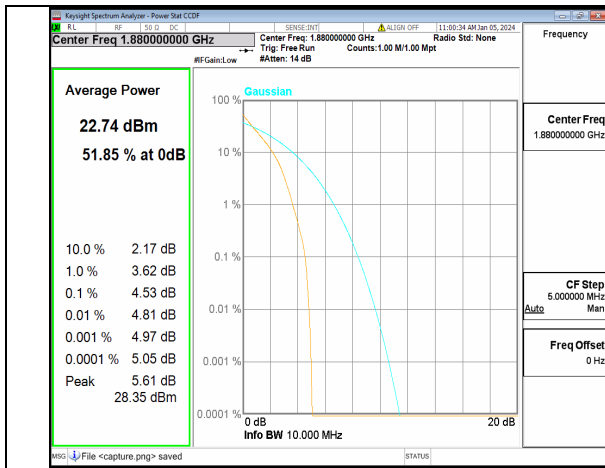
n2 10M DFT-s-OFDM BPSK Outer_Full Mid
