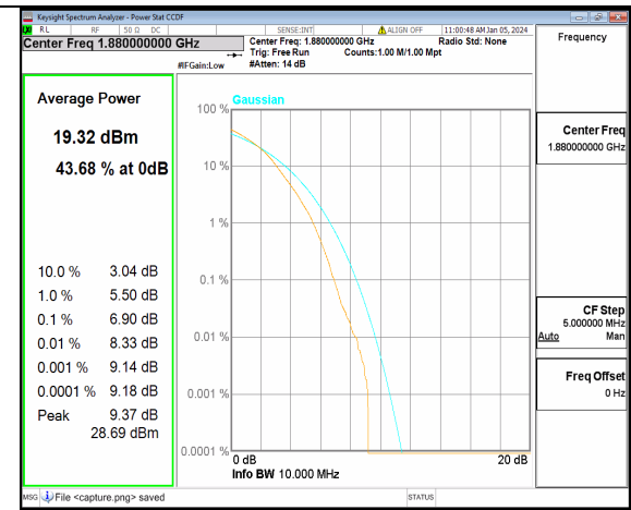
n2 10M DFT-s-OFDM 256QAM Outer_Full Mid
