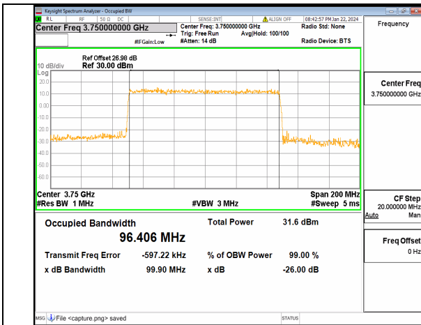
n77(3700-3980MHz) 100M DFT-s-OFDM 16QAM Outer_Full Low
