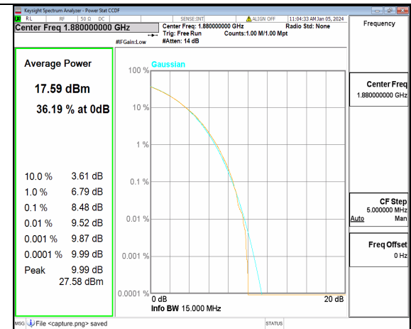
n2 15M CP-OFDM 256QAM Outer_Full Mid
