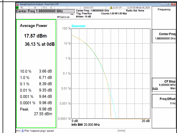
n2 20M CP-OFDM 256QAM Outer_Full Mid
