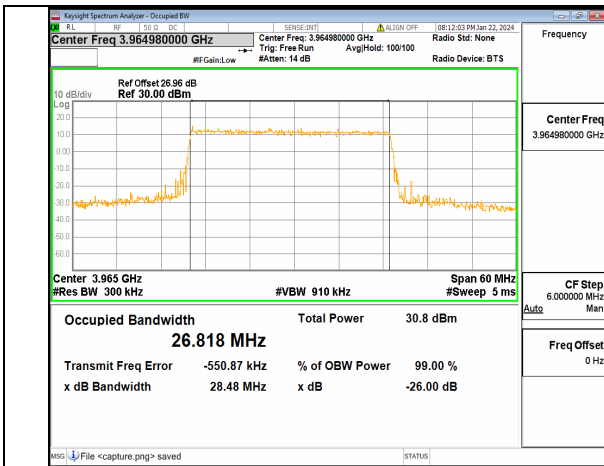
n77(3700-3980MHz) 30M DFT-s-OFDM 16QAM Outer_Full High
