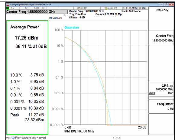
n2 10M CP-OFDM 256QAM Outer_Full Mid
