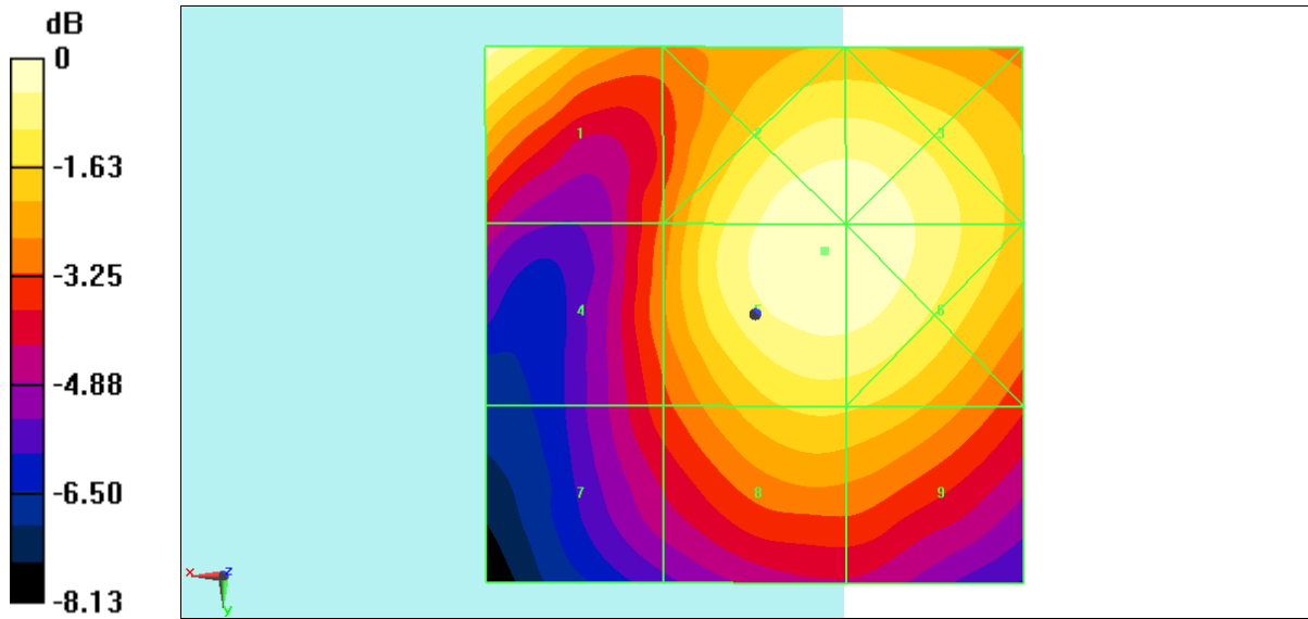
Fig B.3 HAC RF E-Field LTE Band48 QPSK
