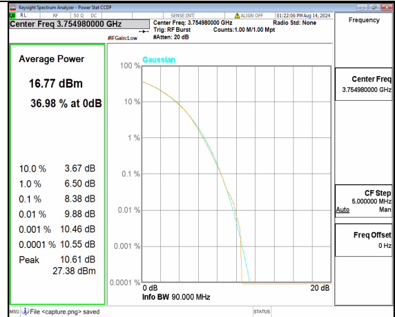
n78(3700-3800MHz) 90M CP-OFDM 256QAM Outer_Full High
