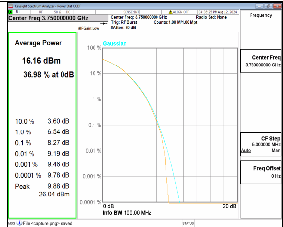
n77(3700-3980MHz) 100M CP-OFDM 256QAM Outer_Full Low
