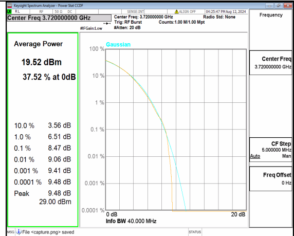
n77(3700-3980MHz) 40M CP-OFDM 256QAM Outer_Full Low
