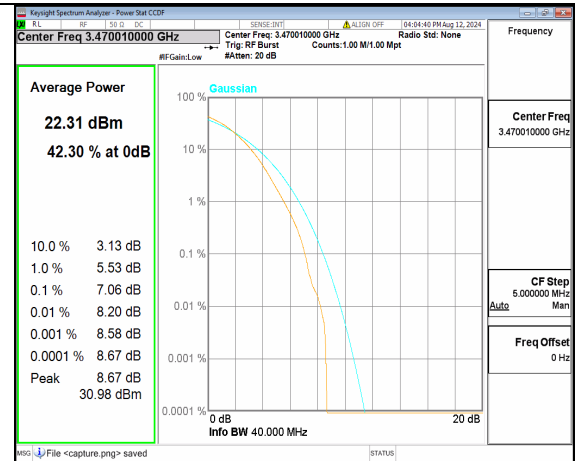
n77(3450-3550MHz) 40M DFT-s-OFDM 256QAM Outer_Full Low
