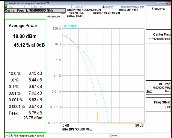
n66 30M DFT-s-OFDM 256QAM Outer_Full High
