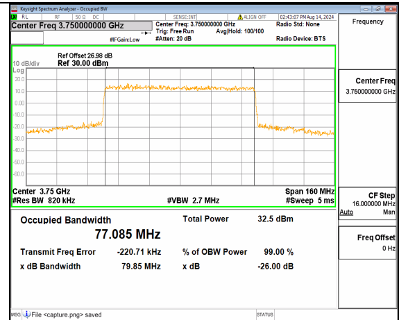
n78(3700-3800MHz) 80M DFT-s-OFDM QPSK Outer_Full Mid
