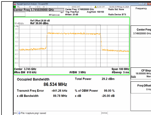
n78(3700-3800MHz) 90M DFT-s-OFDM 256QAM Outer_Full Low
