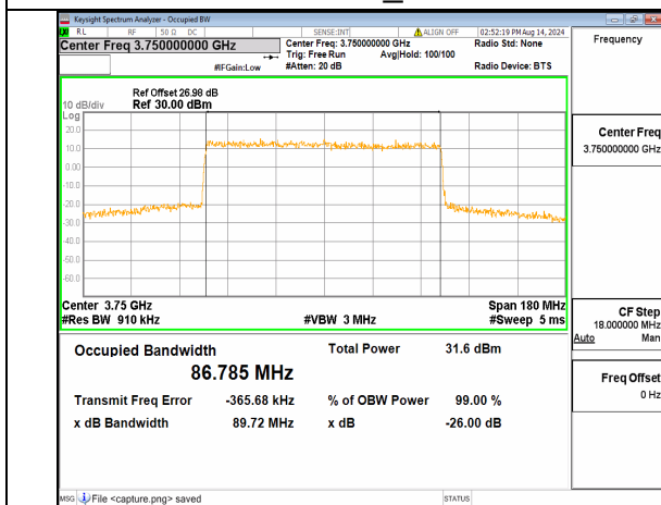
n78(3700-3800MHz) 90M DFT-s-OFDM 16QAM Outer_Full Mid
