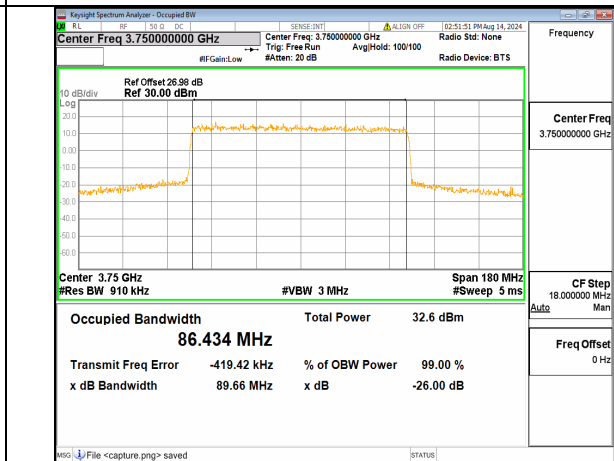
n78(3700-3800MHz) 90M DFT-s-OFDM QPSK Outer_Full Mid
