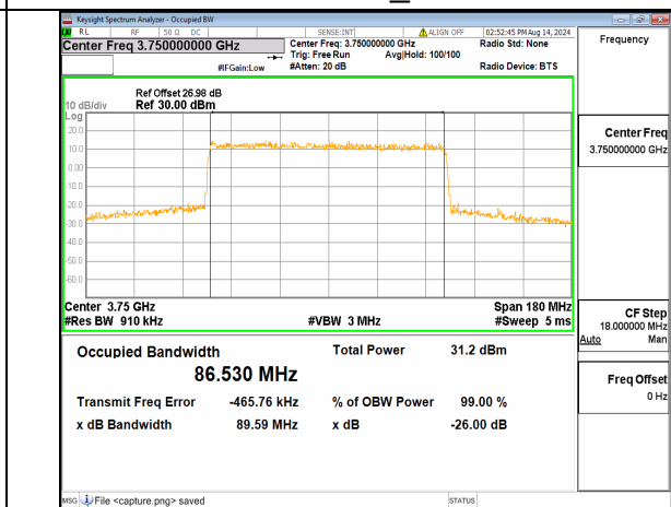
n78(3700-3800MHz) 90M DFT-s-OFDM 64QAM Outer_Full Mid
