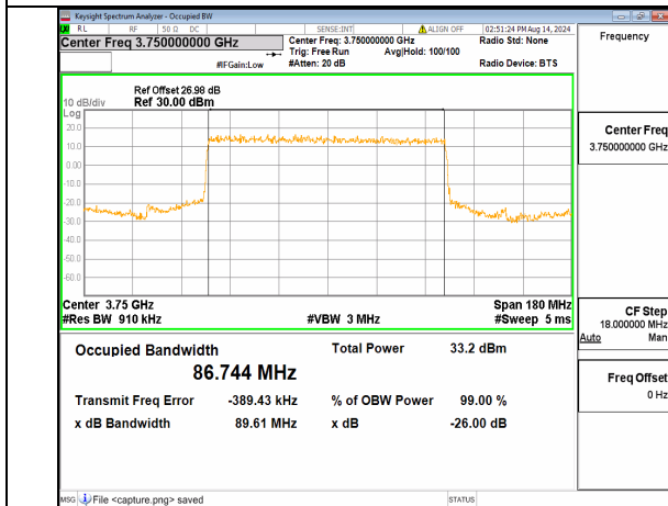
n78(3700-3800MHz) 90M DFT-s-OFDM BPSK Outer_Full Mid
