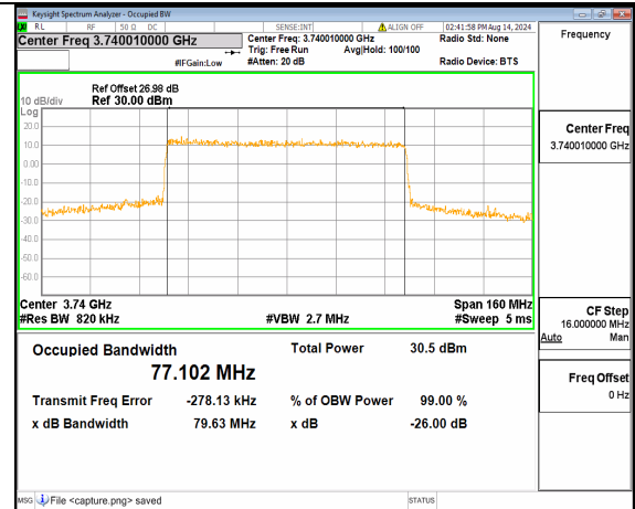
n78(3700-3800MHz) 80M CP-OFDM QPSK Outer_Full Low
