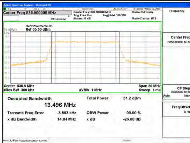
B26 Part22 / 15MHz / QPSK/ Mid CH
