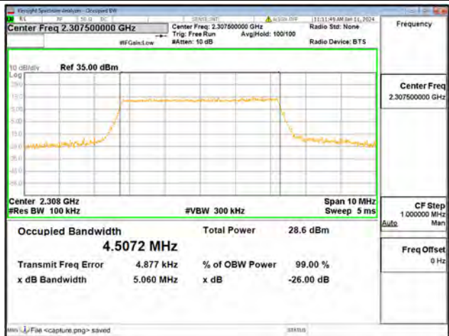
B30 / 5MHz / 64QAM/ Low CH
