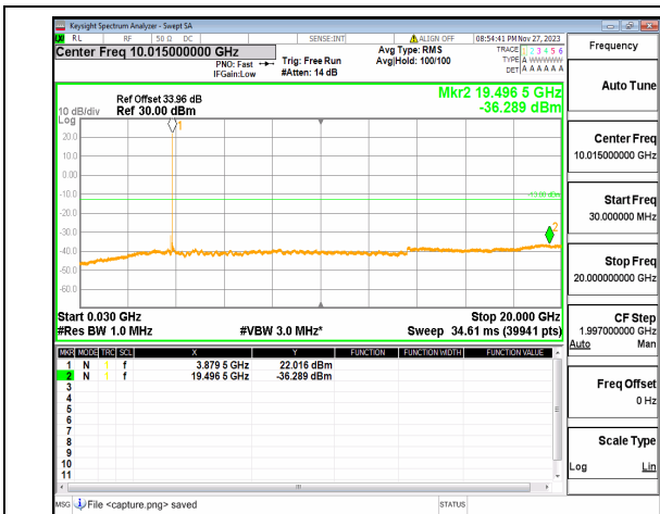
n77(3700-3980MHz) (30MHz-20GHz) 80M DFT-s-OFDM QPSK Edge_1RB_Right Mid
