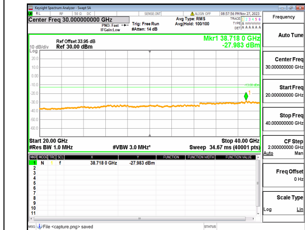
n77(3700-3980MHz) (20GHz-40GHz) 80M DFT-s-OFDM BPSK Edge_1RB_Right High
