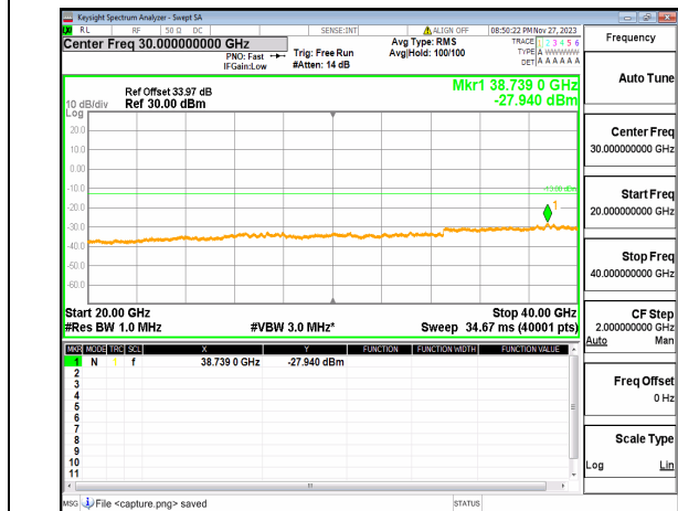
n77(3700-3980MHz) (20GHz-40GHz) 80M DFT-s-OFDM QPSK Edge_1RB_Right Low
