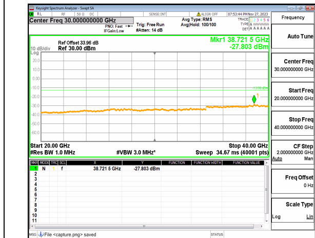
n77(3700-3980MHz) (20GHz-40GHz) 20M DFT-s-OFDM QPSK Edge 1RB Left Mid
