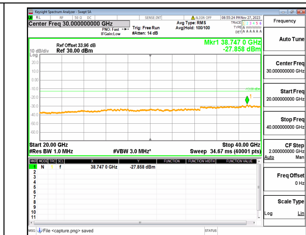
n77(3700-3980MHz) (20GHz-40GHz) 80M DFT-s-OFDM QPSK Edge_1RB_Right Mid
