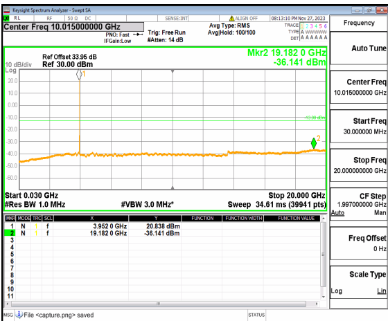
n77(3700-3980MHz) (30MHz-20GHz) 30M DFT-s-OFDM QPSK Edge_1RB Left High
