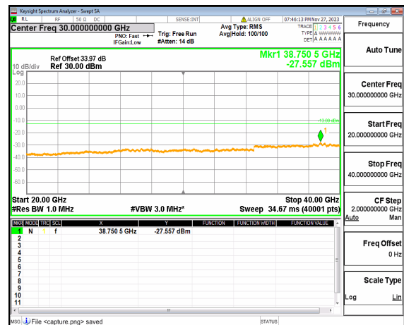
n77(3700-3980MHz) (20GHz-40GHz) 20M DFT-s-OFDM BPSK Edge 1RB Left Low
