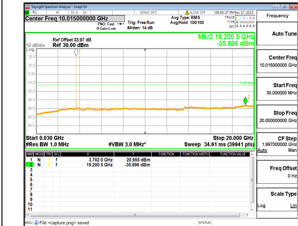
n77(3700-3980MHz) (30MHz-20GHz) 30M DFT-s-OFDM BPSK Edge_1RB Left Low
