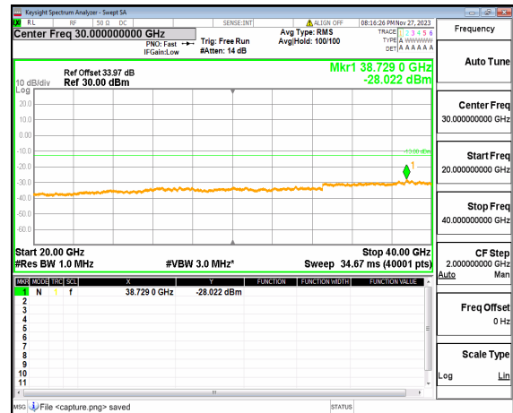
n77(3700-3980MHz) (20GHz-40GHz) 40M DFT-s-OFDM BPSK Edge_1RB Left Low
