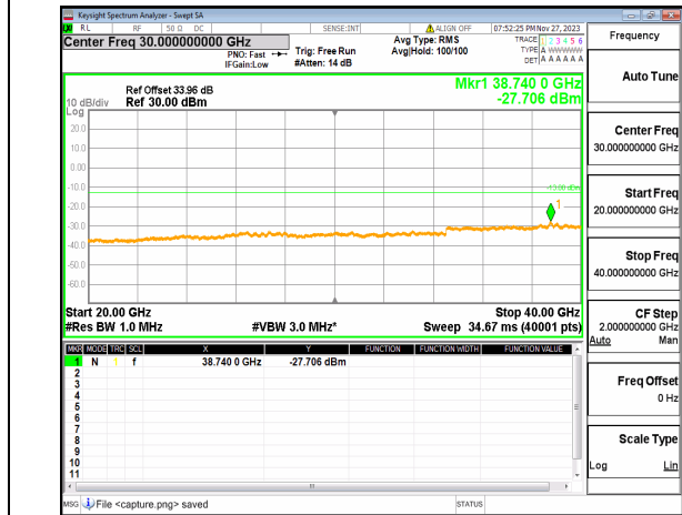
n77(3700-3980MHz) (20GHz-40GHz) 20M DFT-s-OFDM BPSK Edge 1RB Right Mid
