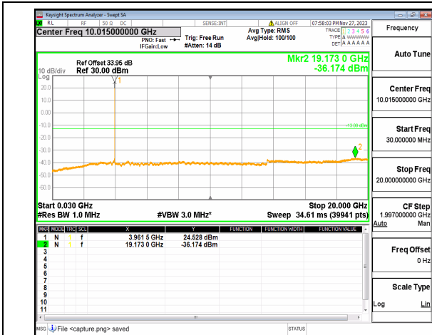
n77(3700-3980MHz) (30MHz-20GHz) 20M DFT-s-OFDM QPSK Edge_1RB Left High
