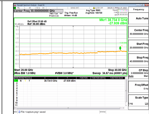
n77(3700-3980MHz) (20GHz-40GHz) 40M DFT-s-OFDM QPSK Edge_1RB_Right Mid
