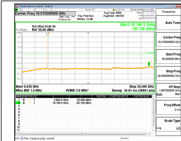
n77(3700-3980MHz) (30MHz-20GHz) 30M DFT-s-OFDM QPSK Edge_1RB_Right Mid
