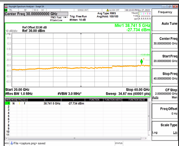
n77(3700-3980MHz) (20GHz-40GHz) 30M DFT-s-OFDM QPSK Edge_1RB_Right Mid
