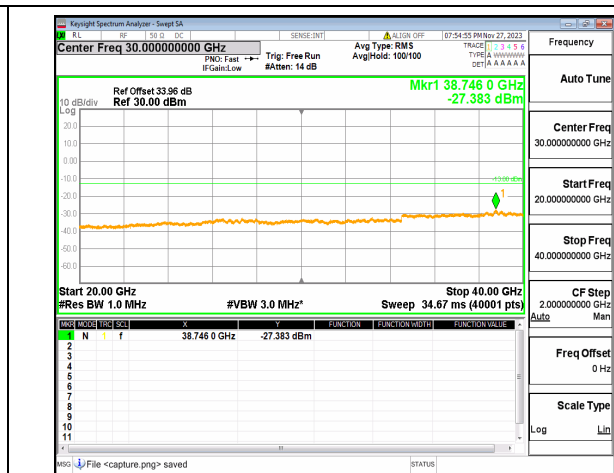
n77(3700-3980MHz) (20GHz-40GHz) 20M DFT-s-OFDM QPSK Edge_1RB_Right Mid
