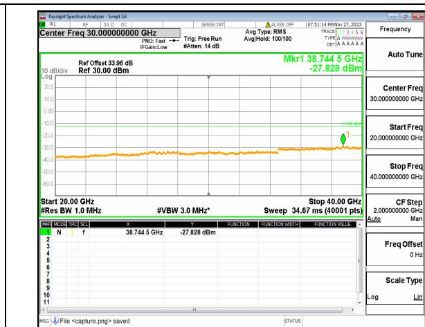
n77(3700-3980MHz) (20GHz-40GHz) 20M DFT-s-OFDM BPSK Edge 1RB Left Mid
