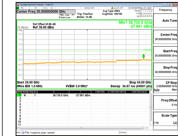
n77(3700-3980MHz) (20GHz-40GHz) 20M DFT-s-OFDM QPSK Edge_1RB Right High
