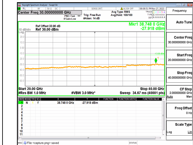
n77(3700-3980MHz) (20GHz-40GHz) 30M DFT-s-OFDM QPSK Edge_1RB_Left Mid
