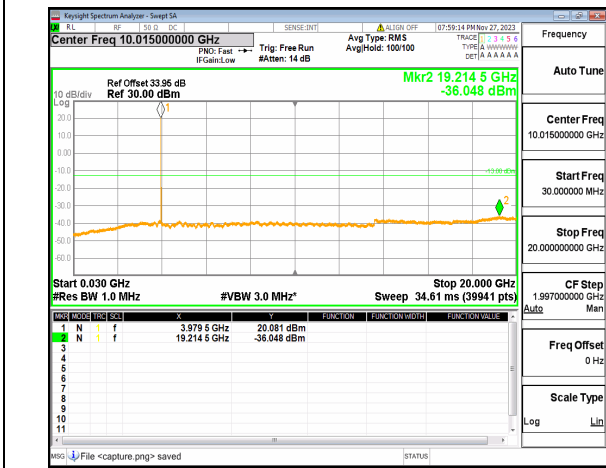
n77(3700-3980MHz) (30MHz-20GHz) 20M DFT-s-OFDM QPSK Edge_1RB Right High
