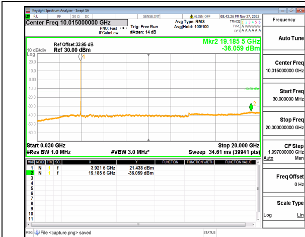
n77(3700-3980MHz) (30MHz-20GHz) 60M DFT-s-OFDM QPSK Edge_1RB Left High
