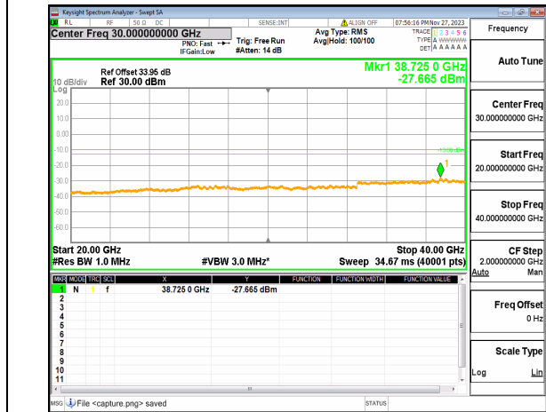
n77(3700-3980MHz) (20GHz-40GHz) 20M DFT-s-OFDM BPSK Edge_1RB_Left High
