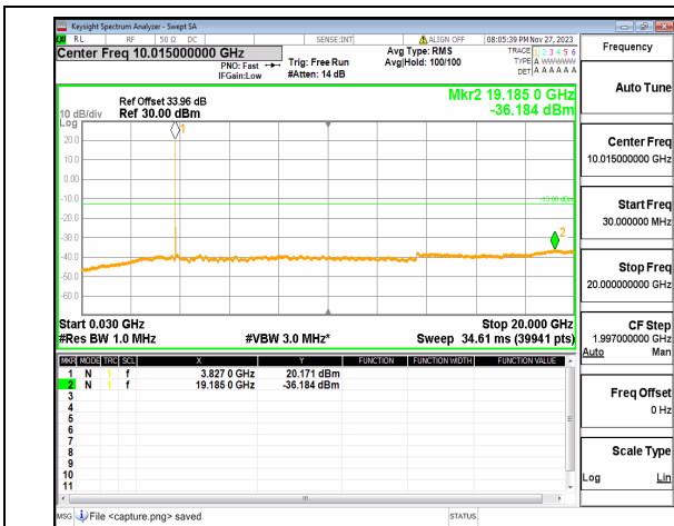
n77(3700-3980MHz) (30MHz-20GHz) 30M DFT-s-OFDM BPSK Edge_1RB_Left Mid
